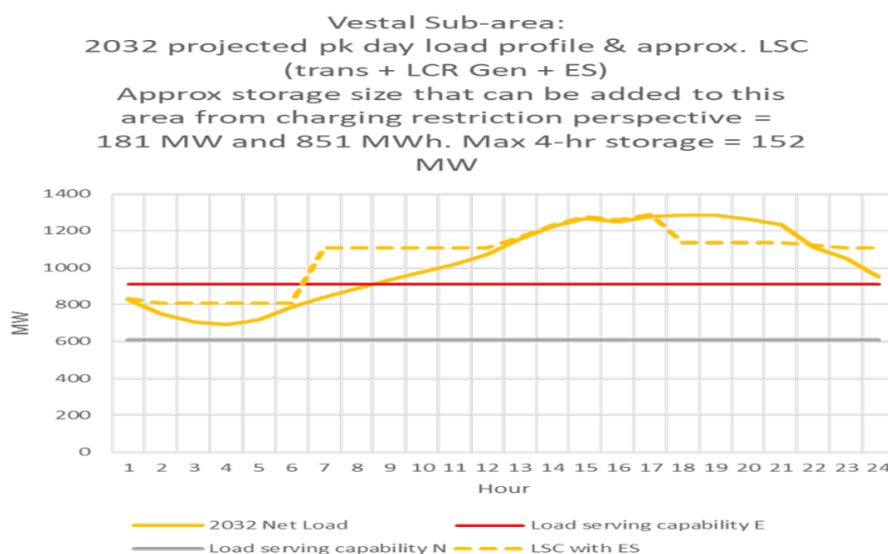
Figure J.3.2-66 Vestal LCR Sub-area 2032 Peak Day Forecast Profiles
