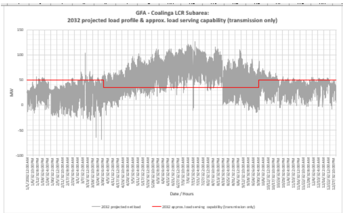
Figure J.3.2-41 Coalinga LCR Sub-area 2032 Forecast Hourly Profiles
