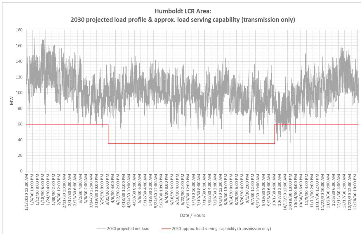
Figure 3.6-3 Humboldt 2030 Forecast Hourly Profile
