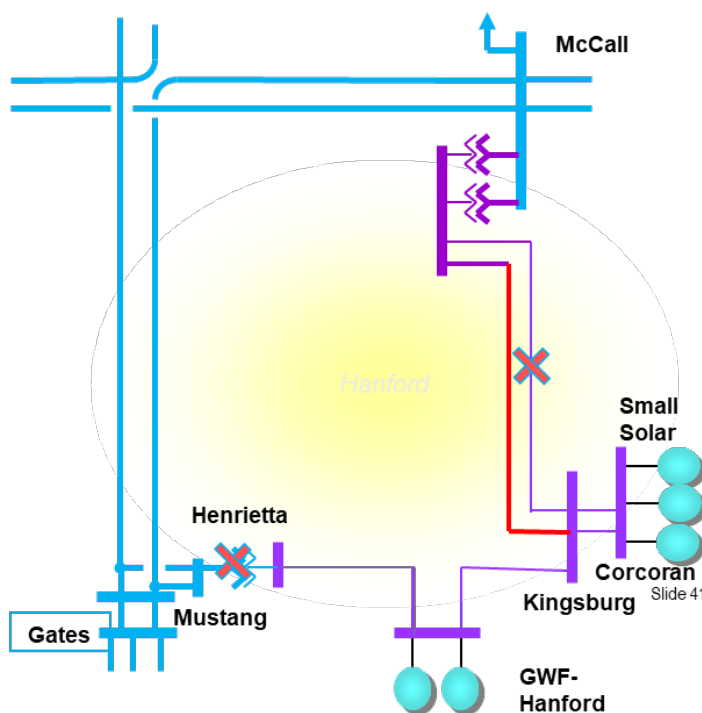
Figure 3.6-35 Hanford LCR Sub-area
