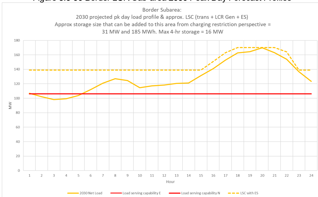
Figure 3.6-90 Border LCR Sub-area 2030 Peak Day Forecast Profiles
