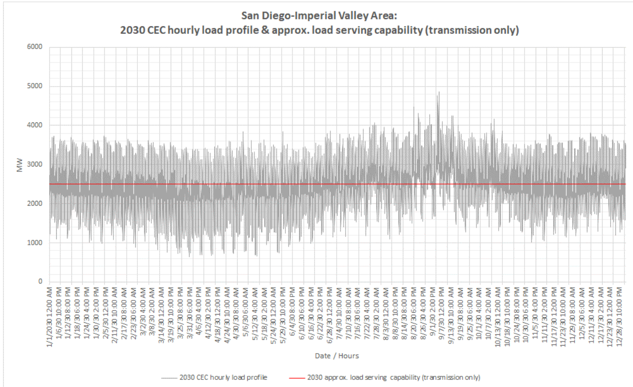
Figure 3.6-95 San Diego-Imperial Valley Area 2030 Hourly Load Forecast Profiles with Transmission Only Load Serving Capability
