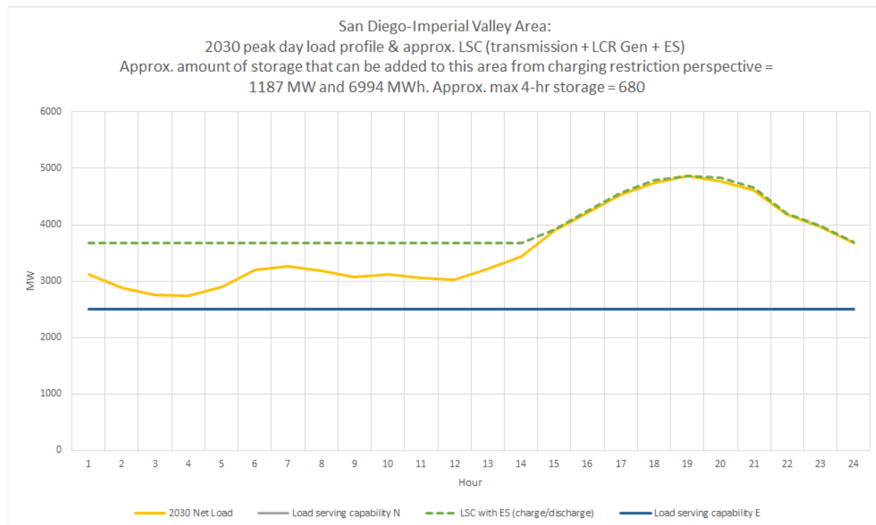
Figure 3.6-96 San Diego-Imperial Valley LCR Area 2030 Estimated Amount of Storage that Can Be Added Based on Charging Restriction
