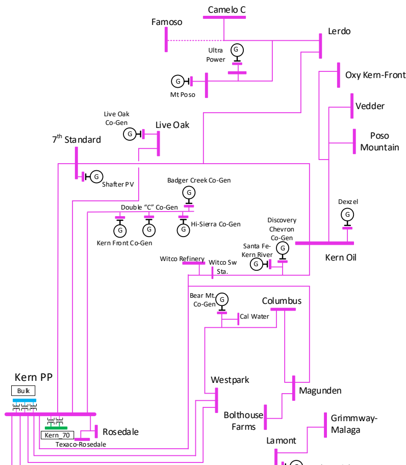
Figure 3.6-56 Kern Oil LCR Sub-area
