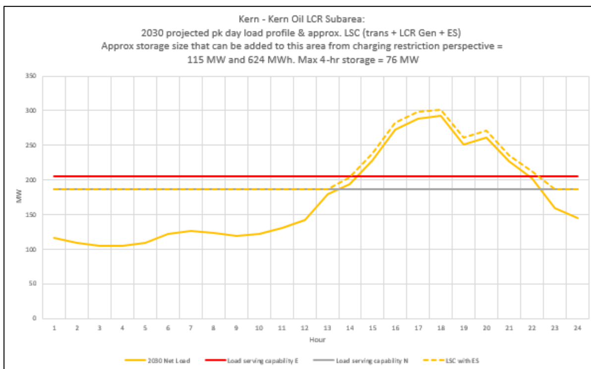
Figure 3.6-58 Kern Oil LCR Sub-area 2030 Forecast Hourly Profiles
