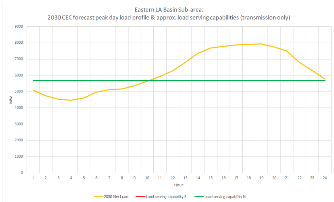
Figure 3.6-82 Eastern LA Basin LCR Sub-area 2030 Hourly Load Forecast Profiles with Transmission Only Load Serving Capability
