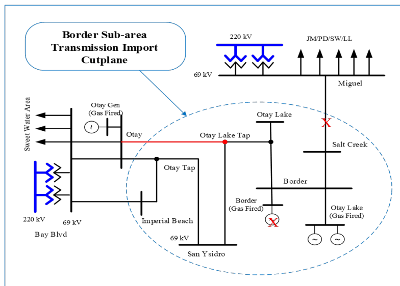
Figure 3.6-88 Border LCR Sub-area
