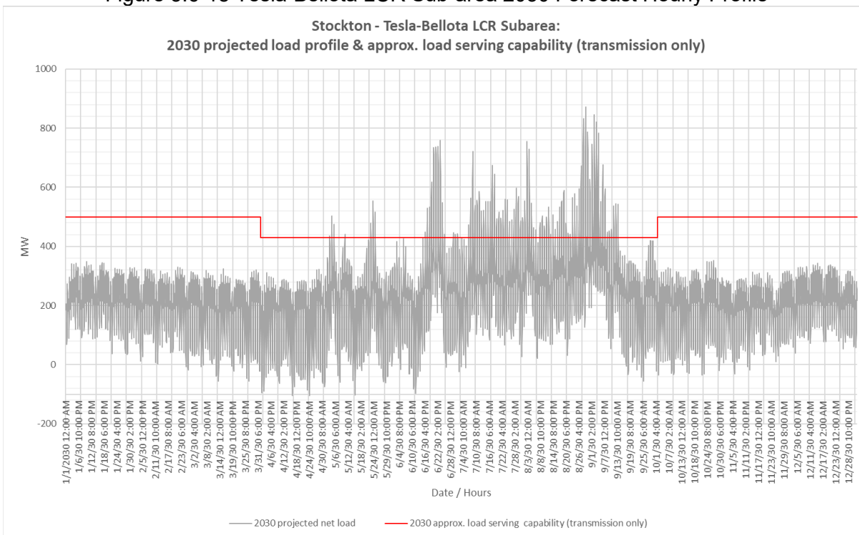
Figure 3.6-18 Tesla-Bellota LCR Sub-area 2030 Forecast Hourly Profile
