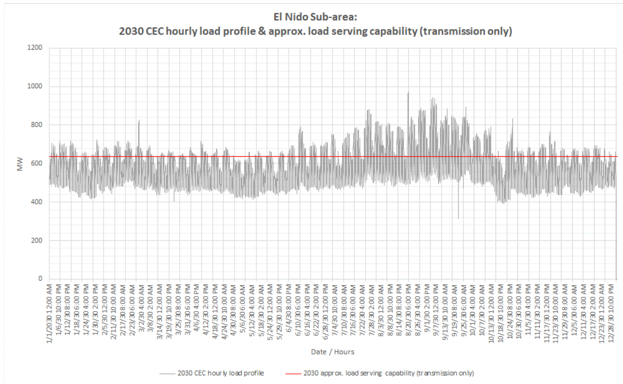
Figure 3.6-77 El Nido LCR Sub-area 2030 Estimated Amount of Storage that Can Be Added Based on Charging Restriction
