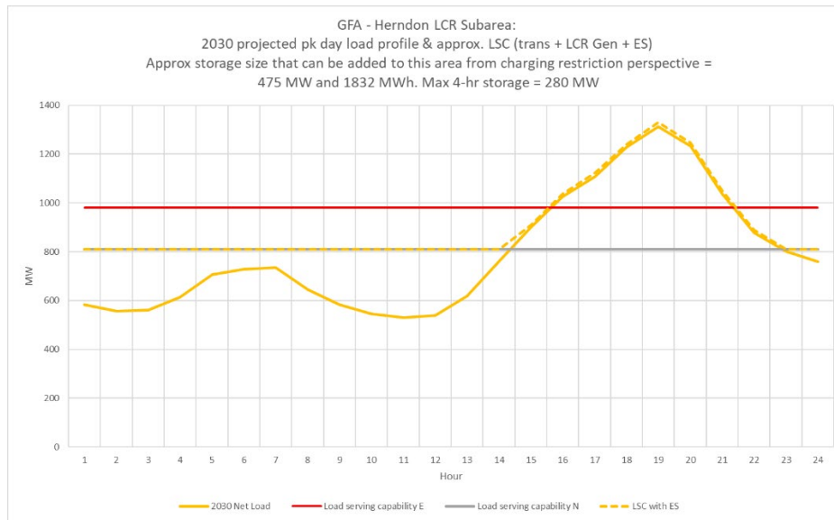
Figure 3.6-49 Herndon LCR Sub-area 2030 Forecast Hourly Profiles
