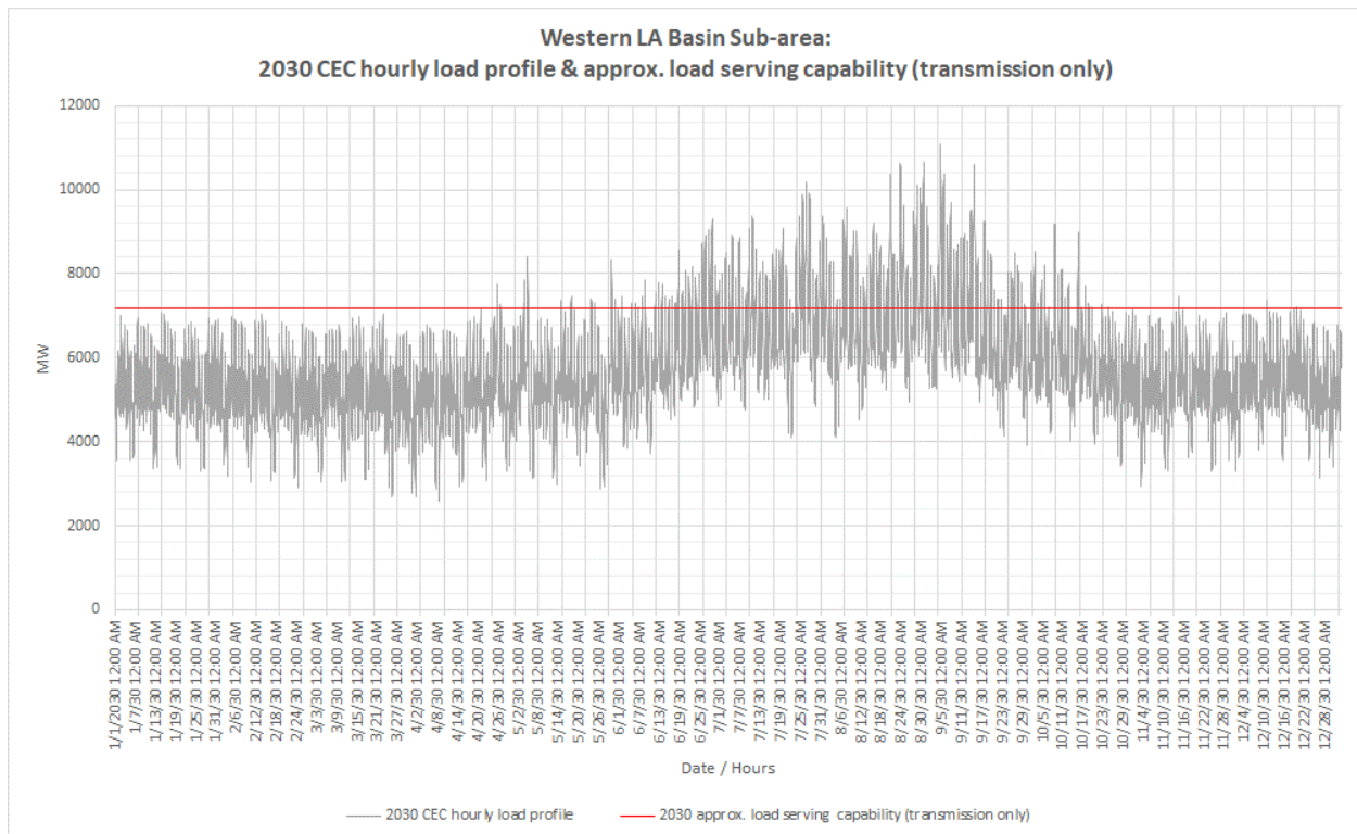
Figure 3.6-79 Western LA Basin LCR Sub-area 2030 Hourly Load Forecast Profiles with Transmission Only Load Serving Capability
