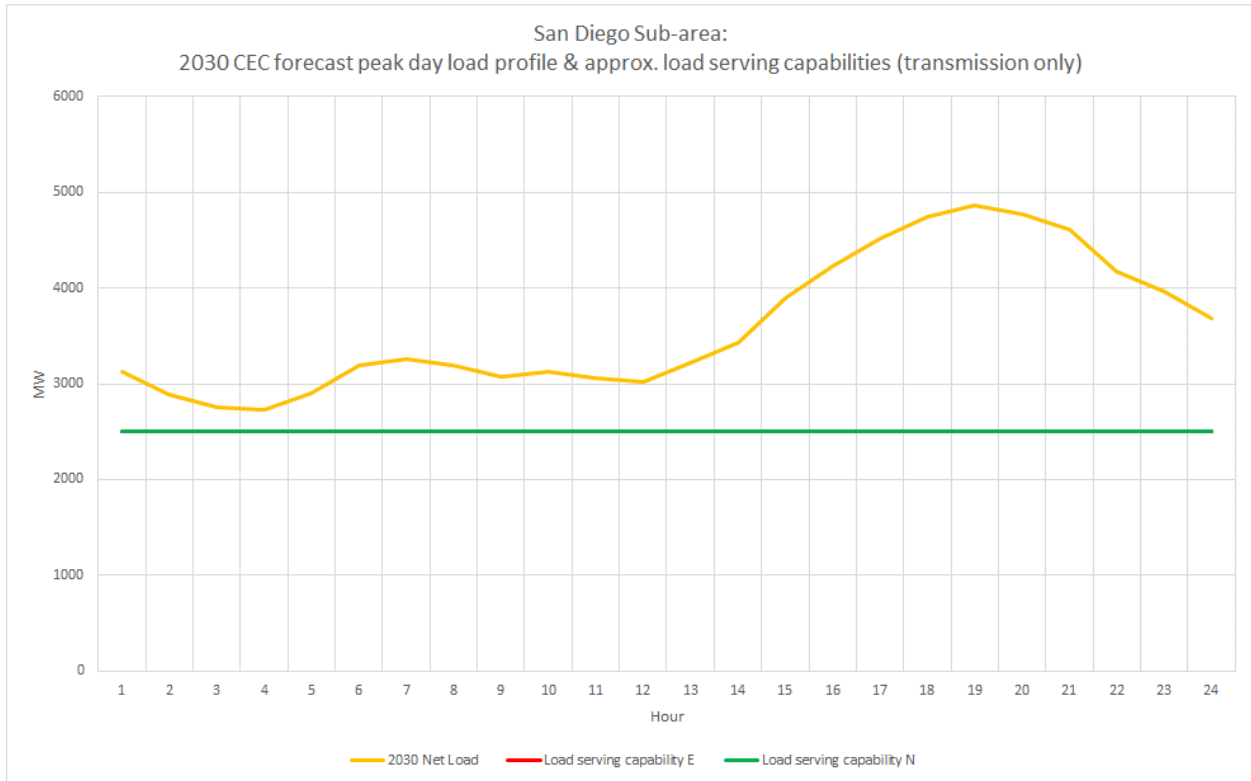
Figure 3-92 San Diego LCR sub-area 2030 Hourly Load Forecast Profiles with Transmission Only Load Serving Capability
