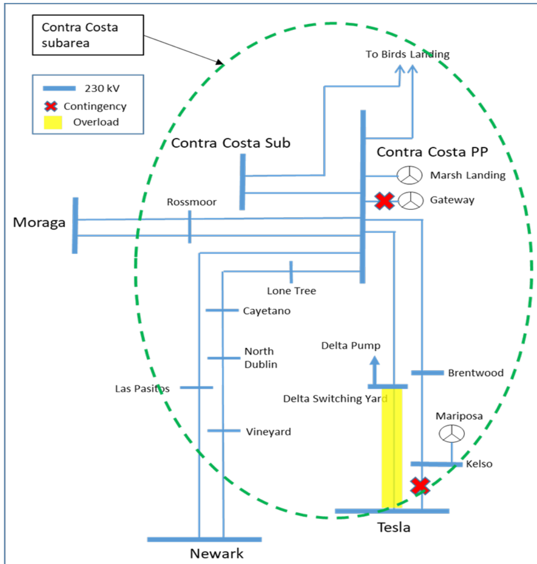
Figure 3.6-31 Contra Costa LCR Sub-area
