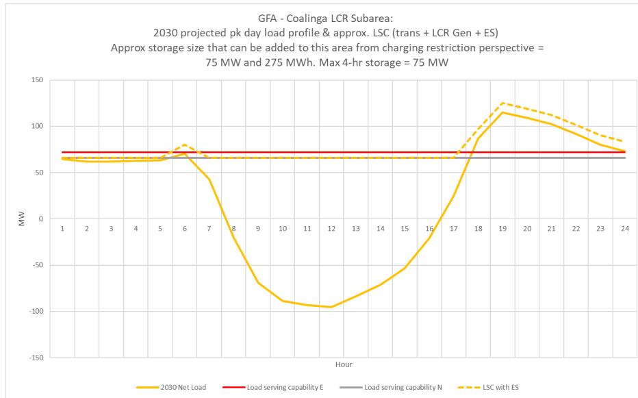
Figure 3.6-40 Coalinga LCR Sub-area 2030 Forecast Hourly Profiles
