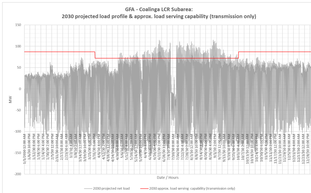
Figure 3.6-40 Coalinga LCR Sub-area 2030 Forecast Hourly Profiles
