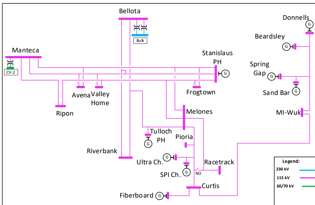
Figure 3.6-15 Stanislaus LCR Sub-area
