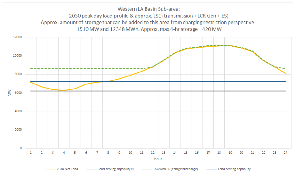
Figure 3.6-80 LCR Sub-area 2030 Estimated Amount of Storage that Can Be Added Based on Charging Restriction
