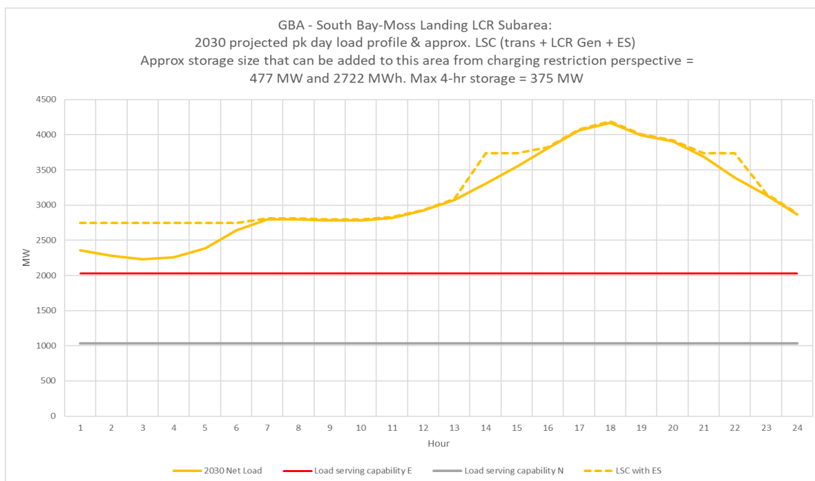
Figure 3.6-25 South Bay-Moss Landing LCR Sub-area 2030 Peak Day Forecast Profiles
