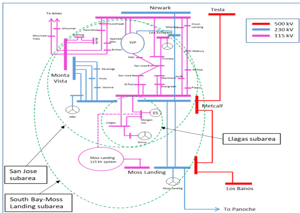
Figure 3.6-20 Llagas LCR Sub-area
