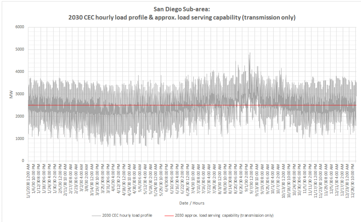
Figure 3-93 San Diego LCR Sub-area 2030 Estimated Amount of Storage that Can Be Added Based on Charging Restriction
