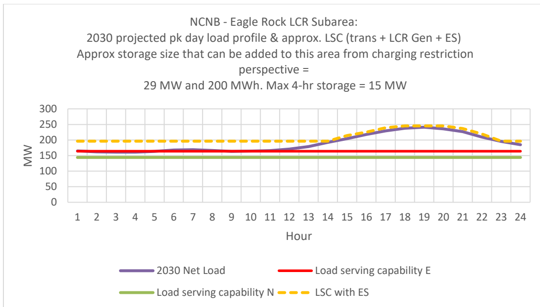
Figure 3.6-9 Eagle Rock LCR Sub-area 2030 Forecast Hourly Profiles
