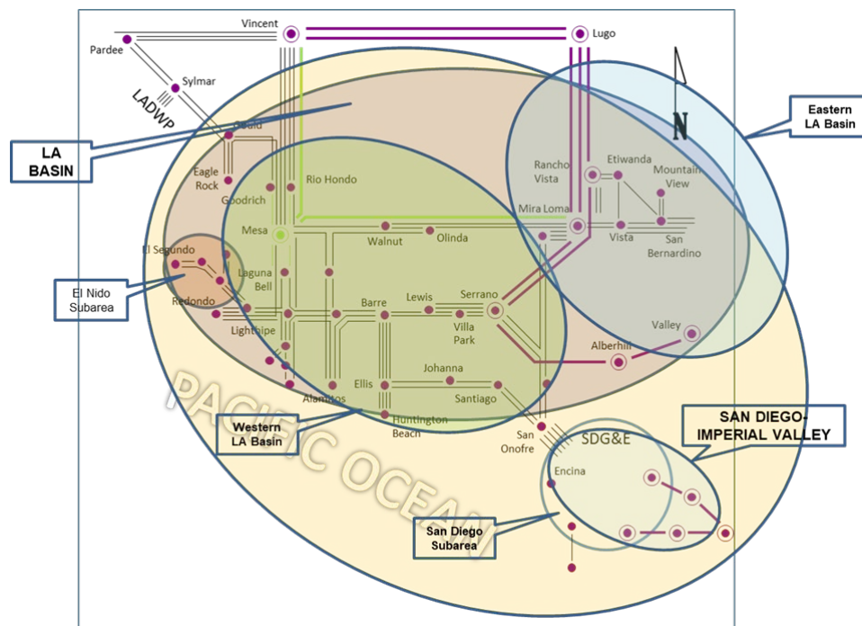
Figure 3.6-87 San Diego-Imperial Valley LCR Area
