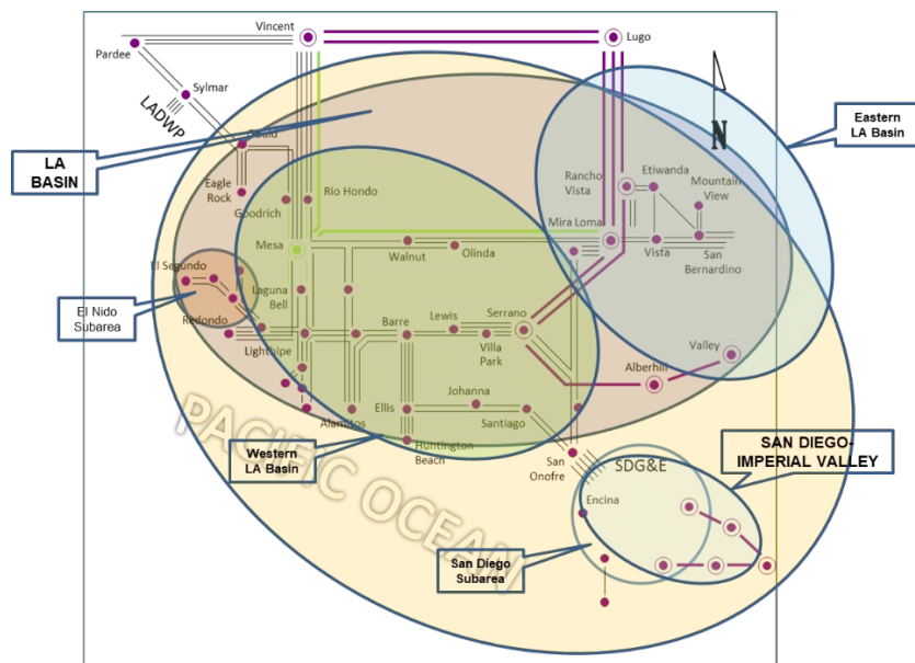
Figure 3.6-74 LA Basin LCR Area
