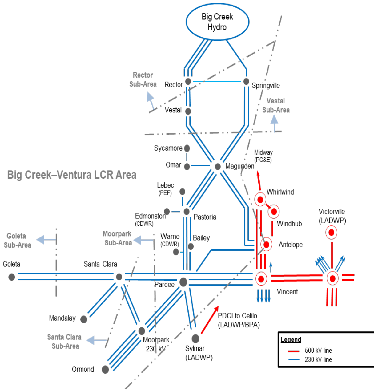
Figure 3.6-65 Big Creek/Ventura LCR Area
