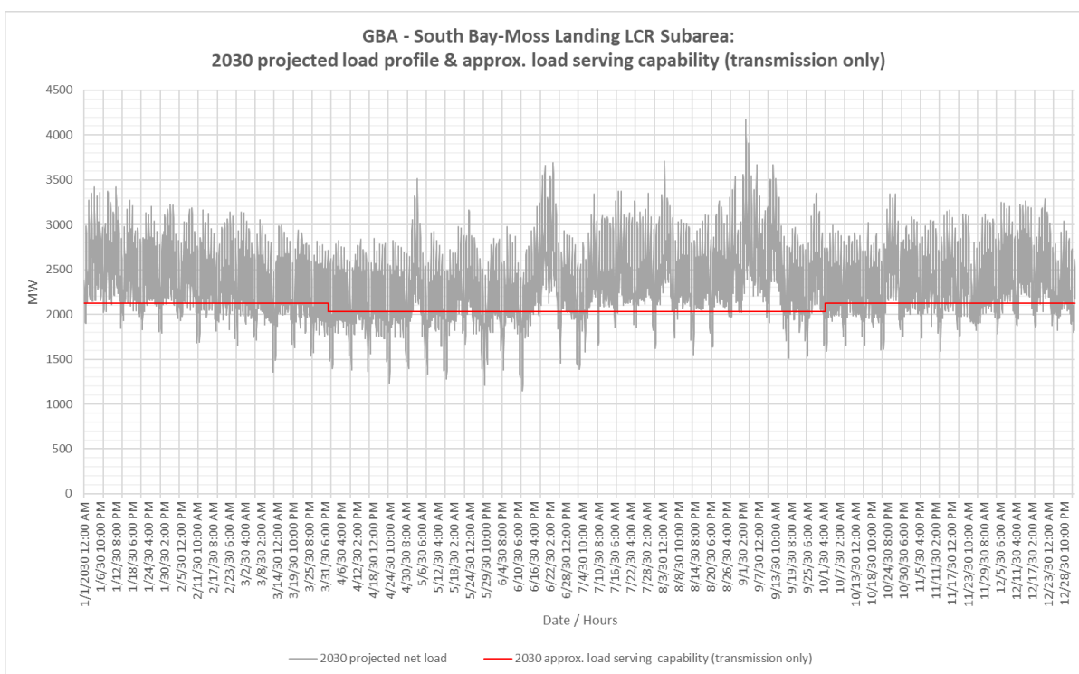
Figure 3.6-26 South Bay-Moss Landing LCR Sub-area 2030 Forecast Hourly Profiles
