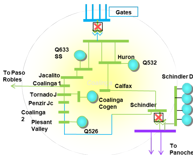
Figure 3.6-38 Coalinga LCR Sub-area
