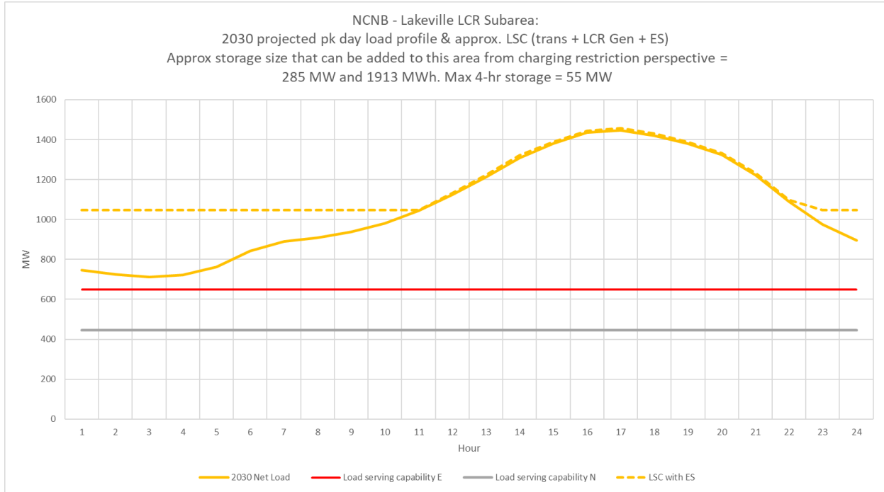
Figure 3.6-6 North Coast and North Bay 2030 Forecast Hourly Profile
