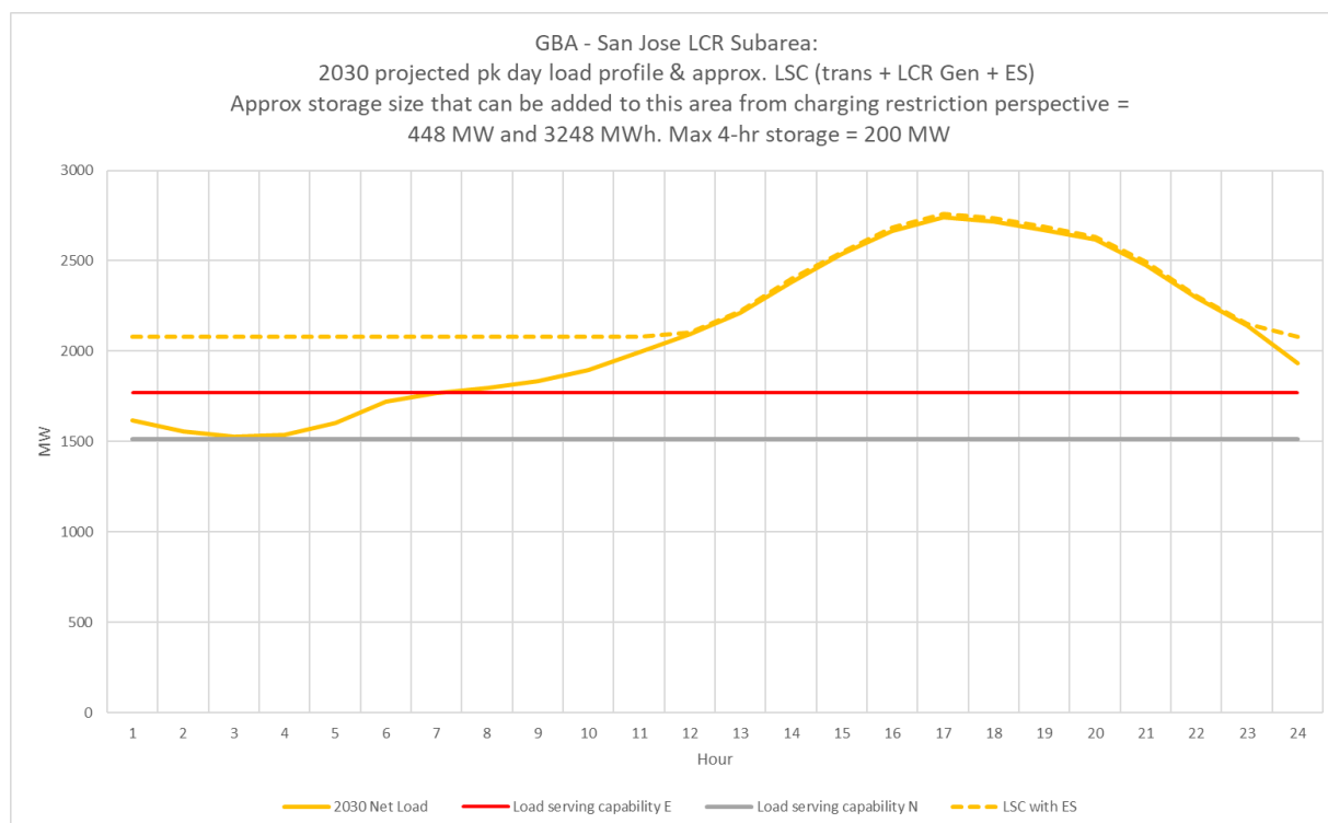
Figure 3.6-23 San Jose LCR Sub-area 2030 Peak Day Forecast Profiles
