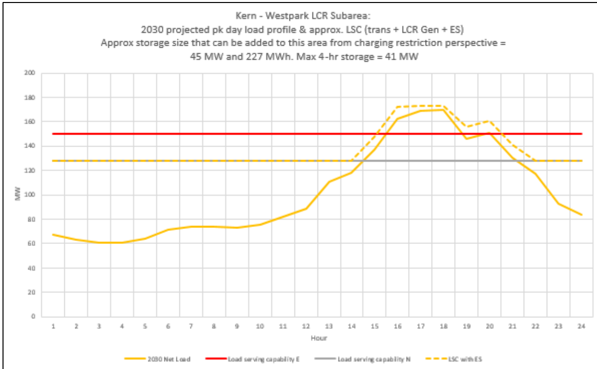
Figure 3.6-55 Westpark LCR Sub-area 2030 Forecast Hourly Profiles
