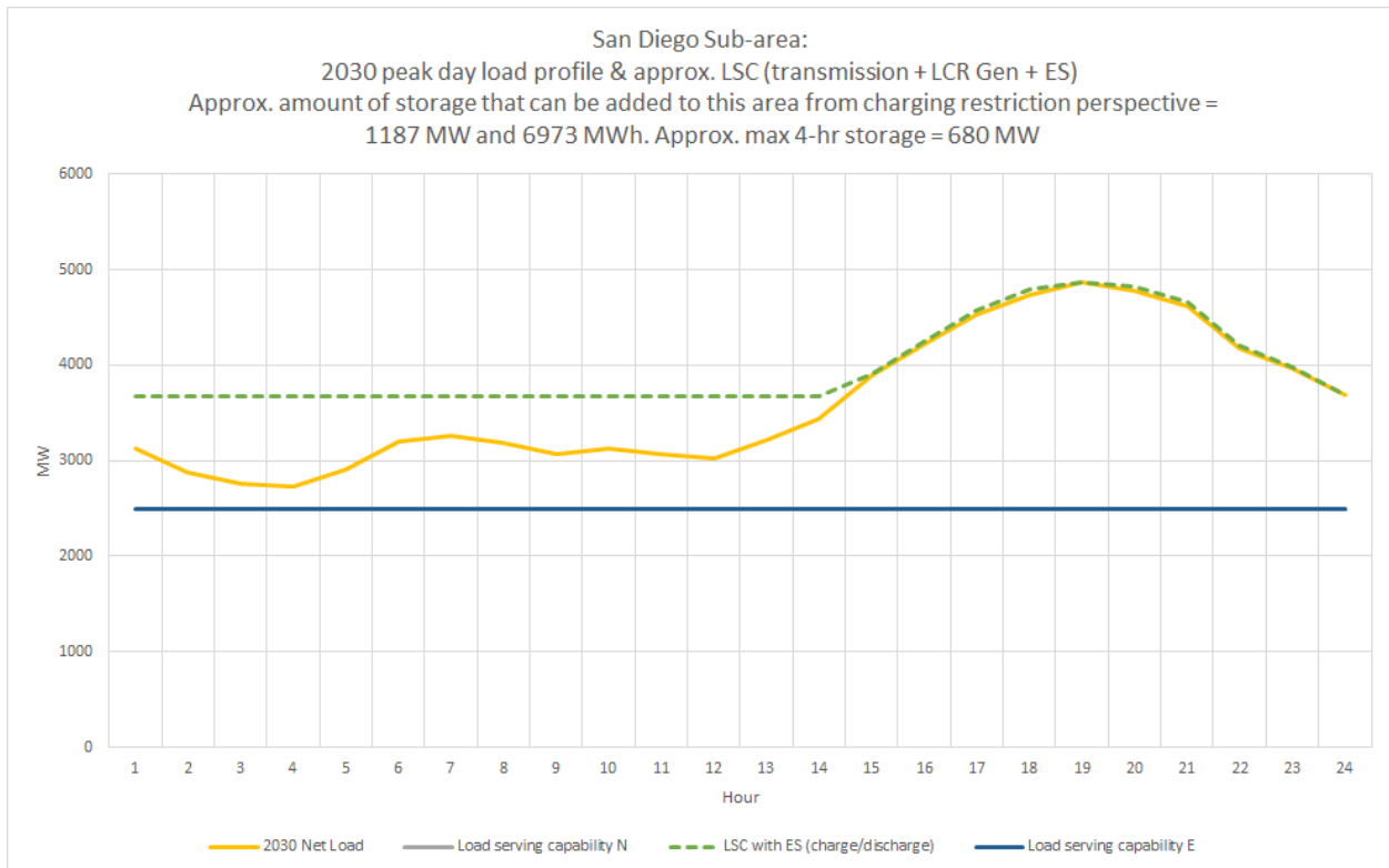
Figure 3-93 San Diego LCR Sub-area 2030 Estimated Amount of Storage that Can Be Added Based on Charging Restriction
