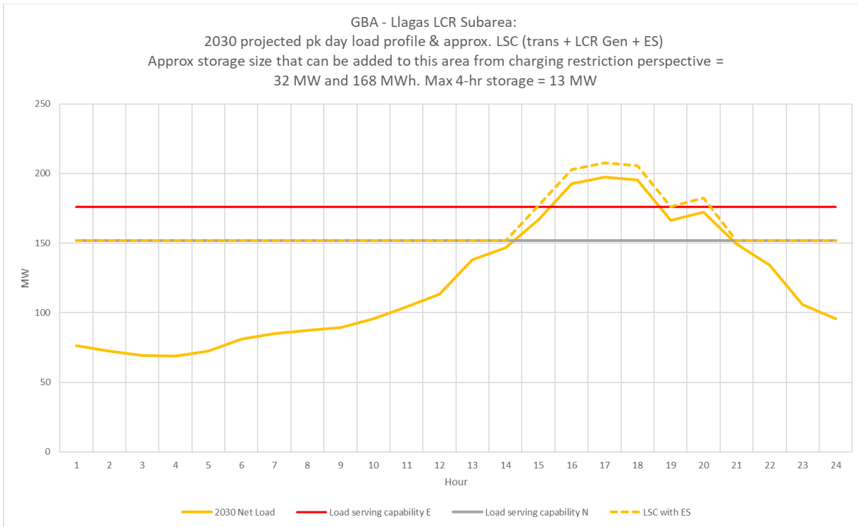
Figure 3.6-22 Llagas LCR Sub-area 2030 Forecast Hourly Profiles
