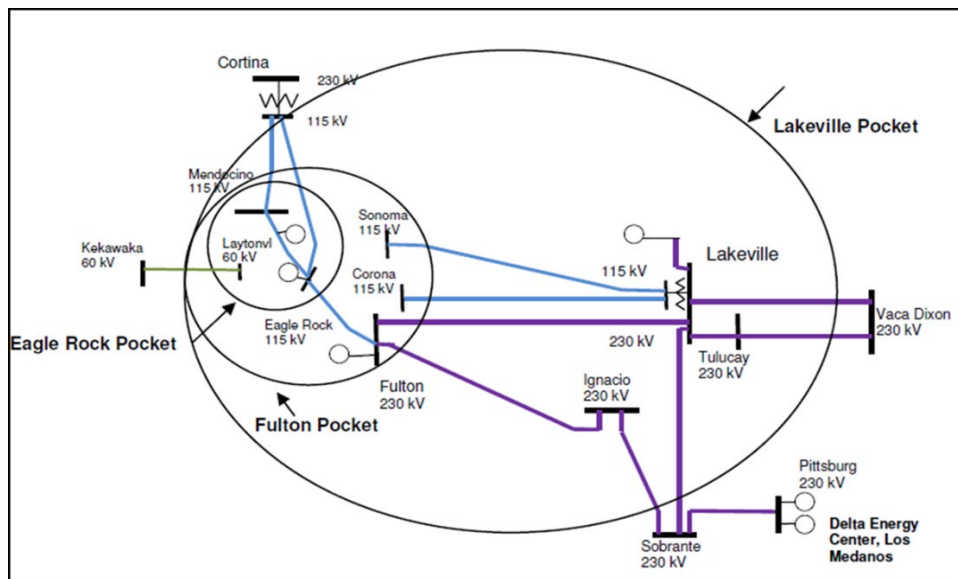
Figure 3.6-4 North Coast and North Bay LCR Area
