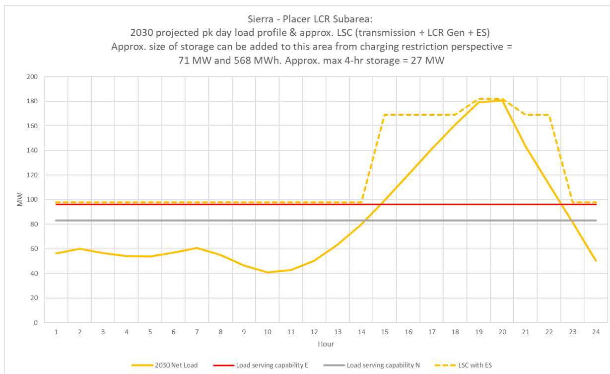
Figure 3.6-13 Placer LCR Sub-area 2030 Forecast Hourly Profiles
