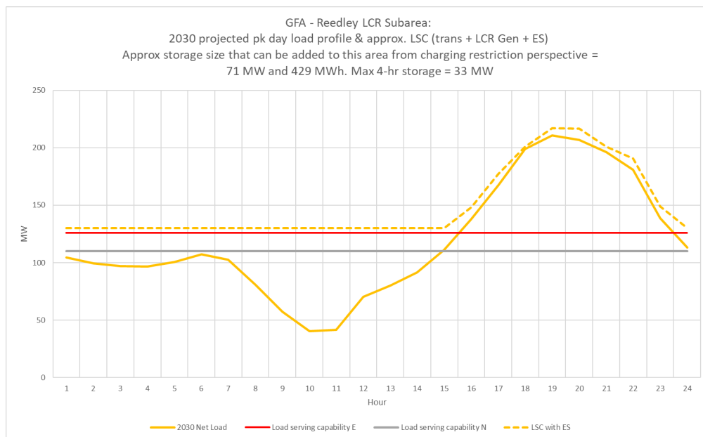
Figure 3.6-43 Reedley LCR Sub-area 2030 Forecast Hourly Profiles
