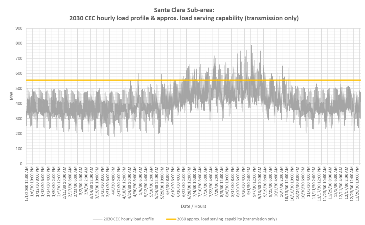
Figure 3.6-71 Santa Clara Sub-area 2030 Forecast Hourly Profiles
