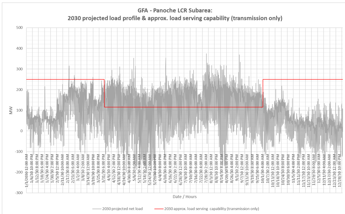
Figure 3.6-46 Panoche LCR Sub-area 2030 Forecast Hourly Profiles
