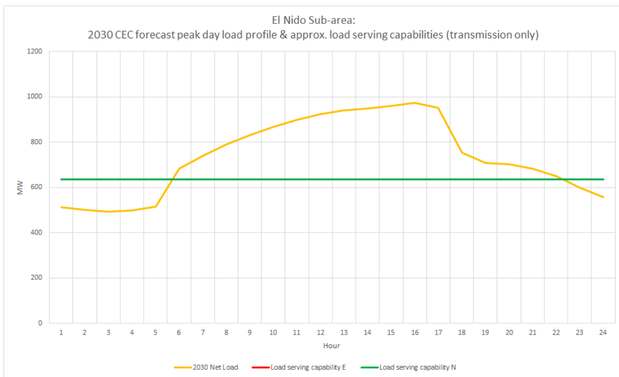
Figure 3.6-75 El Nido LCR Sub-area 2030 Peak Day Forecast Profiles
