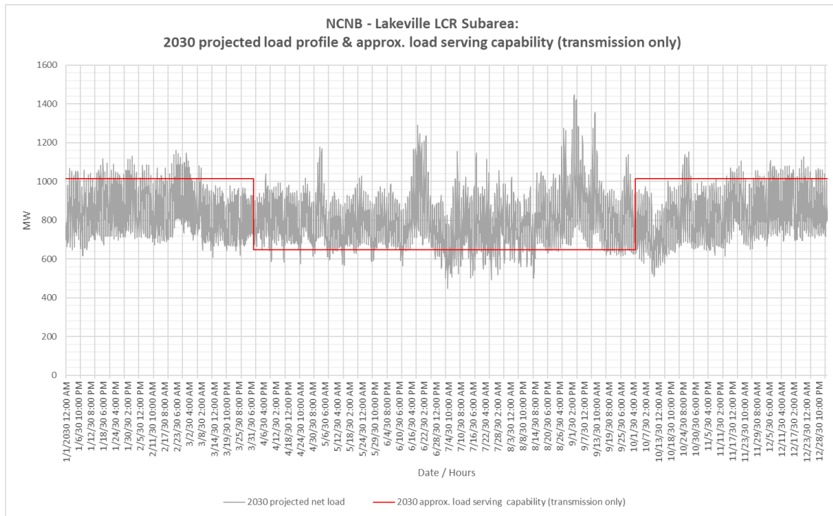
Figure 3.6-6 North Coast and North Bay 2030 Forecast Hourly Profile
