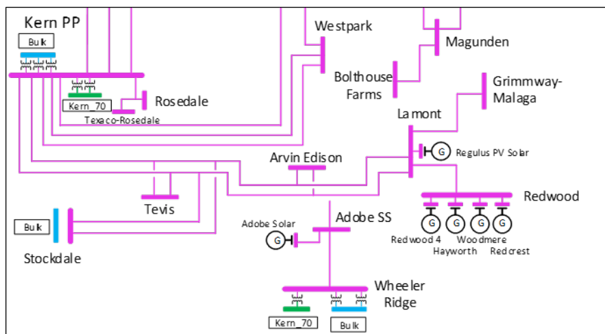
Figure 3.6-59 Kern PP-Tevis 115 kV LCR Sub-area
