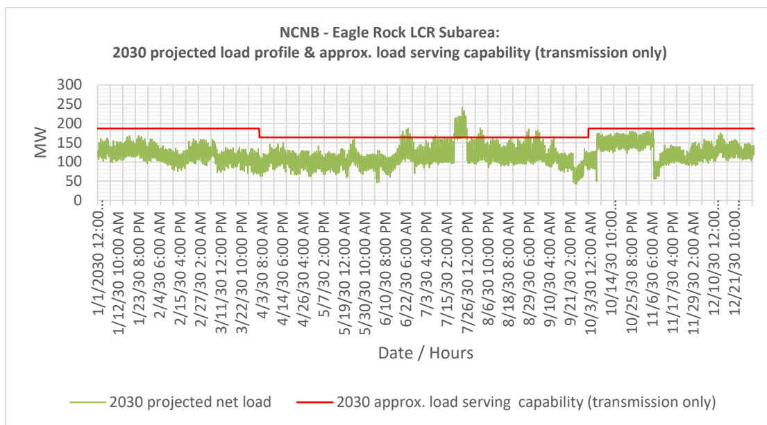
Figure 3.6-9 Eagle Rock LCR Sub-area 2030 Forecast Hourly Profiles
