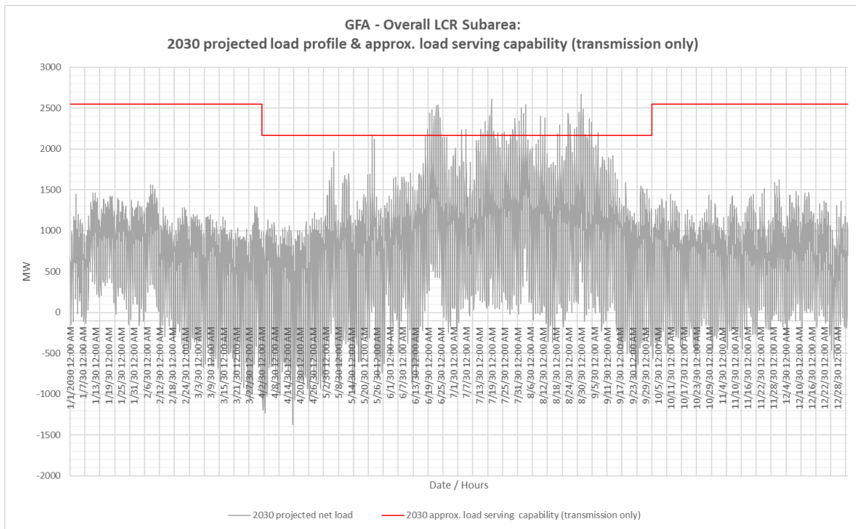
Figure 3.6-52 Greater Fresno Overall LCR Area 2030 Forecast Hourly Profiles
