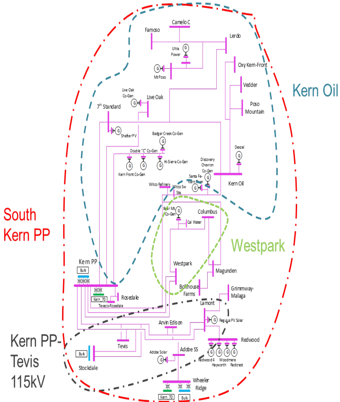
Figure 3.6-53 Kern LCR Area
