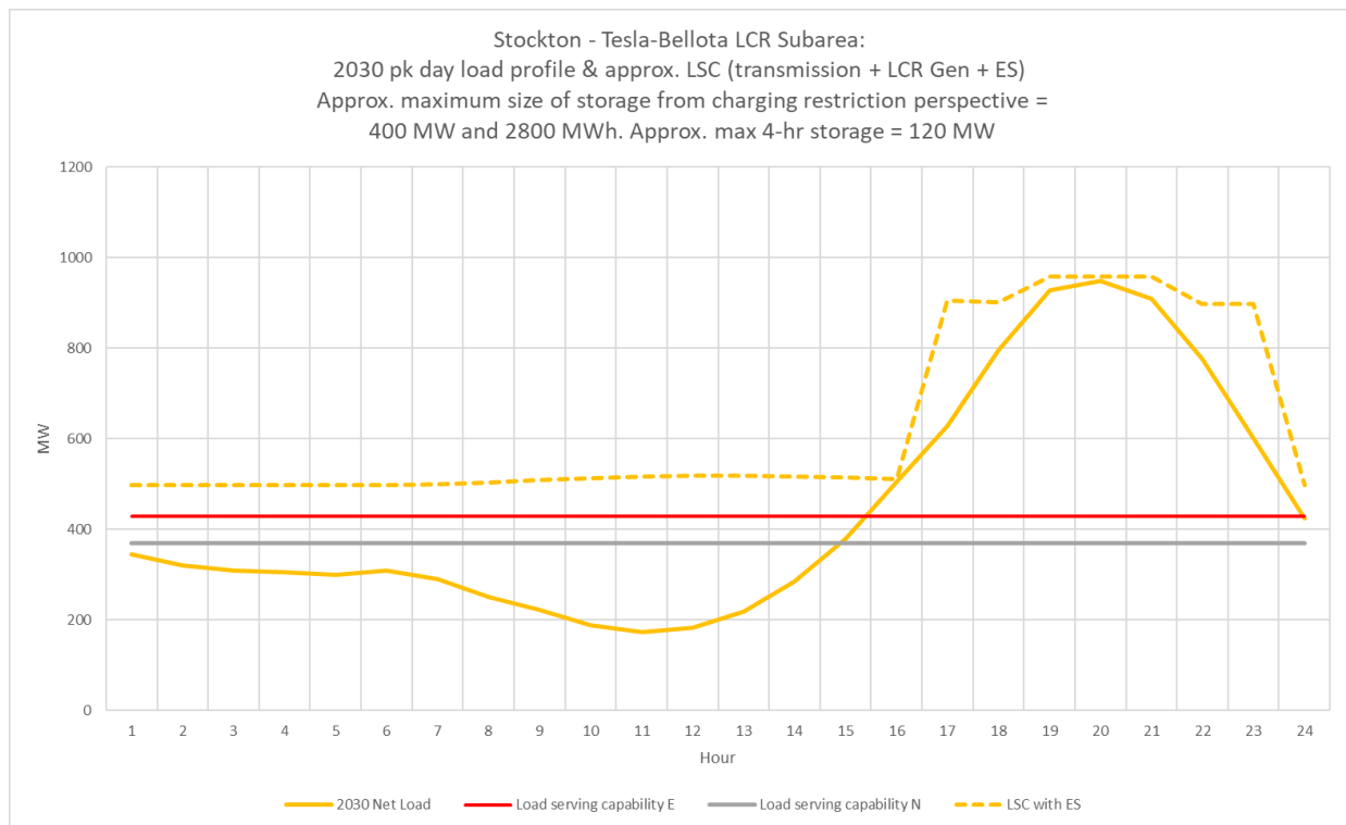
Figure 3.6-17 Tesla-Bellota LCR Sub-area 2030 Peak Day Forecast Profiles
