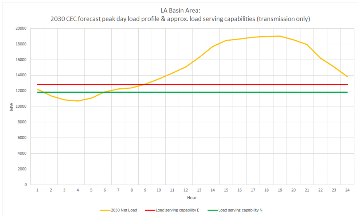
Figure 3.6-84 Overall LA Basin LCR area 2030 Peak Day Forecast Profiles
