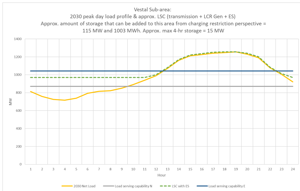
Figure 3.6-68 Vestal Sub-area 2030 Forecast Hourly Profile
