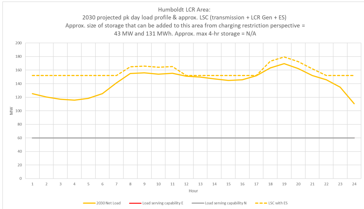
Figure 3.6-3 Humboldt 2030 Forecast Hourly Profile
