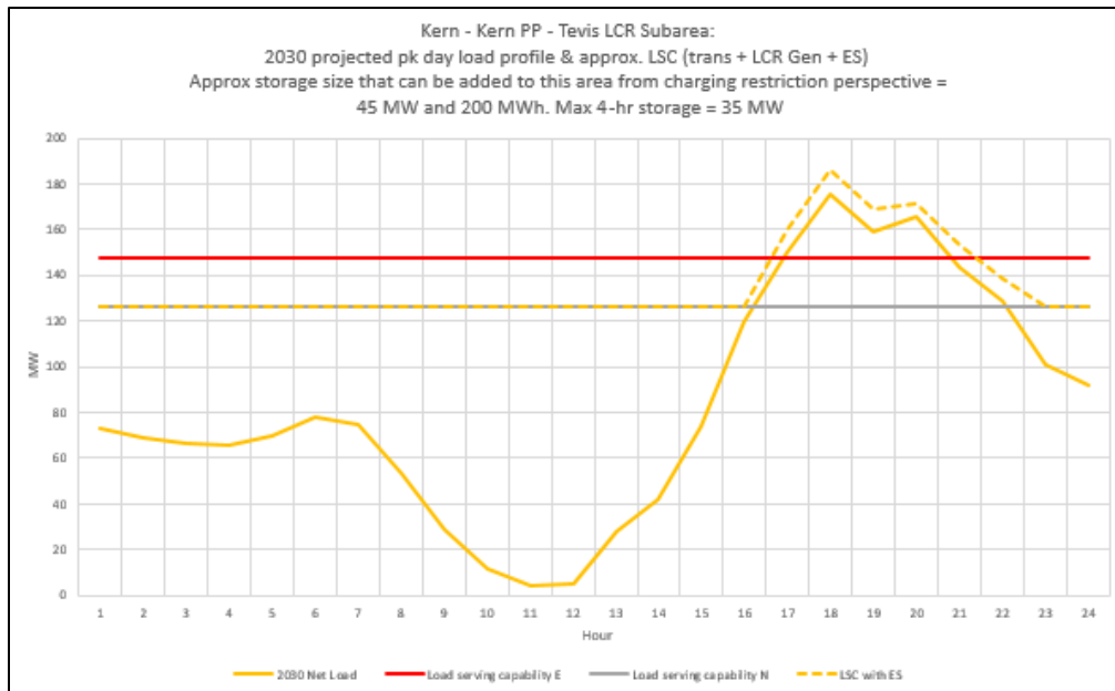
Figure 3.6-61 Kern PP-Tevis LCR Sub-area 2030 Forecast Hourly Profiles
