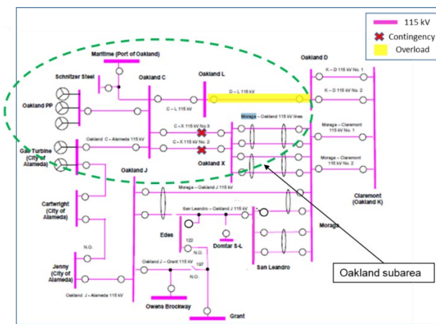
Figure 3.6-27 Oakland LCR Sub-area
