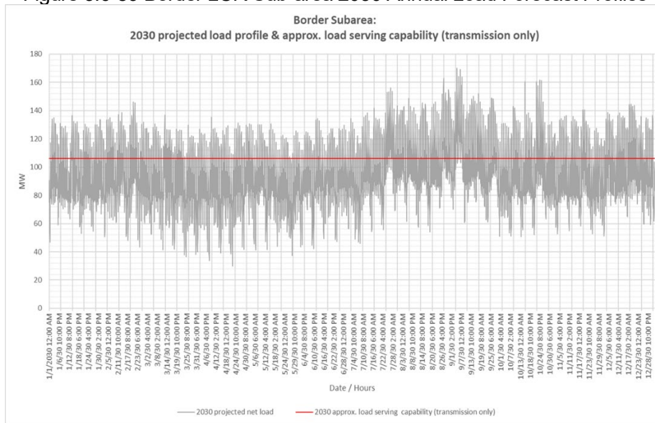
Figure 3.6-89 Border LCR Sub-area 2030 Annual Load Forecast Profiles
