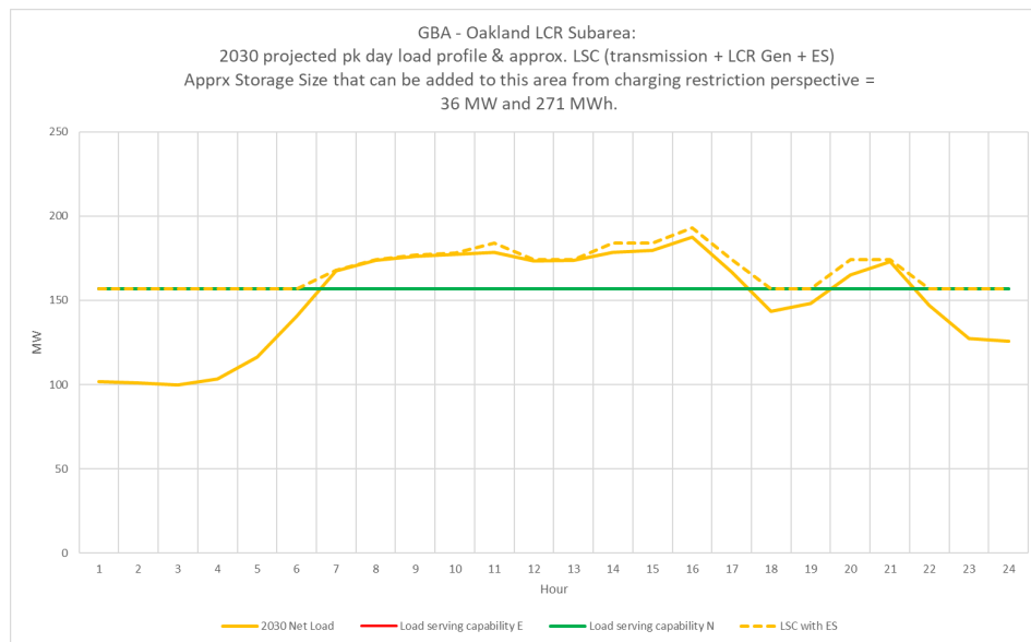
Figure 3.6-29 Oakland LCR Sub-area 2030 Forecast Hourly Profiles
