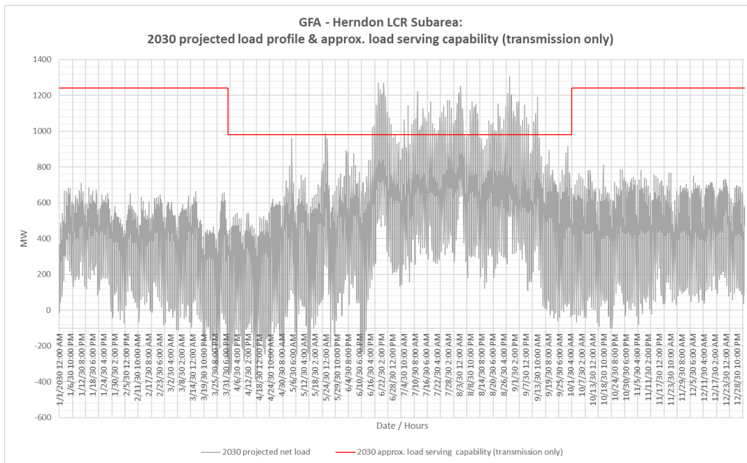
Figure 3.6-49 Herndon LCR Sub-area 2030 Forecast Hourly Profiles
