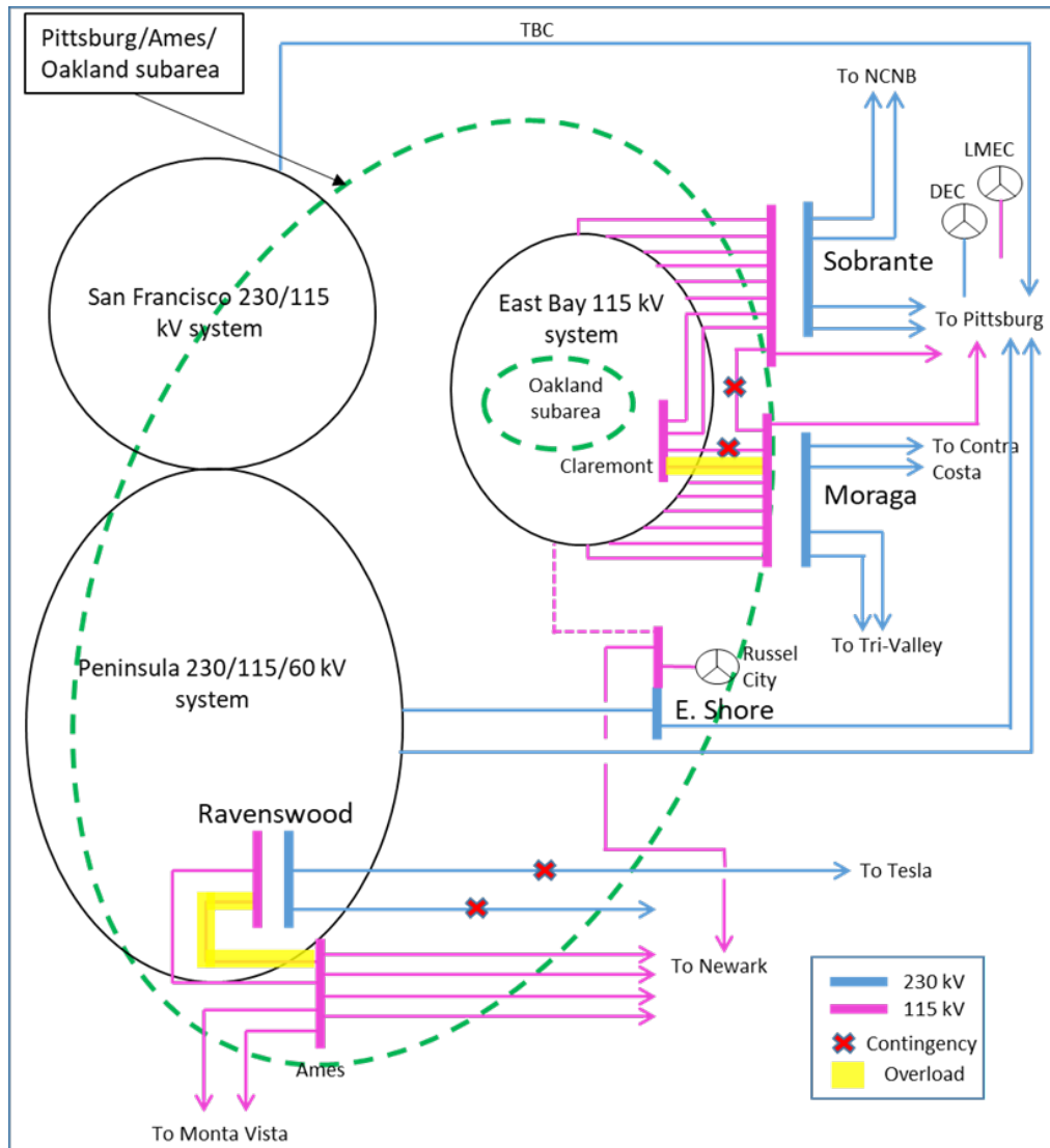
Figure 3.6-30 Ames-Pittsburg-Oakland LCR Sub-area
