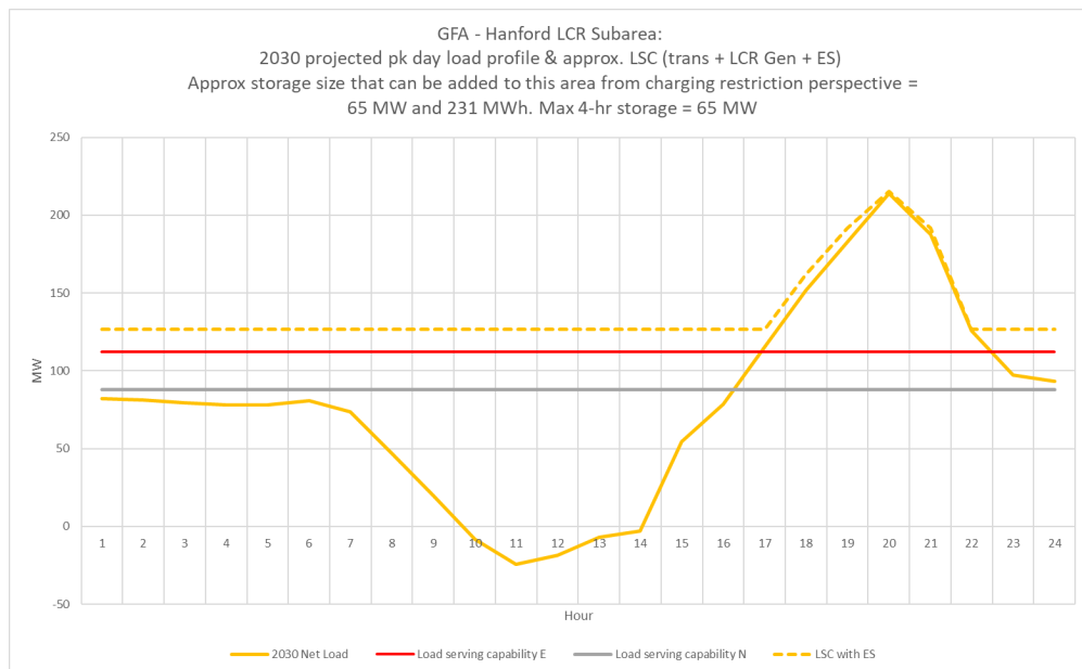
Figure 3.6-37 Hanford LCR Sub-area 2030 Forecast Hourly Profiles
