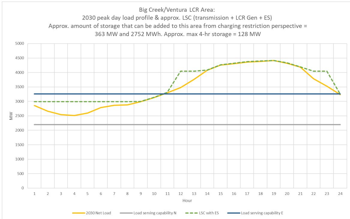
Figure 3.6-73 Big Creek/Ventura LCR area 2030 Peak Day Forecast Profiles
