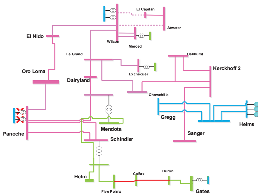
Figure 1.6-56 Panoche LCR Sub-area
