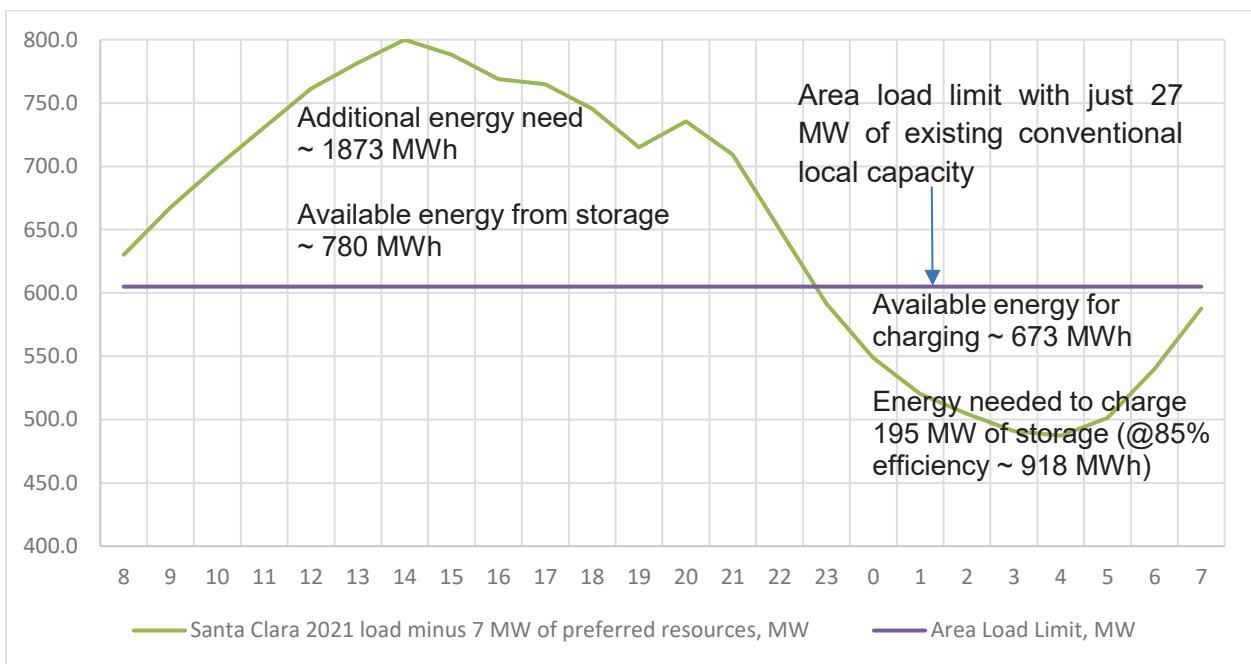
Figure 1.6-83 Santa Clara Sub-area Stoage Analysis
