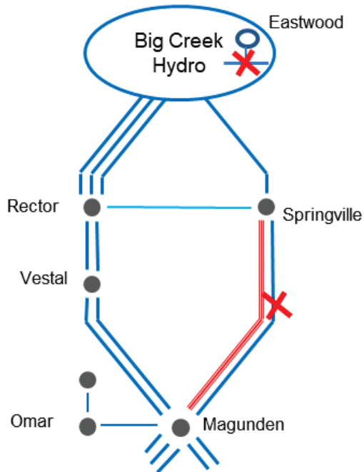
Figure 1.6-79 Vestal LCR Sub-area
