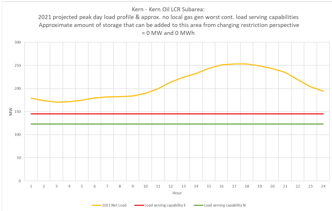
Figure 1.6-74 Kern Oil LCR Sub-area 2021 Forecast Hourly Profiles
