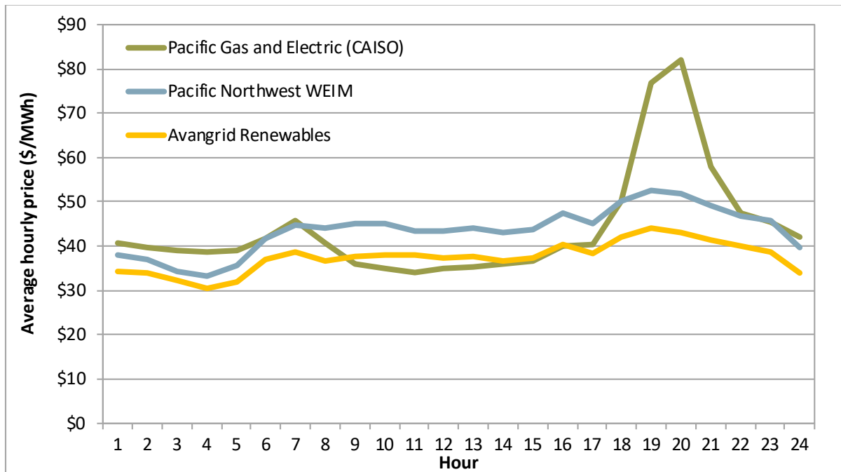
Figure 1.1 Average hourly 15-minute price (September 2023)
