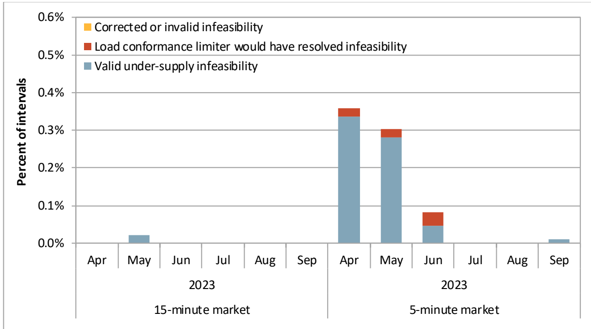
Figure 1.3 Frequency of under-supply power balance infeasibilities by month Avangrid Renewables
