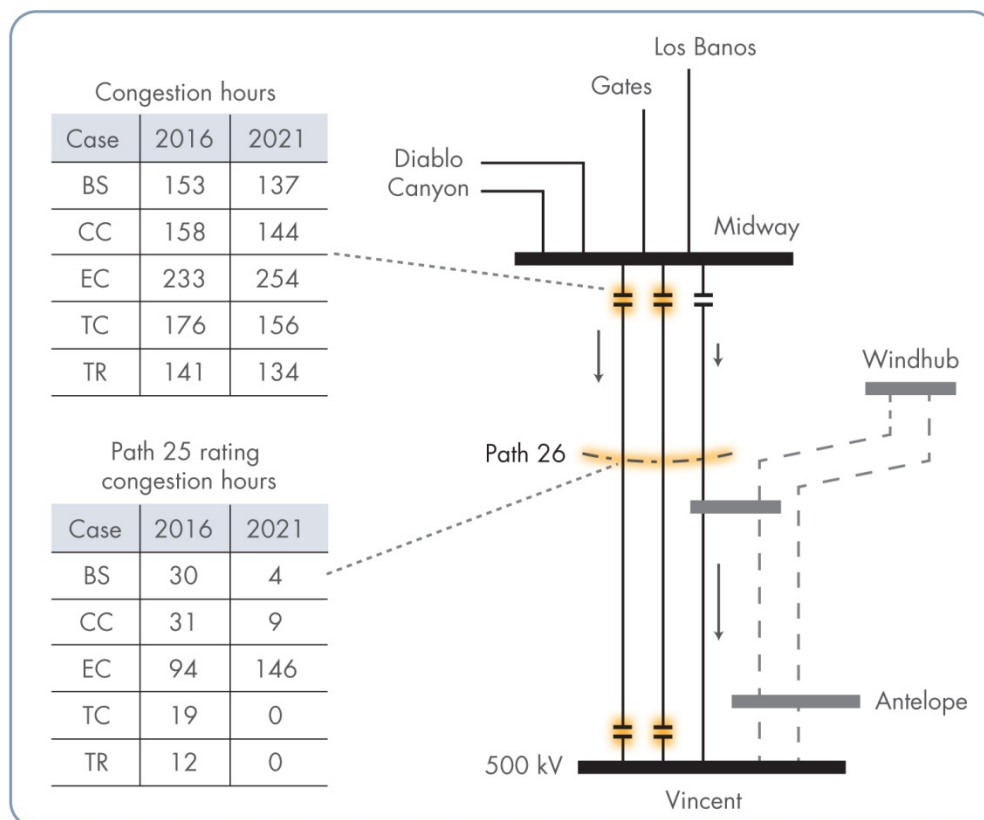
Figure 5.6-2: Path 26 system diagram and simulated congestion hours
