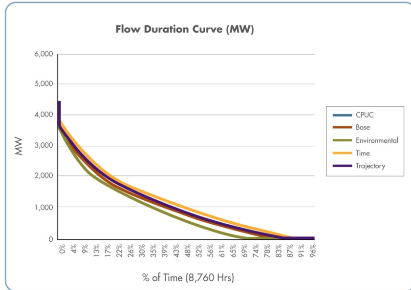
Figure 4.6-18 Delivered energy on COI
