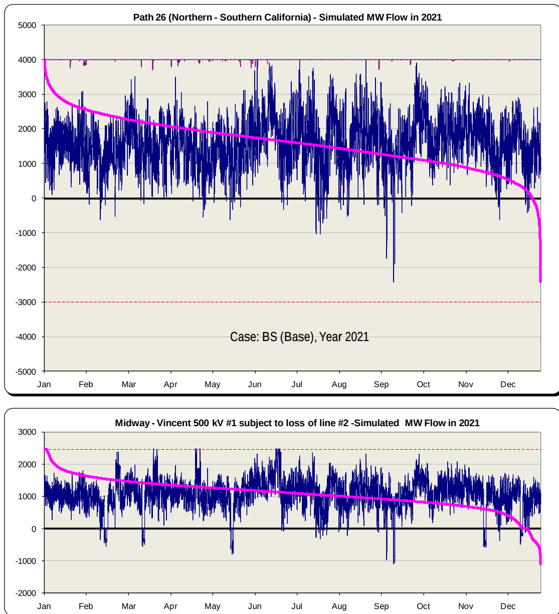
Figure 5.6-3: Simulated Power Flow on Path 26
