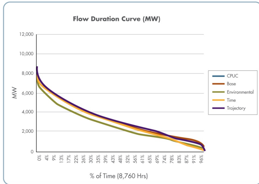
Figure 4.6-10 Delivered Energy on West of River
