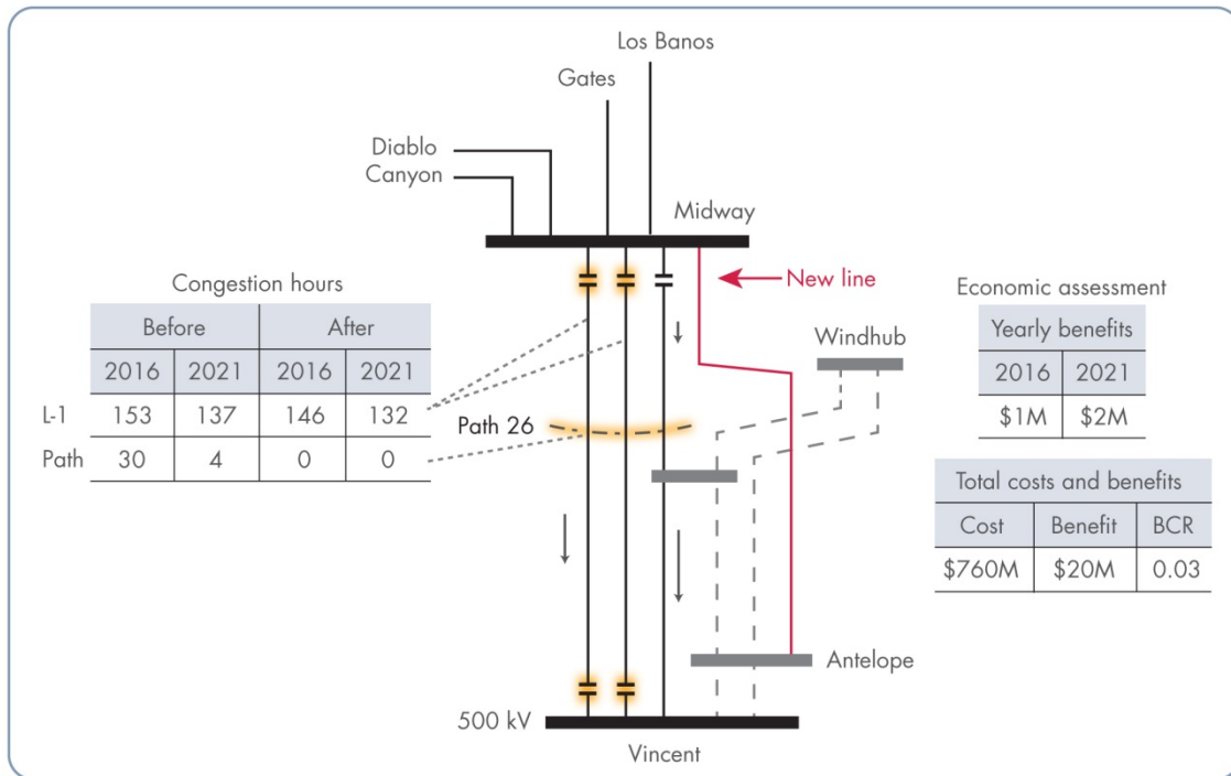
Figure 5.6-6: Alternative 3: Build Midway – Antelope 500 kV line
