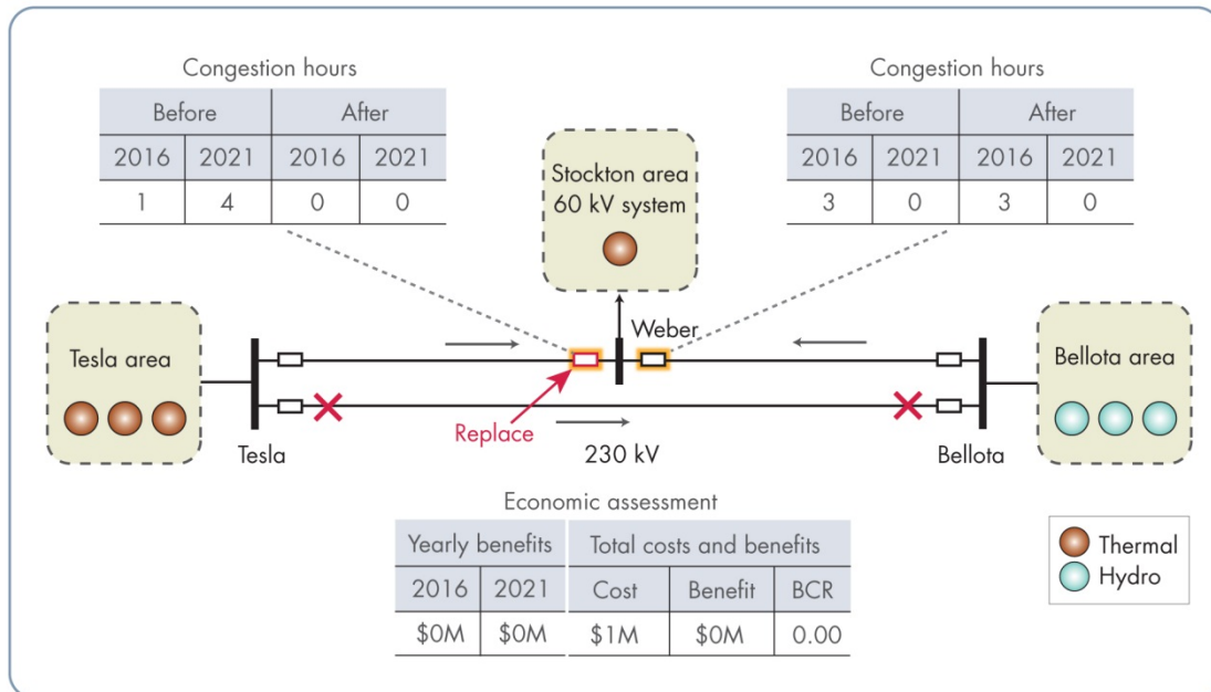
Figure 5.6-27: Alternative 1: Replace Weber circuit breaker for the Tesla-Weber 230 kV line
