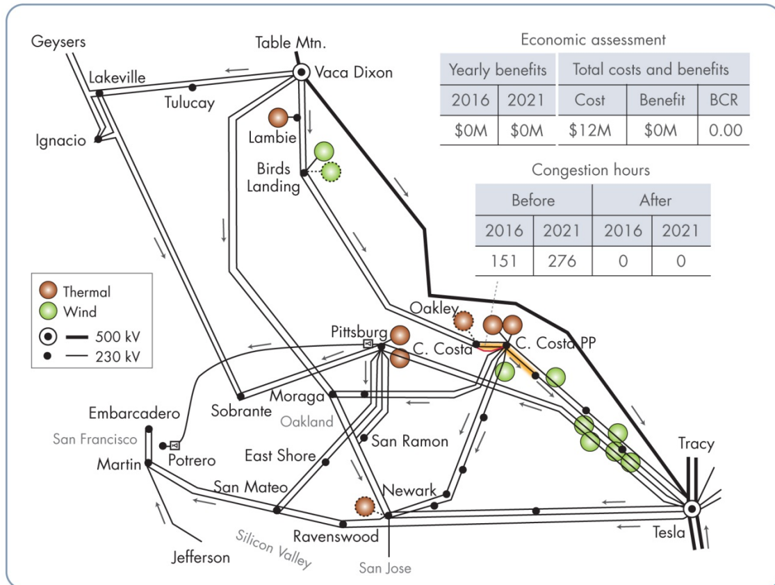
Figure 5.6-14: Alternative 2: Build Contra Costa Sub-Contra Costa PP 230 kV line #2
