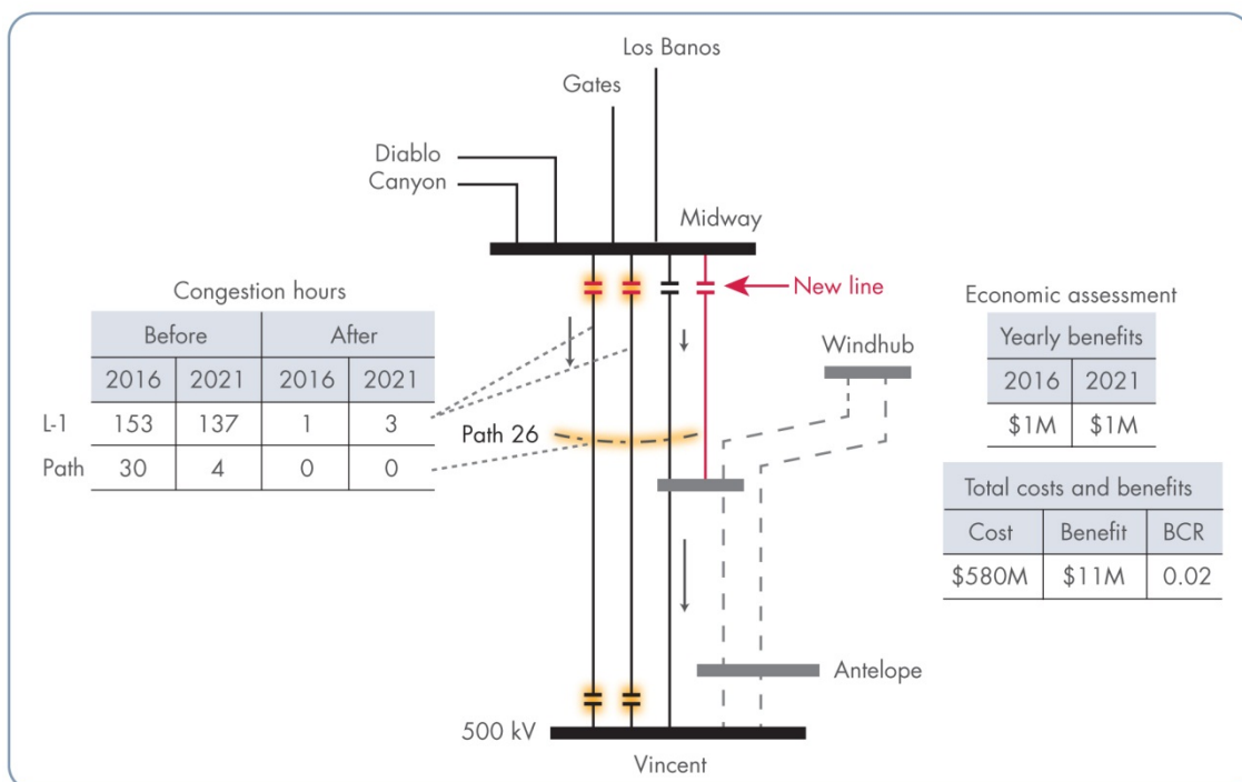
Figure 5.6-5: Alternative 2: Build Midway – Whirlwind 500 kV line #2
