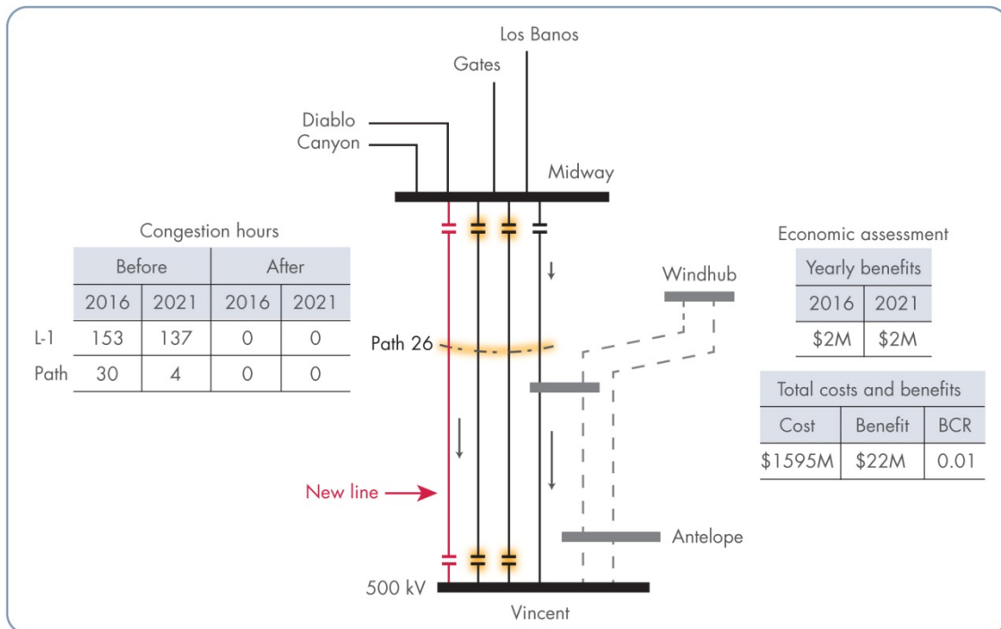
Figure 5.6-7: Alternative 4: Build Midway – Vincent 500 kV line #4
