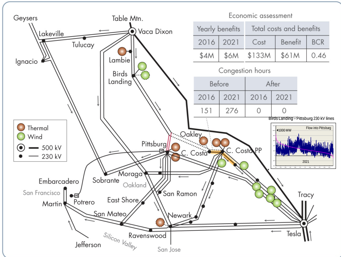
Figure 5.6-15: Alternative 3: Divert Birds Landing-Contra Costa 230 kV lines to Pittsburg
