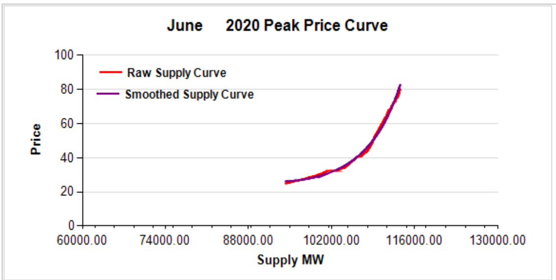
FIGURE 2: June 2020 ON-PEAK REGRESSION RESULT
