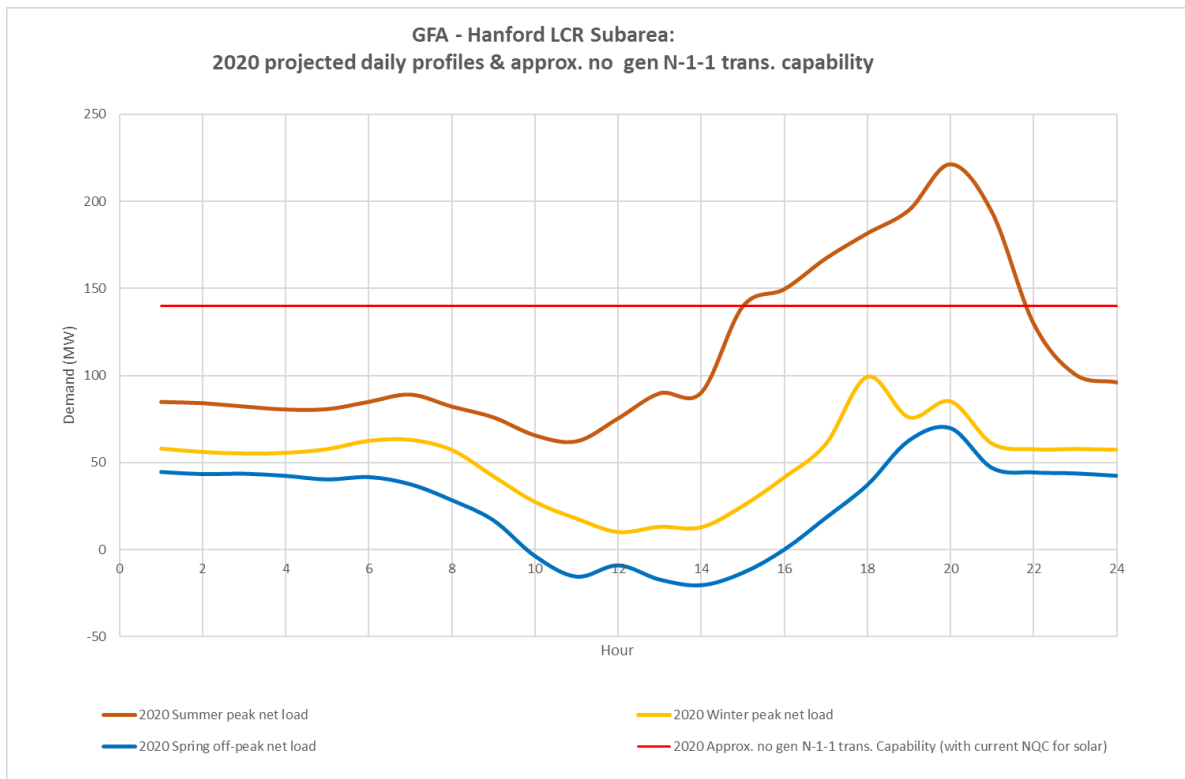
Figure 3.3-65 Hanford LCR Sub-area 2020 Forecast Hourly Profiles
