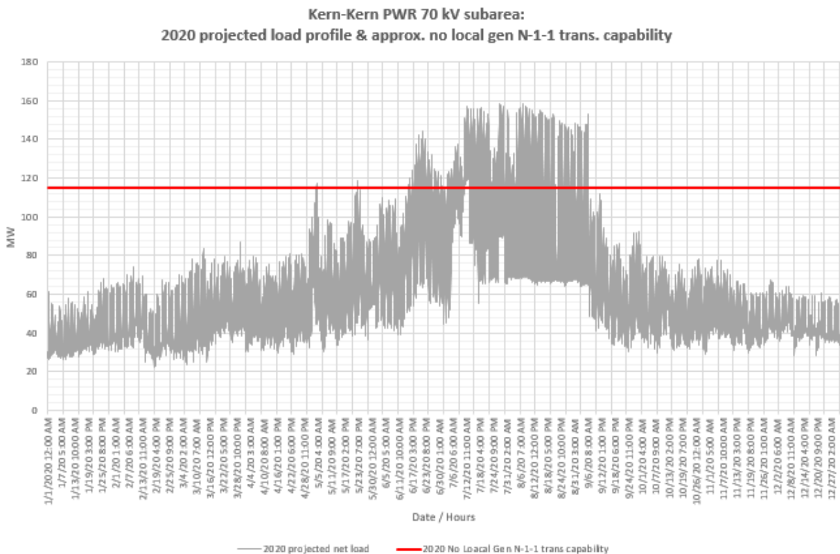
Figure 3.3-84 Kern 70 kV LCR Sub-area 2020 Forecast Hourly Profiles
