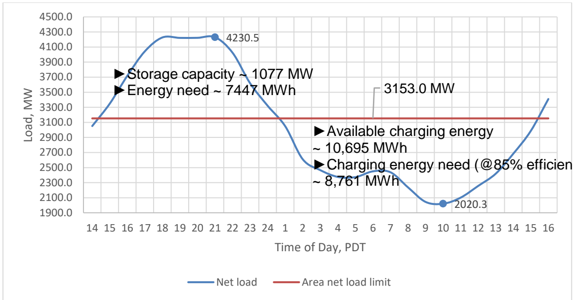
Figure 3.2-80 Big Creek/Ventura Local Capacity Energy Storage Analysis with Sylmar–Pardee Project
