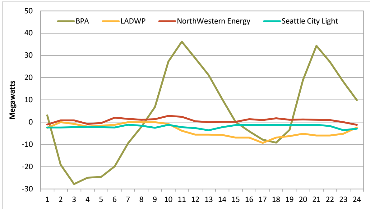
Figure 5.3 Average hourly 15-minute market load conformance (January 2023)
