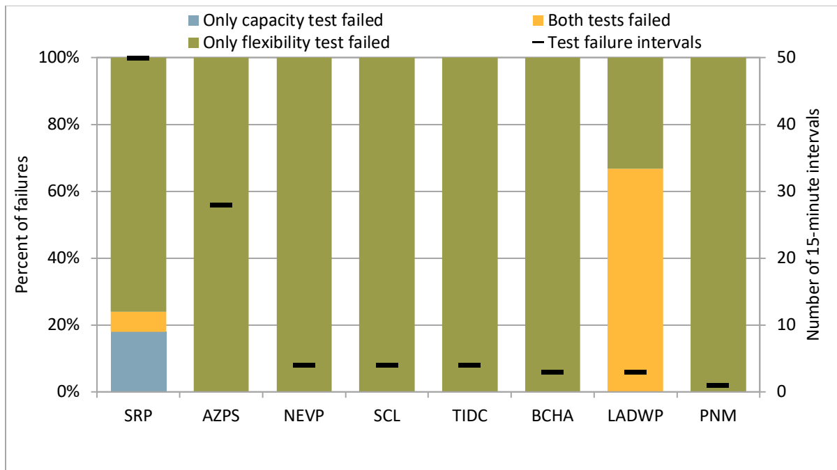
Figure 3.10 Downward capacity/flexibility test failure intervals by concurrence (January 2023)
