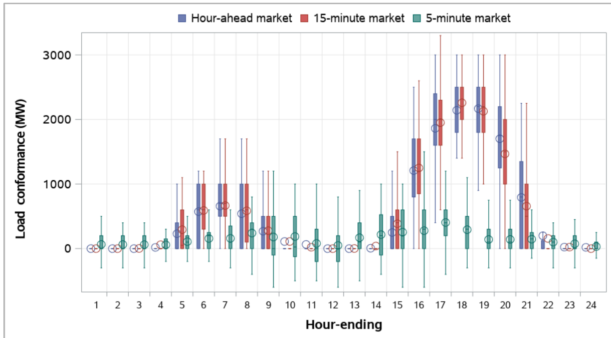
Figure 5.2 Distribution of CAISO load conformance (January 2023)
