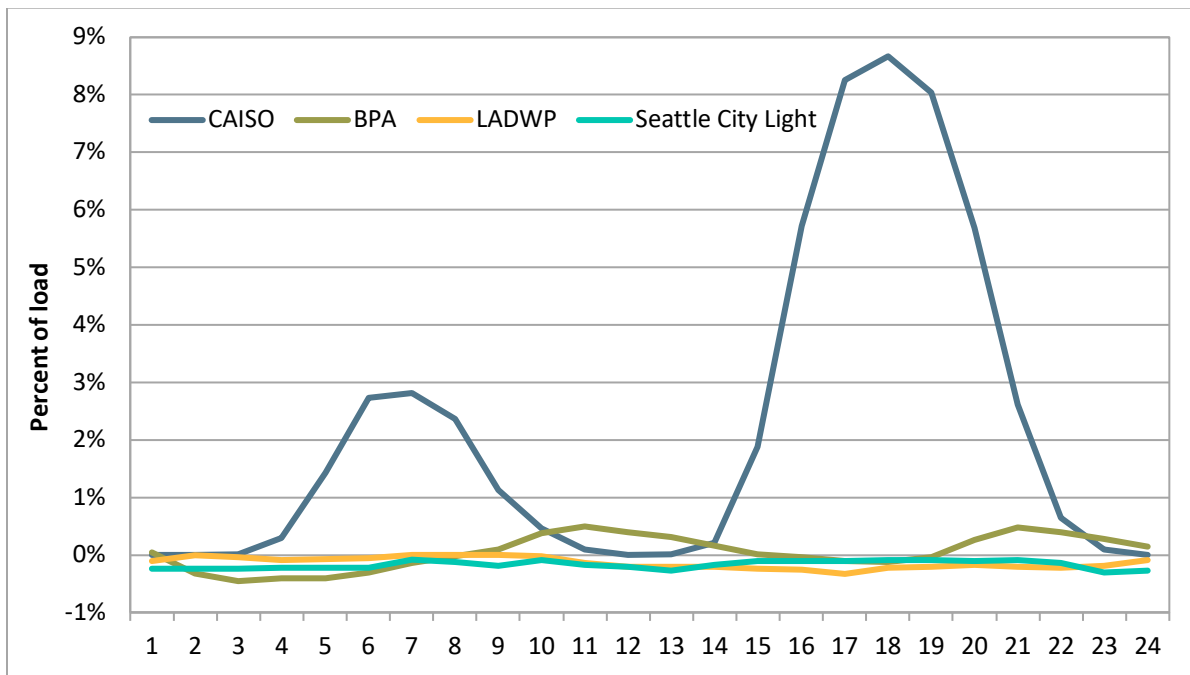
Figure 5.4 Average hourly 15-minute market load conformance as a percent of load (January 2023)
