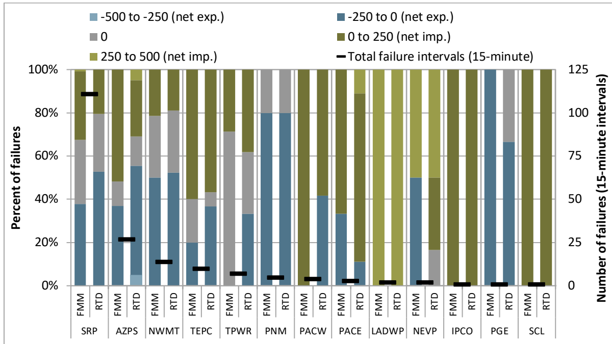
Figure 4.4 Upward test failure by dynamic net WEIM transfer amount (January 2023)
