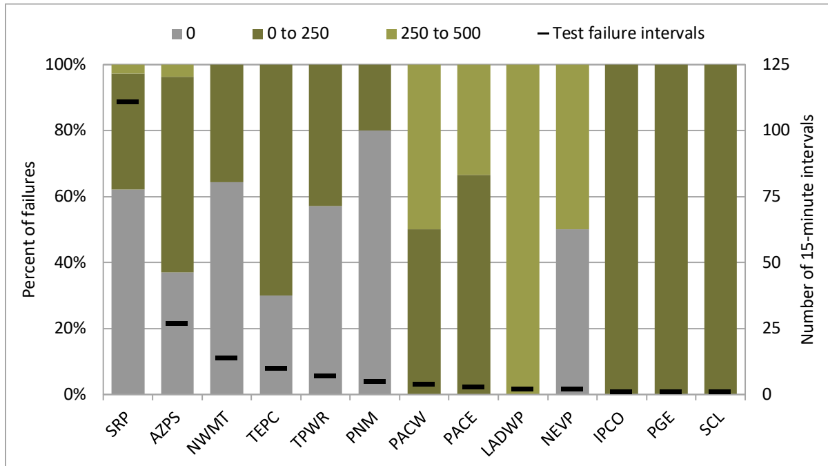
Figure 4.2 Upward capacity/flexibility test failure intervals by dynamic import limit (January 2023)
