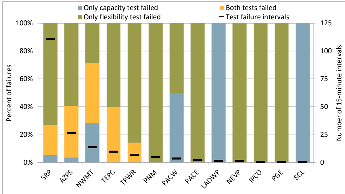
Figure 3.9 Upward capacity/flexibility test failure intervals by concurrence (January 2023)
