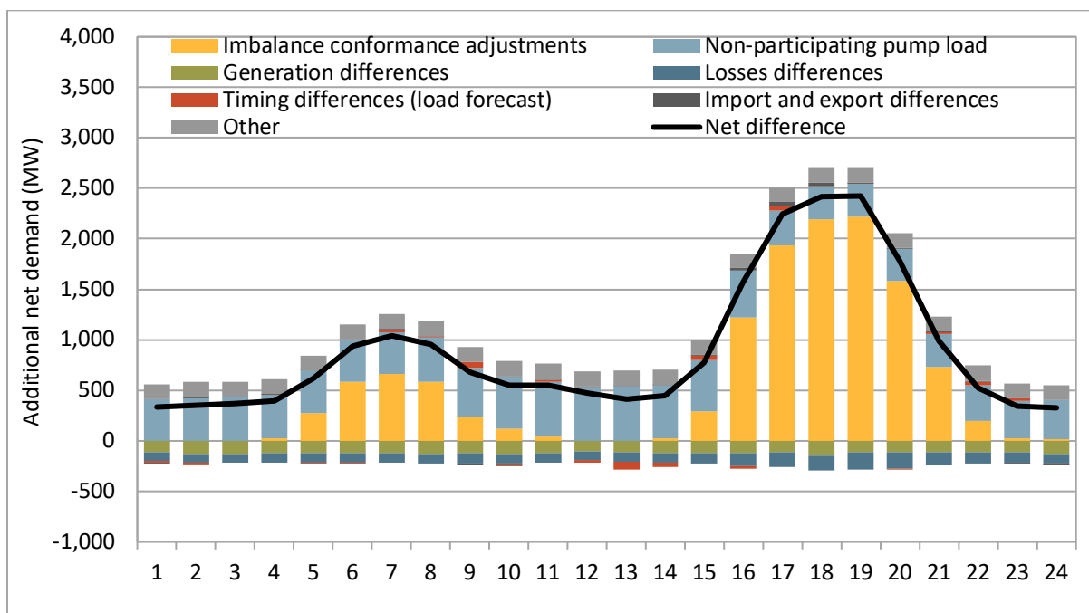
Figure 6.1 Additional CAISO net demand in the latest 15-minute market run not accounted for in the bid-range capacity test (January 2023)
