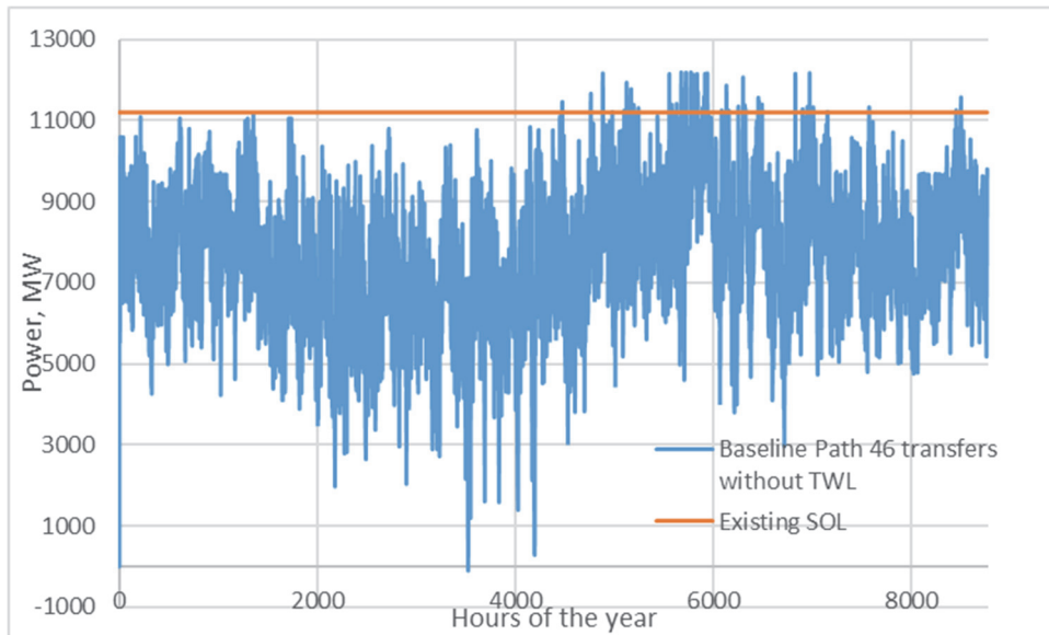
9 Figure 3: Projected Path 46 Transfers without Ten West Link in the Baseline Case
