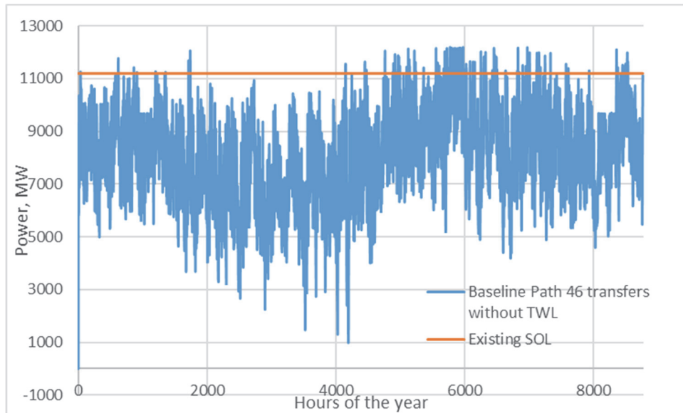
1 Figure 4: Projected Path 46 Transfers without Ten West Link in the Sensitivity 2 Case
