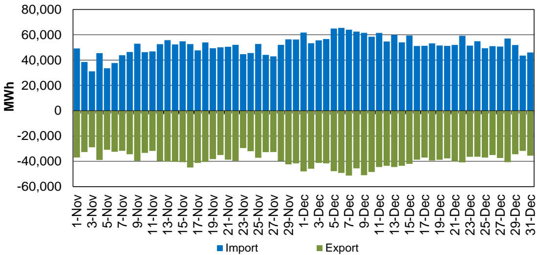
Figure 154: EIM Transfer for IPCO in FMM
