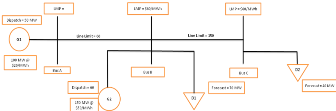
Figure 171: Real-Time Market Example 1.
