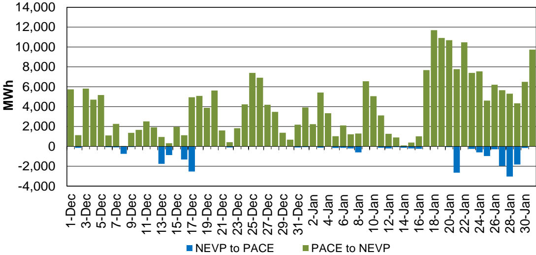
Figure 147: EIM Transfer between PACE and NEVP in FMM
