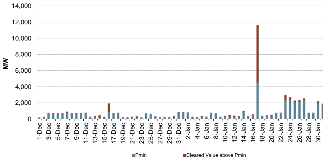
Figure 125: MOC Unit Commitment and Dispatch
