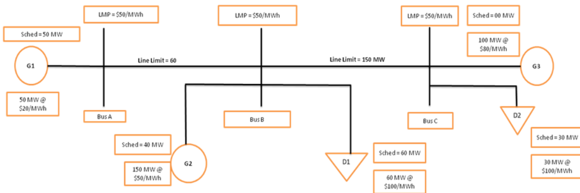
Figure 163: Day-Ahead Market for Example 2
