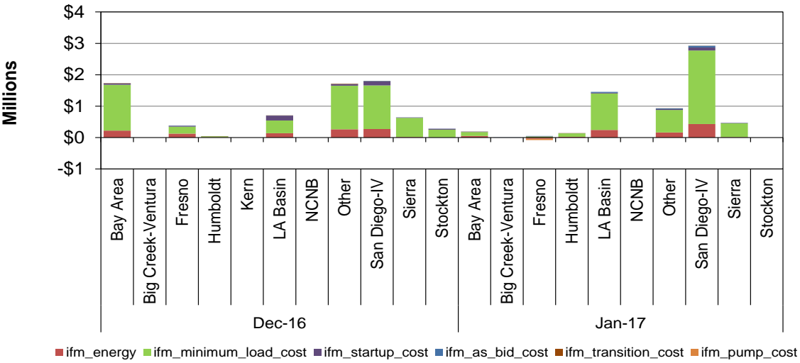
Figure 119: Monthly Cost in IFM by LCR
