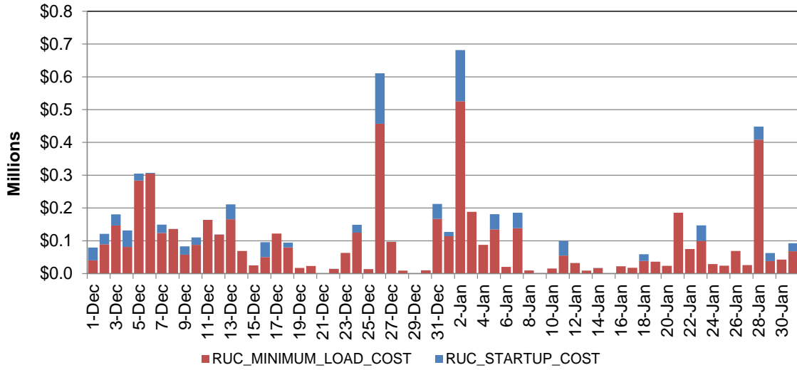
Figure 107: Cost in RUC
