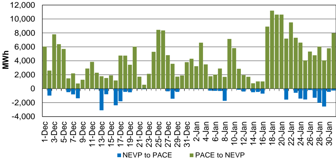
Figure 154: EIM Transfer between PACE and NEVP in RTD
