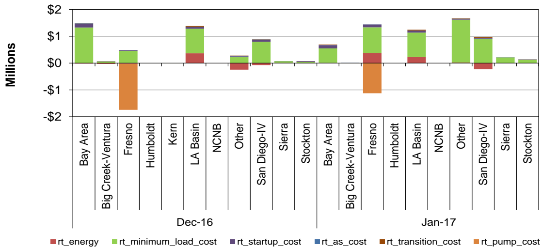
Figure 114: Monthly Cost in RT by LCR
