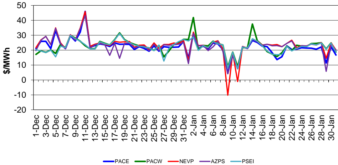
Figure 140: EIM Simple Average LAP Prices (Off-Peak Hours) in RTD
