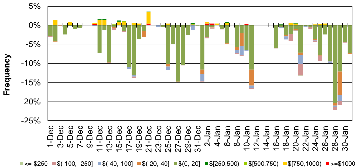
Figure 143: Daily Frequency of EIM LAP Positive Price Spikes and Negative Prices in RTD
