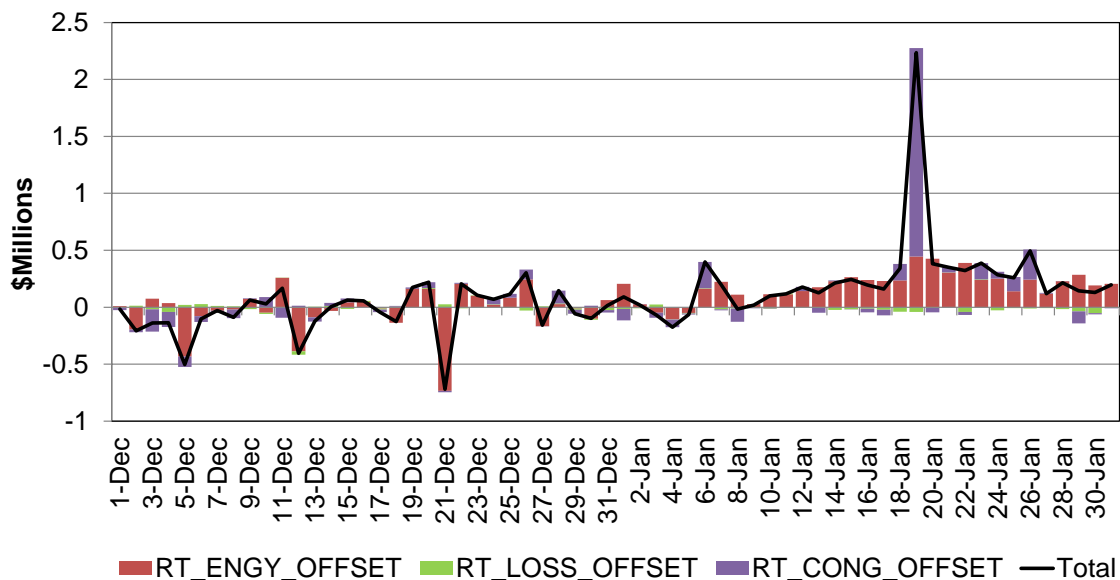
Figure 99: Daily Real-Time Offset Allocation
