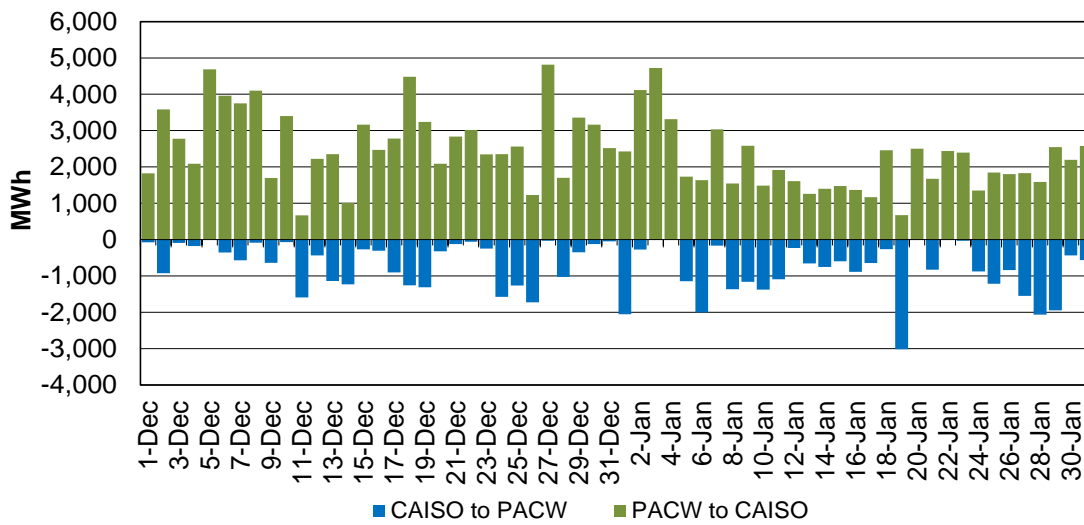
Figure 144: EIM Transfer between CAISO and PAC in FMM
