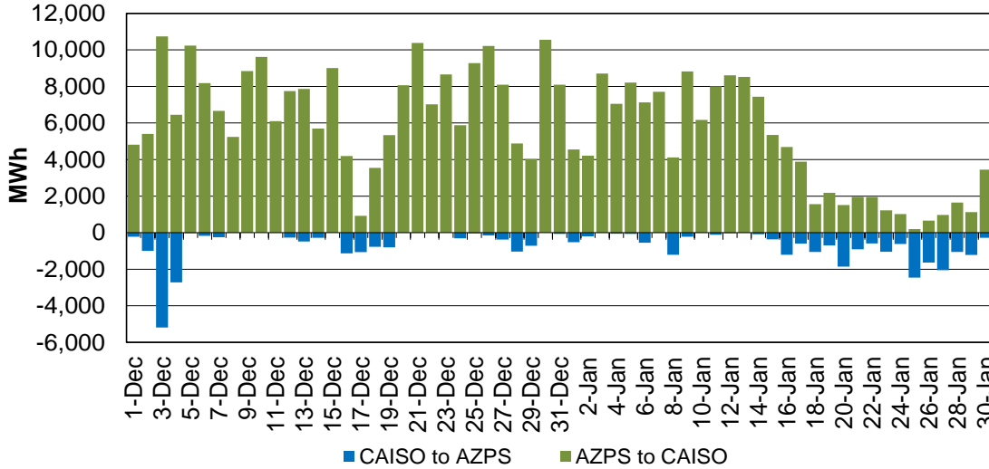
Figure 155: EIM Transfer between CAISO and AZPS in RTD
