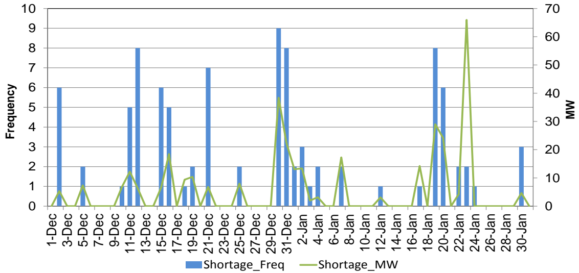
Figure 123: Frequency and Average MW of Shortage
