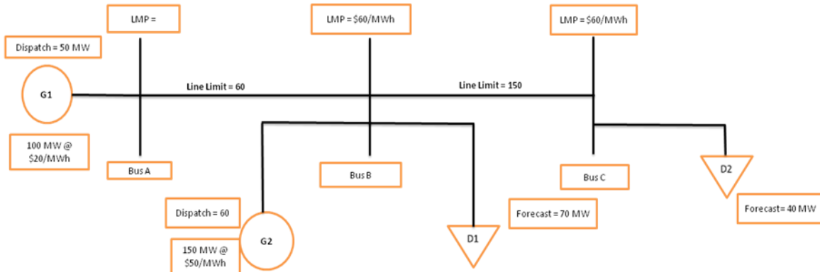
Figure 162: Real-Time Market Example 1.
