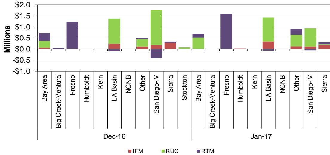
Figure 104: Monthly Bid Cost Recovery Allocation by LCR
