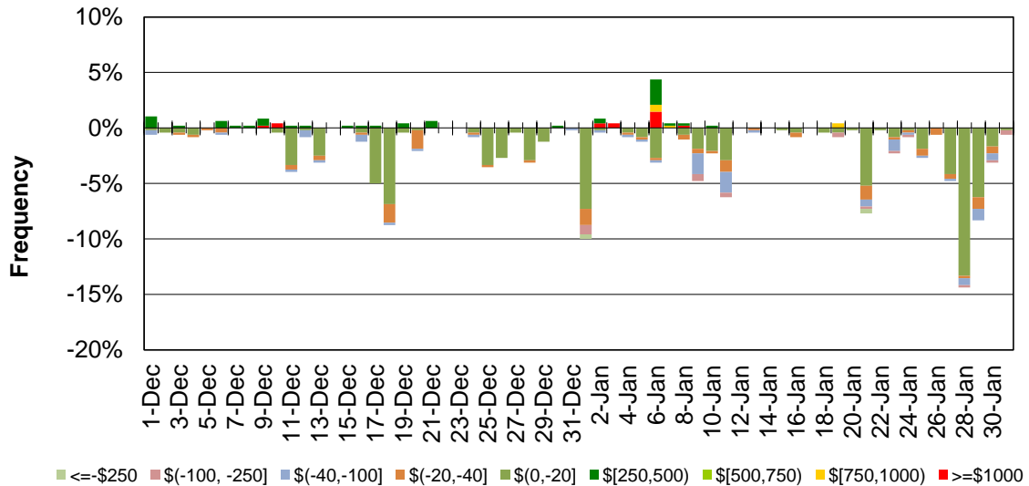
Figure 142: Daily Frequency of EIM LAP Positive Price Spikes and Negative Prices in FMM
