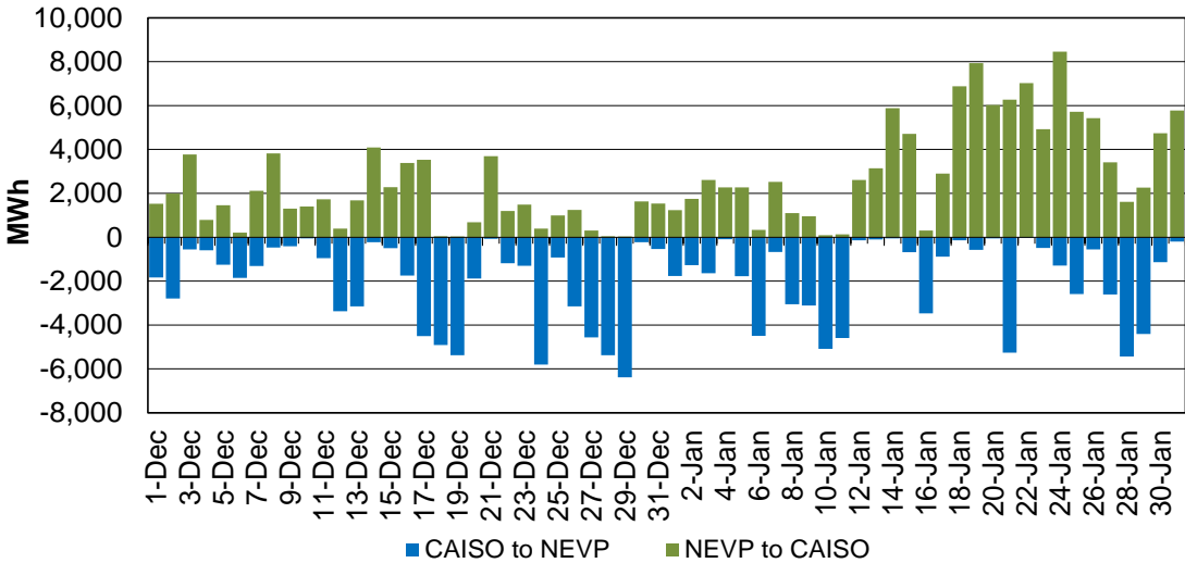
Figure 146: EIM Transfer between CAISO and NEVP in FMM
