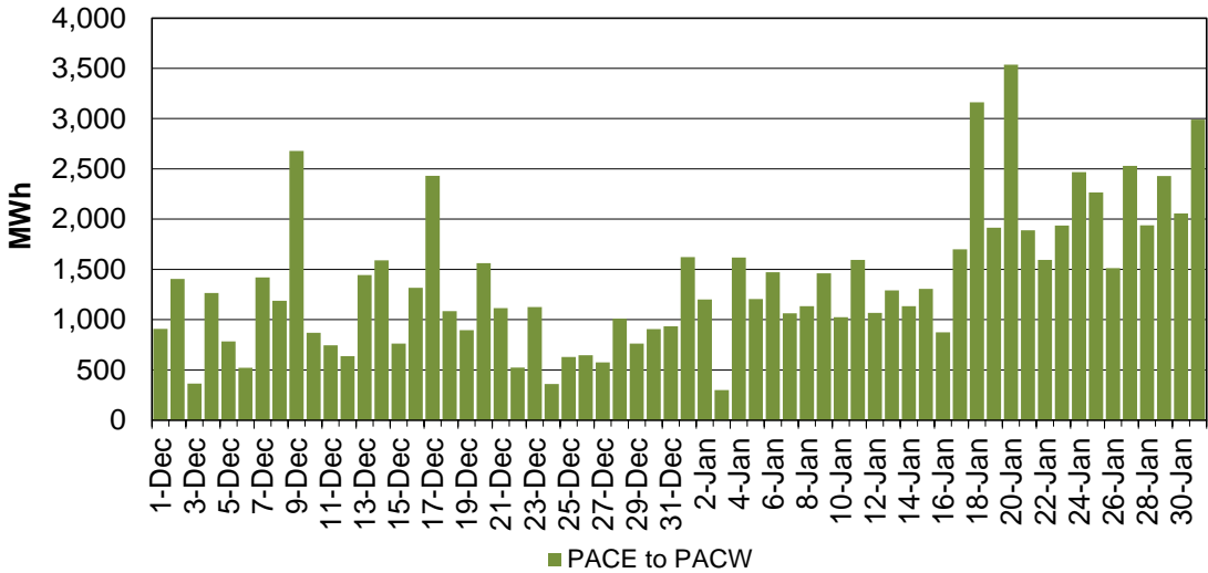
Figure 152: EIM Transfer between PACE and PACW in RTD
