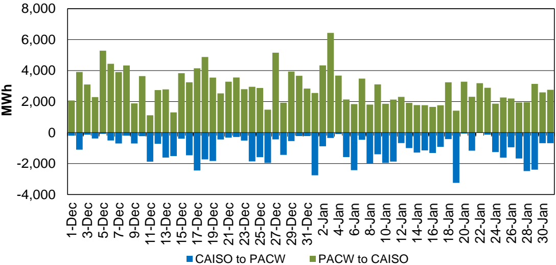
Figure 151: EIM Transfer between CAISO and PAC in RTD
