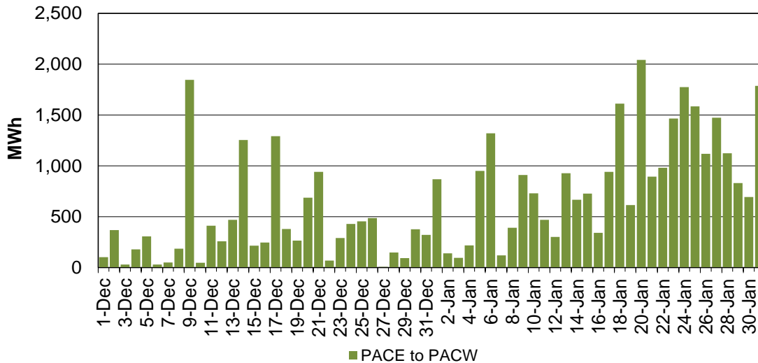
Figure 145: EIM Transfer between PACE and PACW in FMM
