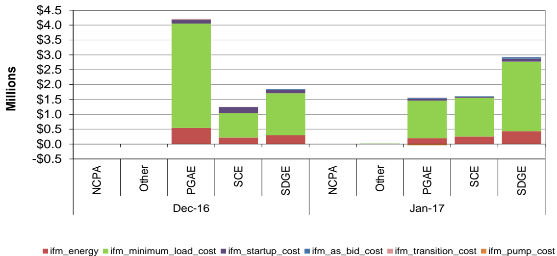
Figure 121: Monthly Cost in IFM by UDC
