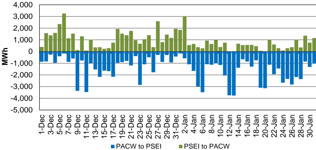
Figure 150: EIM Transfer between PACW and PSEI in FMM
