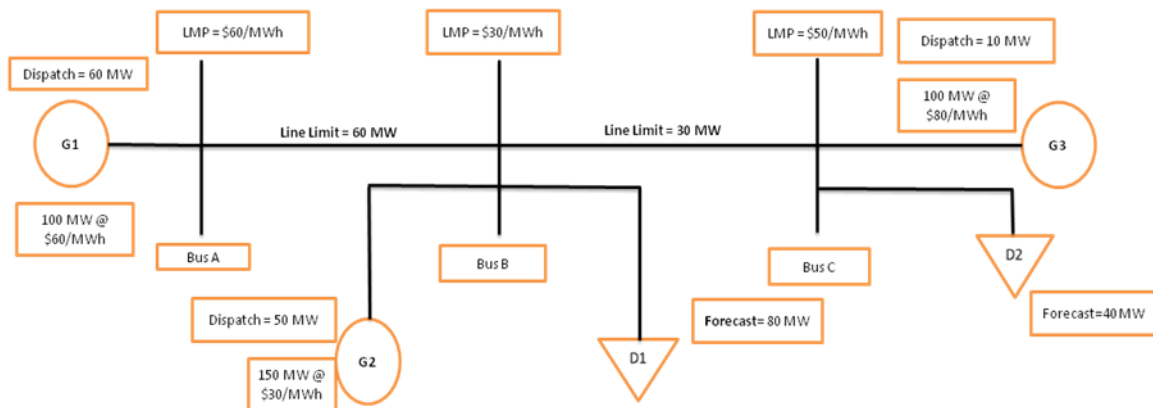
Figure 164: Summary of Real-Time Market Dispatch for Example 2
