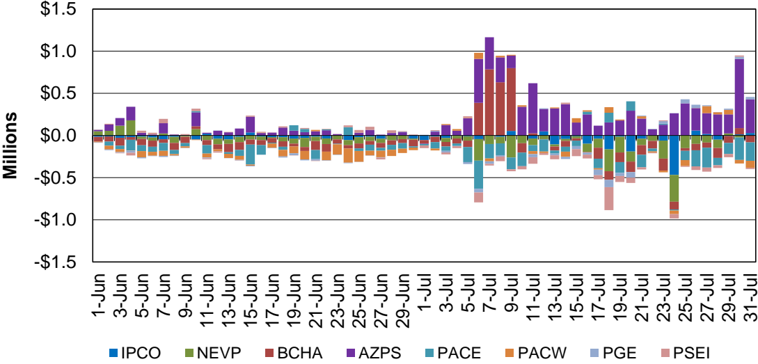
Figure 164: EIM Real-Time Imbalance Energy Offset by Area
