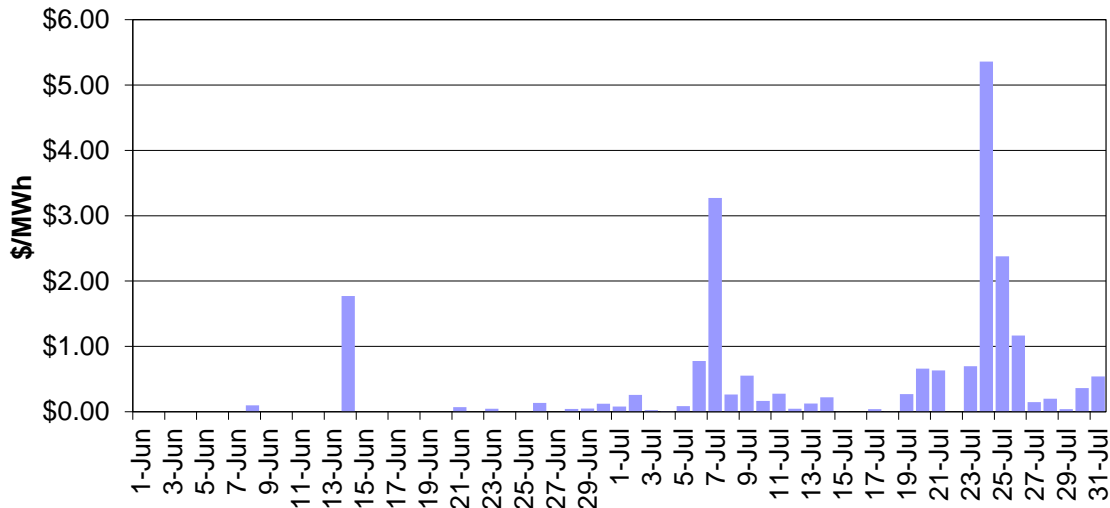
Figure 83: Average RUC Price
