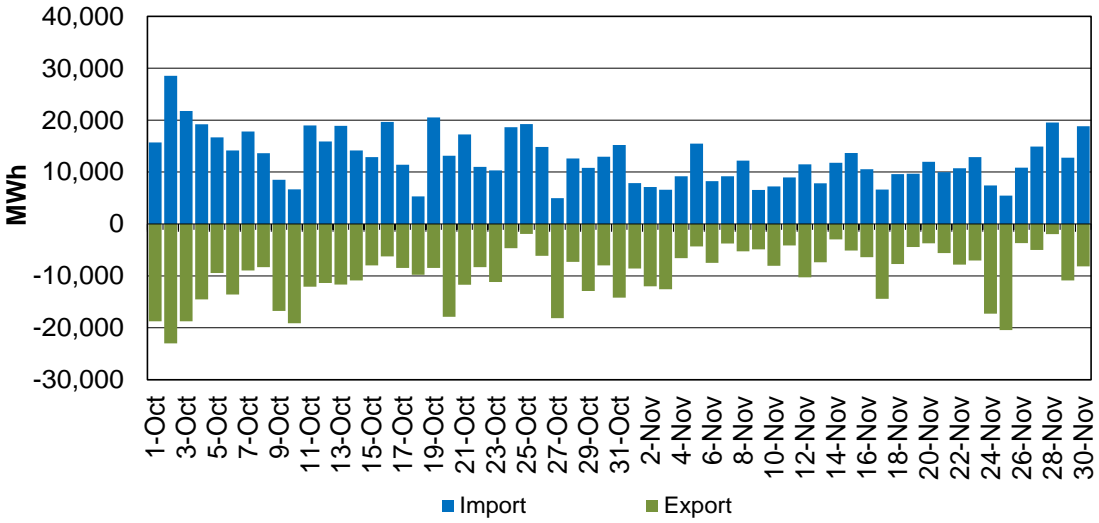
Figure 159: EIM Transfer for CAISO in RTD
