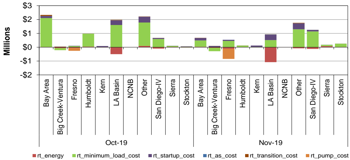
Figure 119: Monthly Cost in RT by LCR
