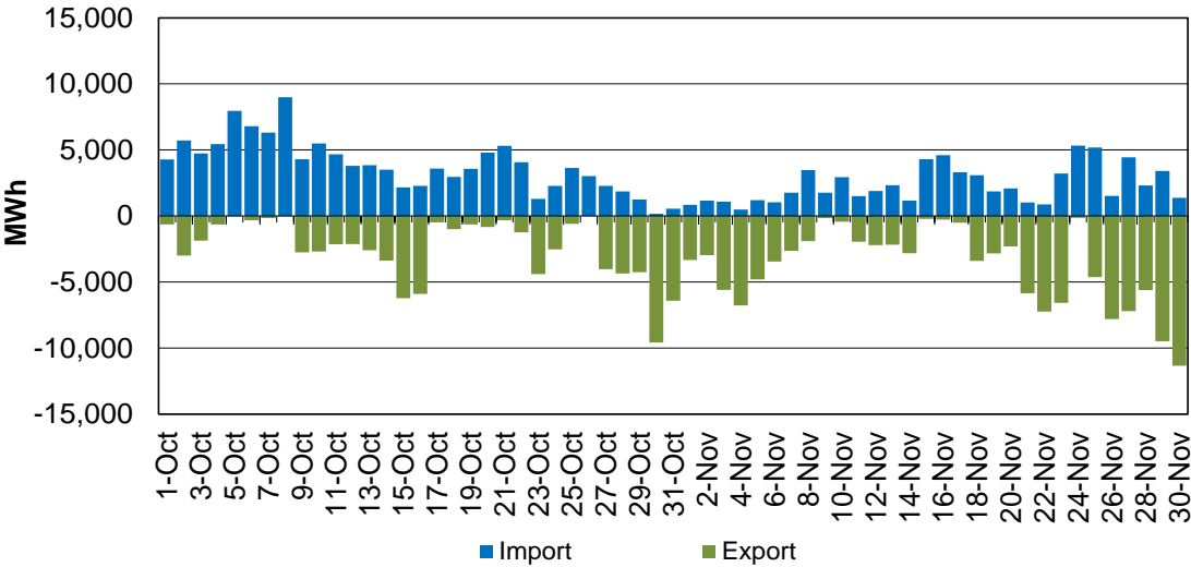
Figure 166: EIM Transfer for BCHA in RTD
