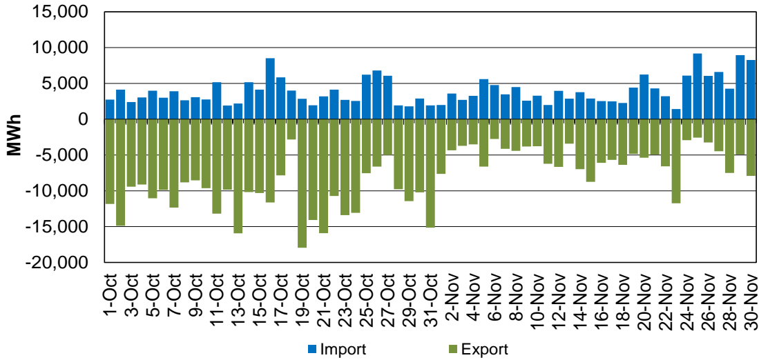
Figure 163: EIM Transfer for AZPS in RTD
