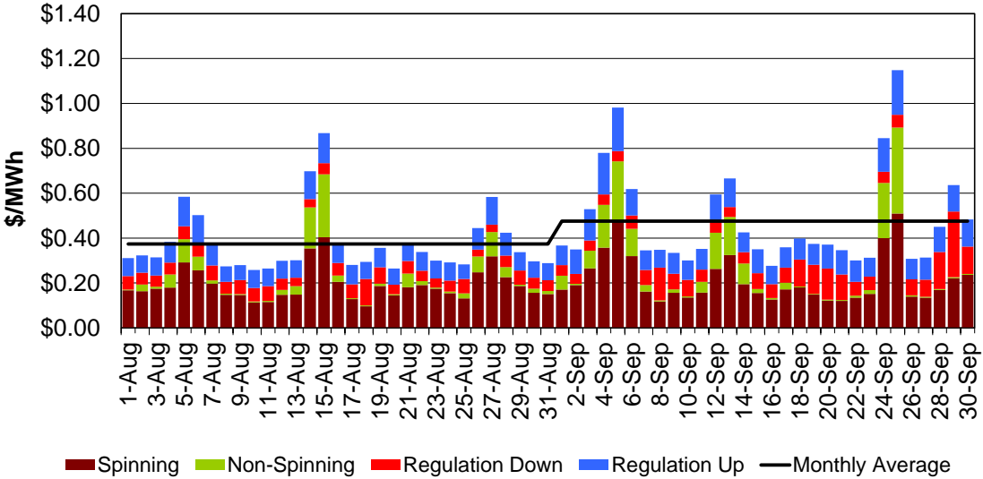
Figure 76: IFM (Day-Ahead) Average Cost to Load
