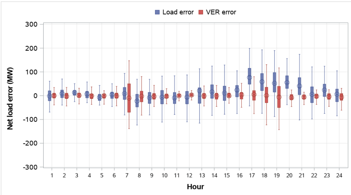
Figure 8.50 Seattle City Light average uncertainty by component (weekdays, May 2022)
