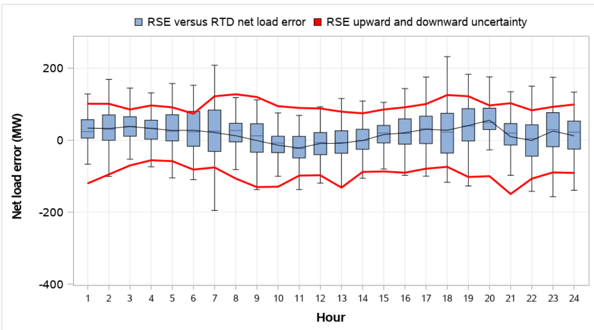
Figure 8.42 PNM distribution of RSE and RTD net load error and comparison to RSE uncertainty (weekdays, May 2022)
