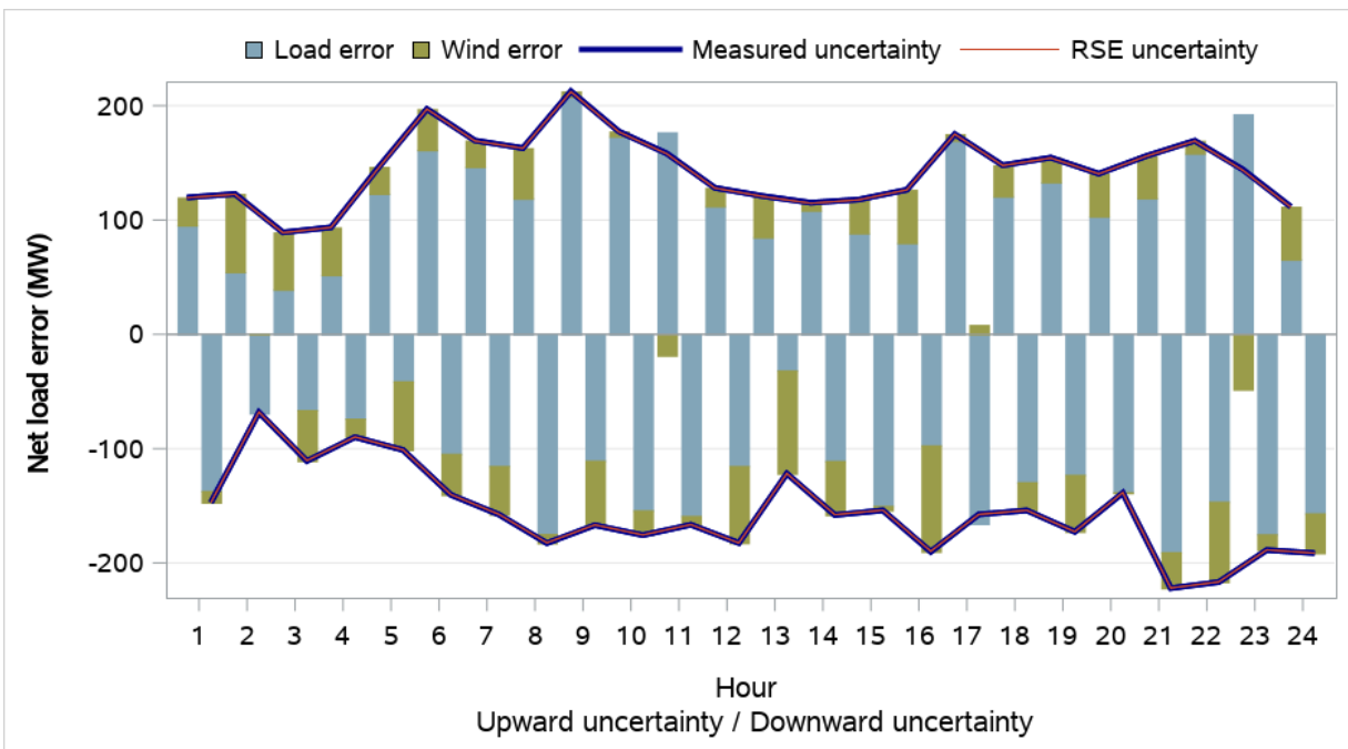
Figure 8.38 Powerex average uncertainty by component (weekdays, May 2022)
