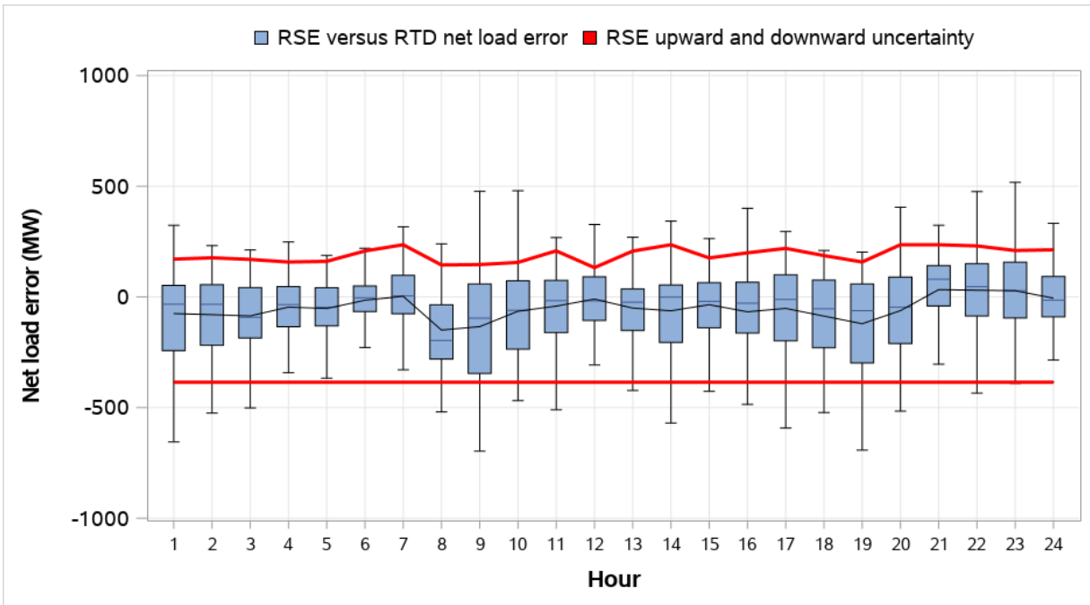
Figure 8.16 BPA distribution of RSE and RTD load and VER error (weekdays, May 2022)
