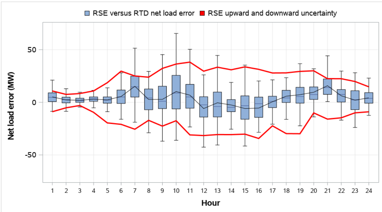
Figure 8.52 Seattle City Light distribution of RSE and RTD load and VER error (weekdays, May 2022)
