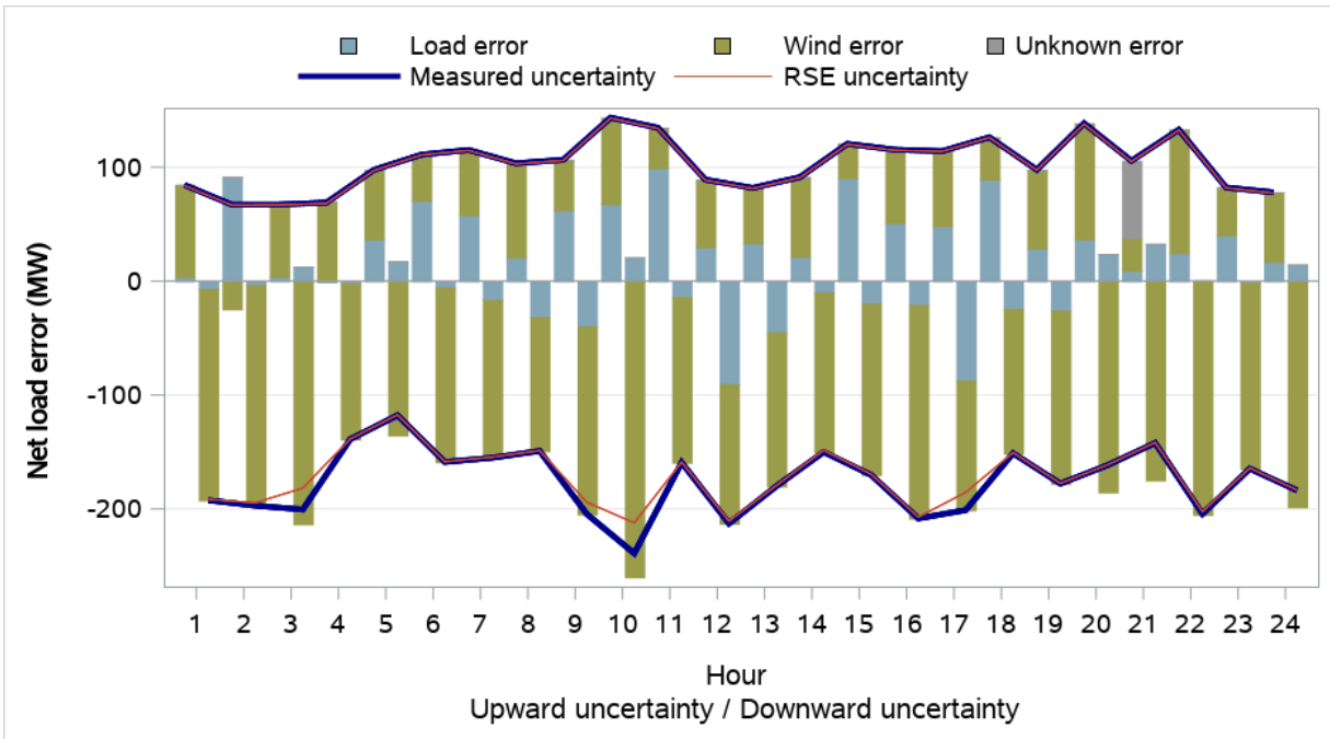
Figure 8.36 Portland General Electric distribution of RSE and RTD net load error and comparison to RSE uncertainty (weekdays, May 2022)
