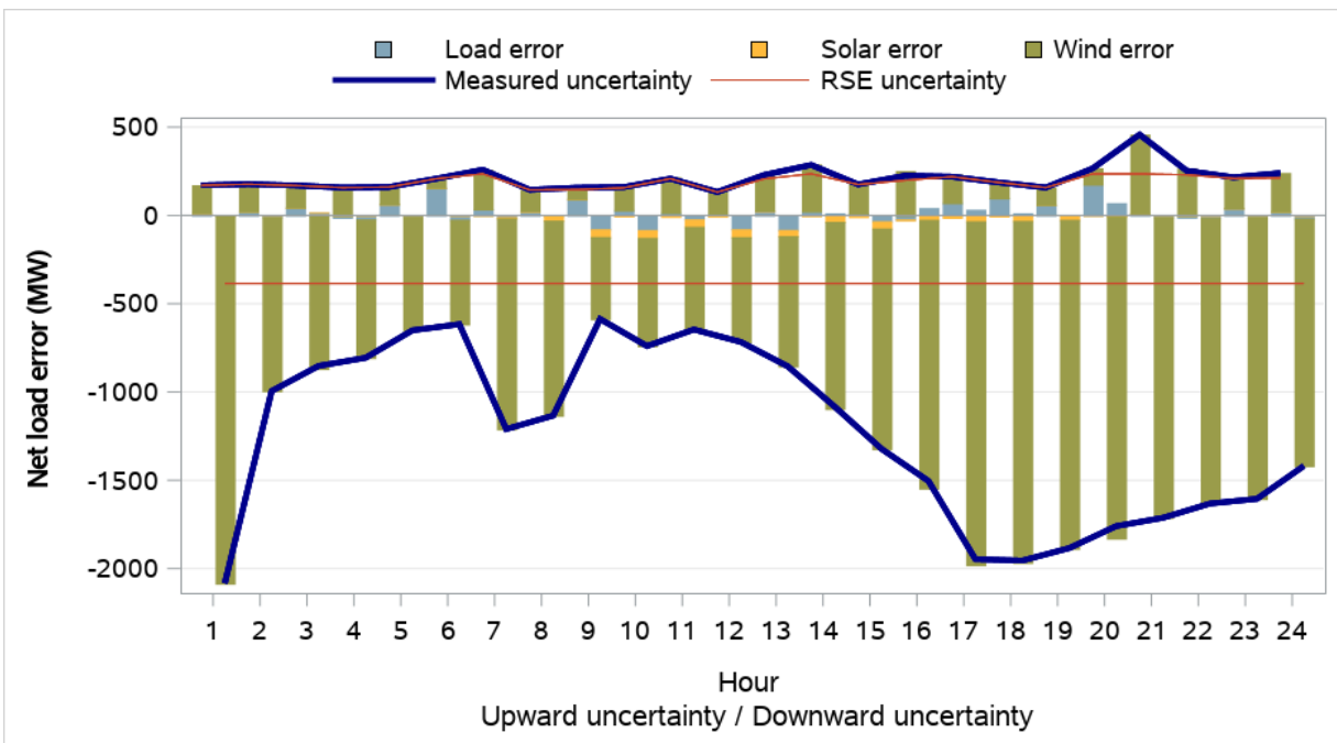
Figure 8.14 BPA average uncertainty by component (weekdays, May 2022)
