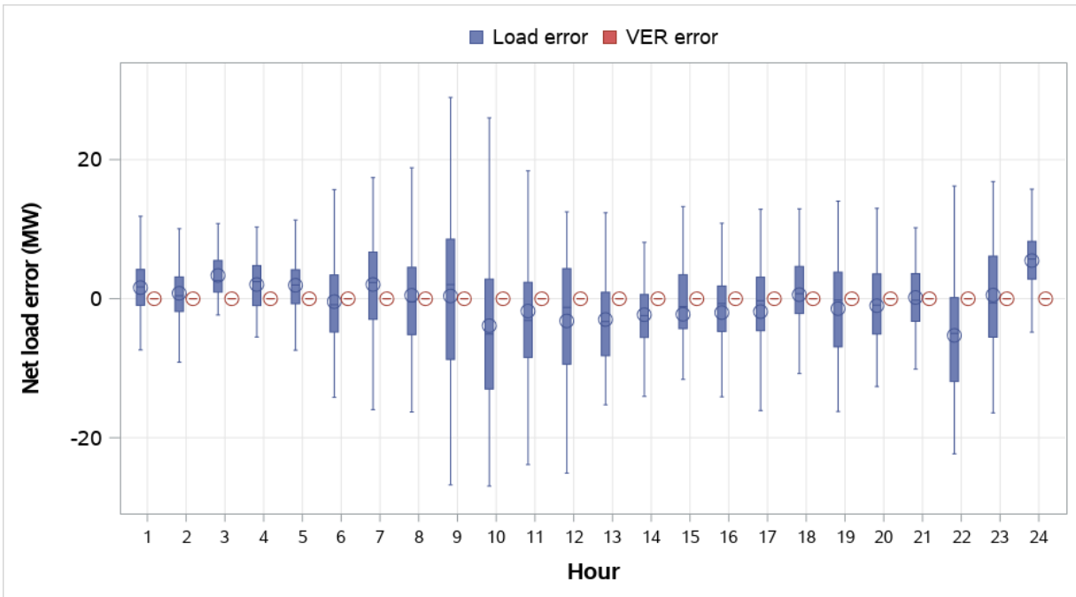
Figure 8.56 Tucson Electric Power average uncertainty by component (weekdays, May 2022)
