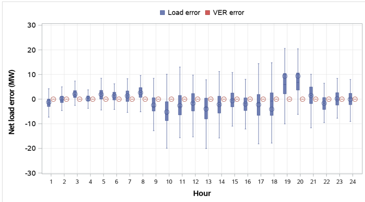
Figure 8.61 Turlock Irrigation District distribution of RSE and RTD load and VER error (weekdays, May 2022)
