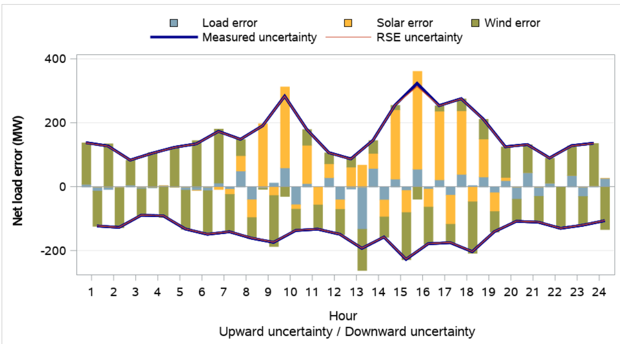
Figure 8.20 LADWP average uncertainty by component (weekdays, May 2022)
