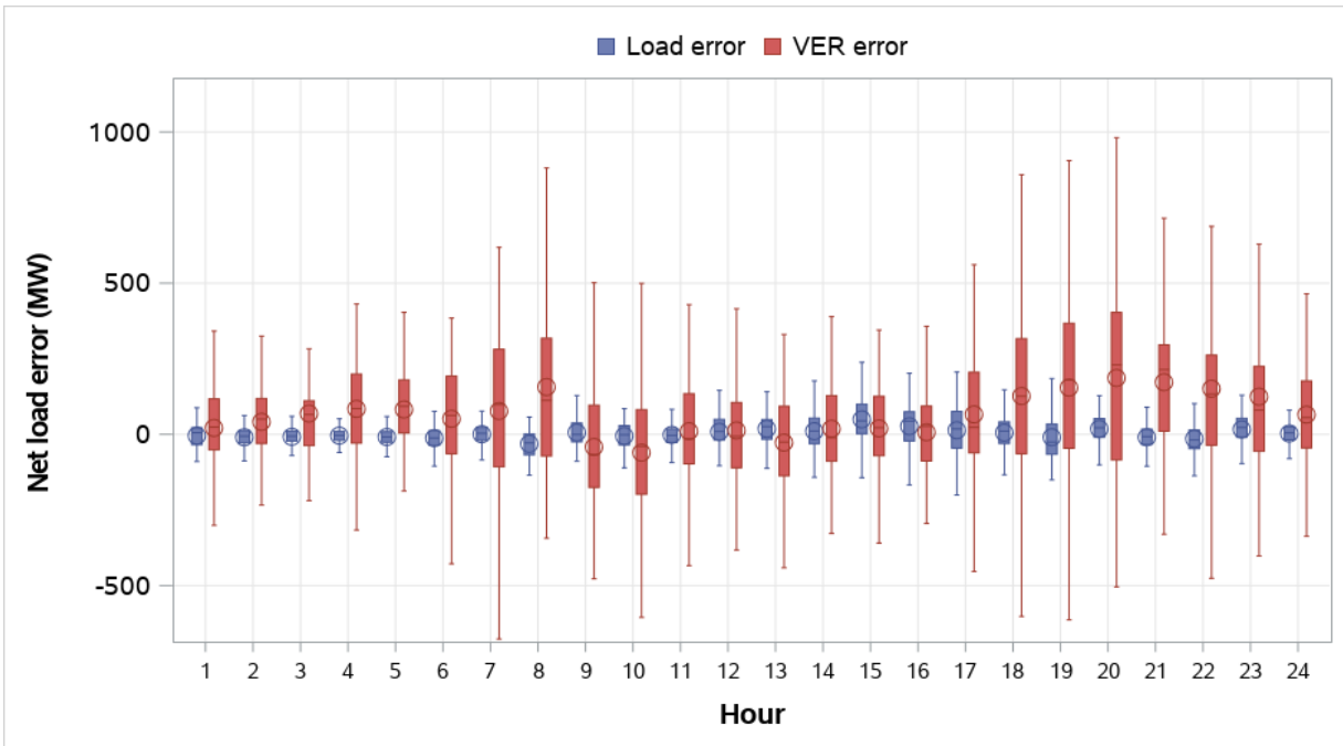
Figure 8.32 PacifiCorp West average uncertainty by component (weekdays, May 2022)
