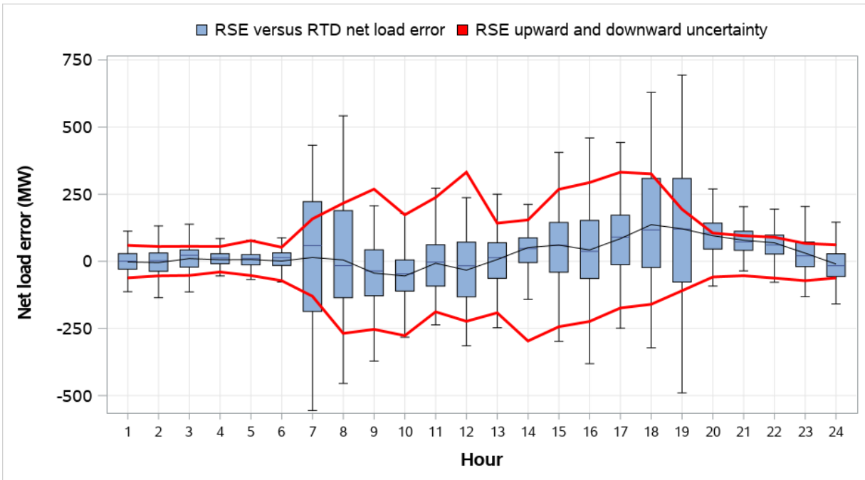
Figure 8.28 NV Energy distribution of RSE and RTD load and VER error (weekdays, May 2022)
