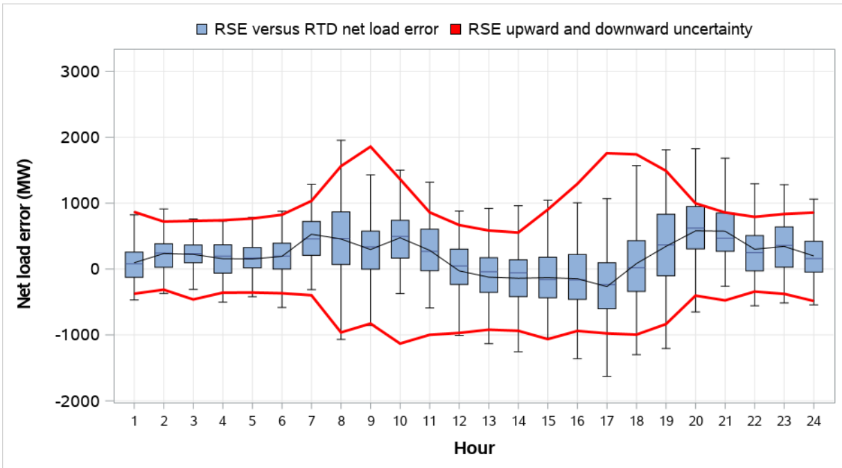
Figure 8.4 CAISO distribution of RSE and RTD load and VER error (weekdays, May 2022)
