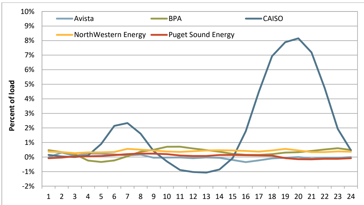
Figure 5.4 Average hourly 15-minute market imbalance conformance as a percent of load (May 2022)
