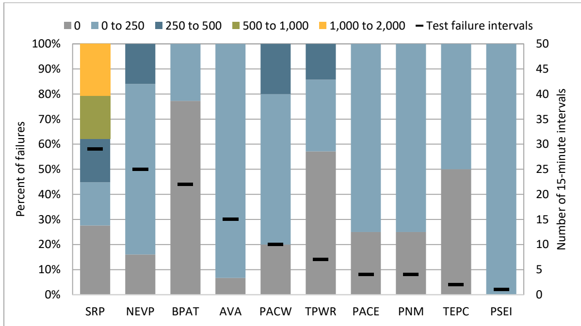
Figure 4.2 Upward capacity/flexibility test failure intervals by incremental import limit (May 2022)
