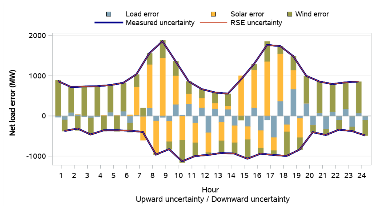
Figure 8.2 CAISO average uncertainty by component (weekdays, May 2022)
