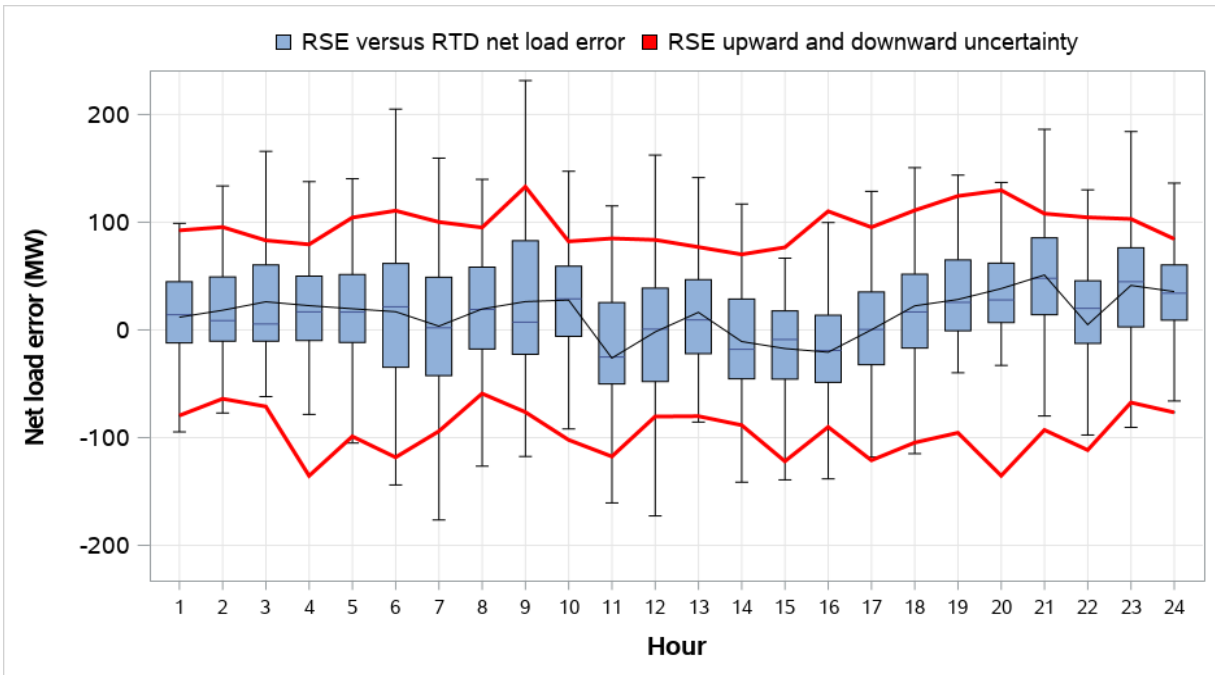
Figure 8.46 Puget Sound Energy distribution of RSE and RTD load and VER error (weekdays, May 2022)
