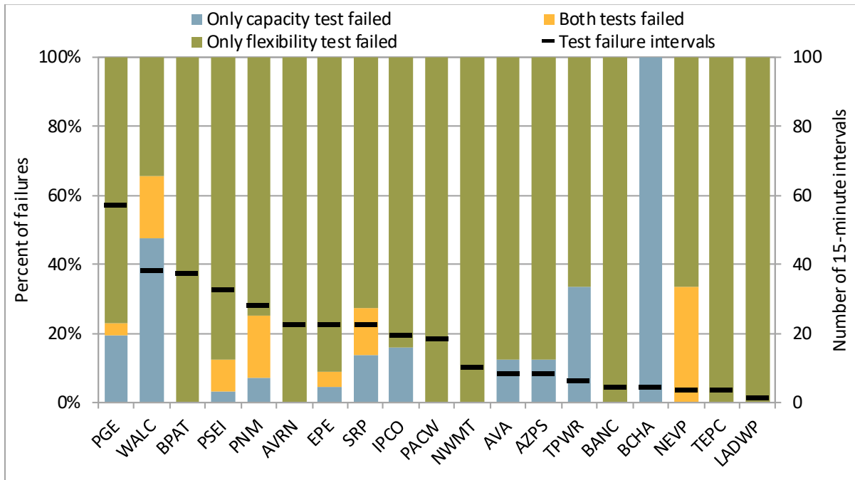
Figure 3.9 Upward capacity/flexibility test failure intervals by concurrence (May 2023)
