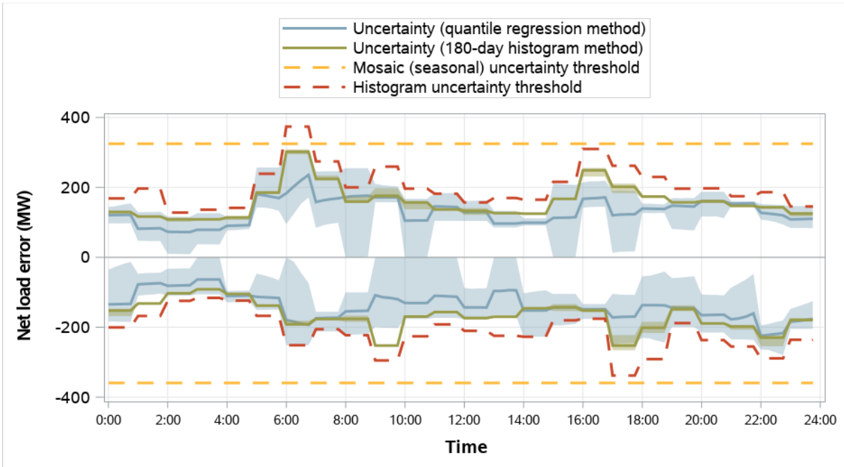
Figure 4.33 Powerex distribution of RSE and RTD net load error and comparison to RSE uncertainty (weekdays, May 2023)
