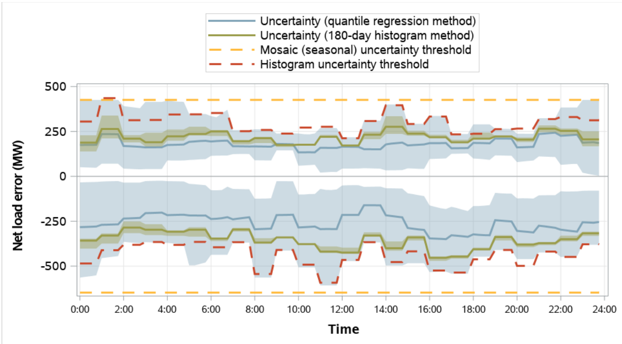
Figure 4.15 BPA distribution of RSE and RTD net load error and comparison to RSE uncertainty (weekdays, May 2023)
