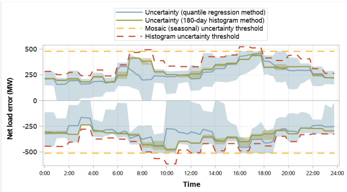
Figure 4.27 PacifiCorp East distribution of RSE and RTD net load error and comparison to RSE uncertainty (weekdays, May 2023)
