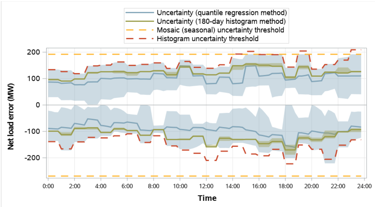
Figure 4.31 Portland General Electric distribution of RSE and RTD net load error and comparison to RSE uncertainty (weekdays, May 2023)
