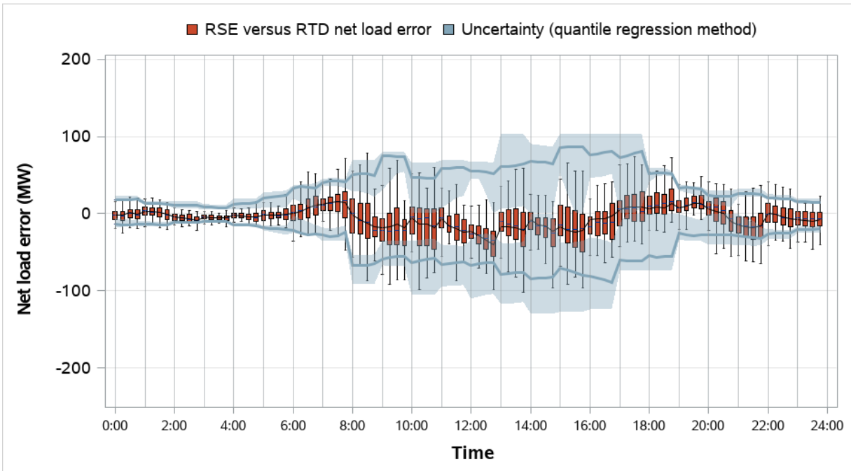
Figure 4.13 BANC distribution of RSE and RTD net load error and comparison to RSE uncertainty (weekdays, May 2023)
