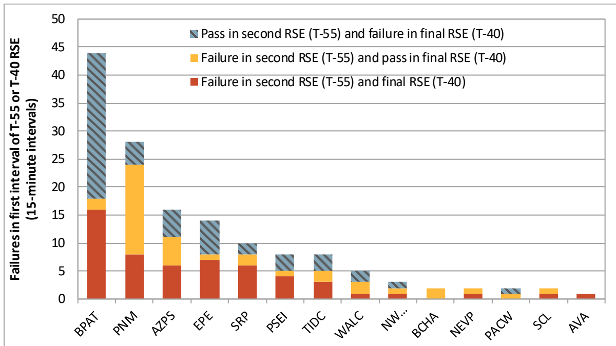
Figure 3.12 Downward resource sufficiency evaluation failures in first 15-minute interval of hour (May 2023)
