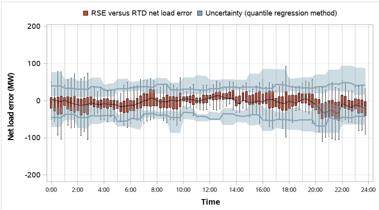
Figure 4.11 Avista distribution of RSE and RTD net load error and comparison to RSE uncertainty (weekdays, May 2023)
