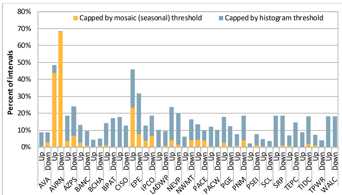
Figure 4.1 Quantile regression uncertainty capped by mosaic or histogram thresholds (May 2023)
