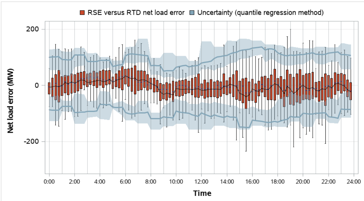
Figure 4.35 PNM distribution of RSE and RTD net load error and comparison to RSE uncertainty (weekdays, May 2023)
