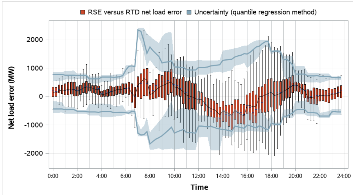
Figure 4.5 CAISO distribution of RSE and RTD net load error and comparison to RSE uncertainty (weekdays, May 2023)
