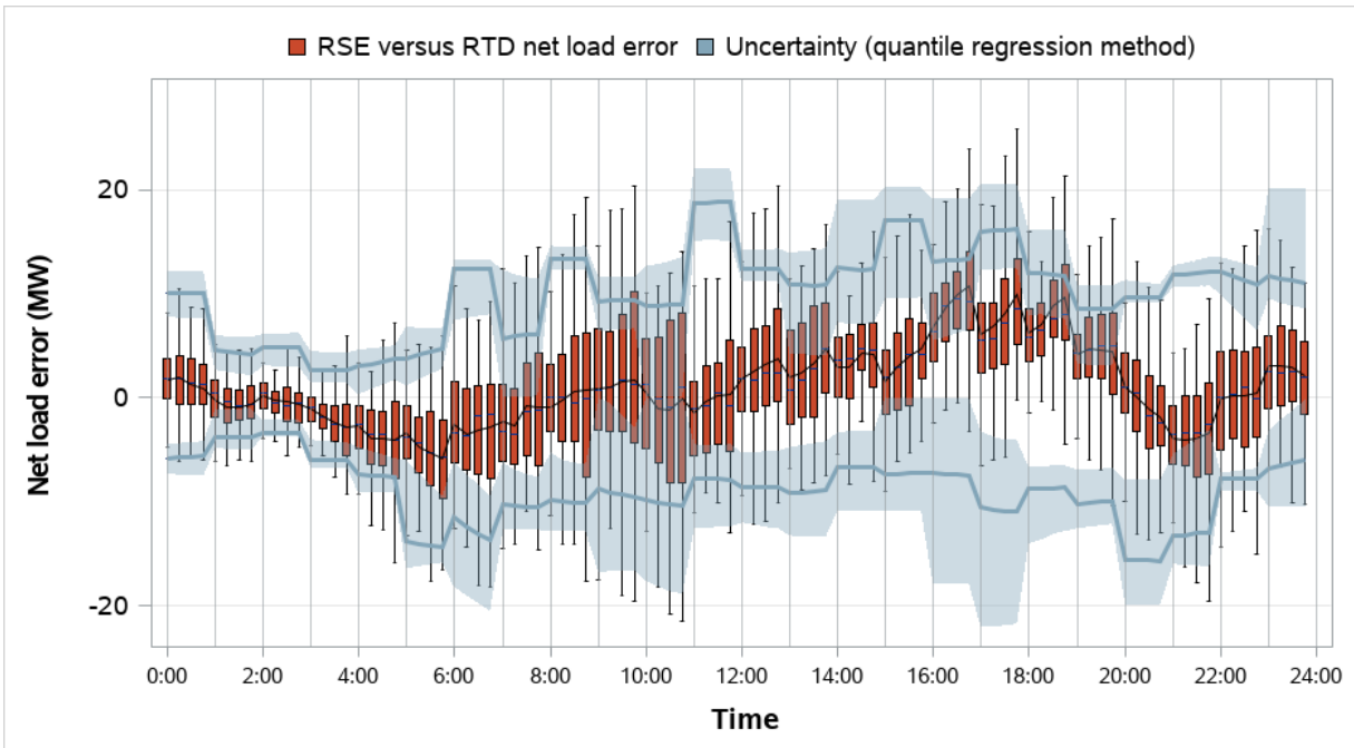
Figure 4.43 Tacoma Power distribution of RSE and RTD net load error and comparison to RSE uncertainty (weekdays, May 2023)
