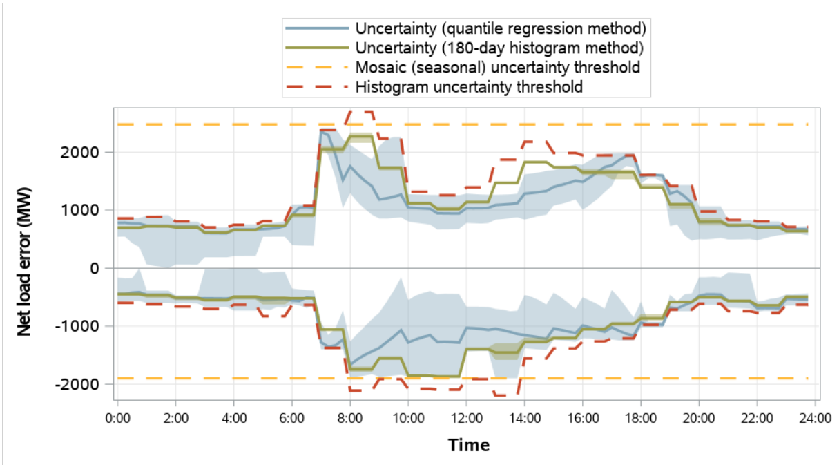
Figure 4.4 CAISO resource sufficiency evaluation uncertainty requirements (weekdays, May 2023)
