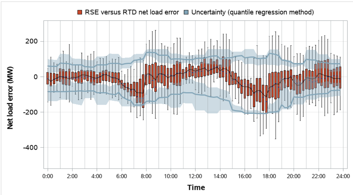
Figure 4.19 Idaho Power distribution of RSE and RTD net load error and comparison to RSE uncertainty (weekdays, May 2023)
