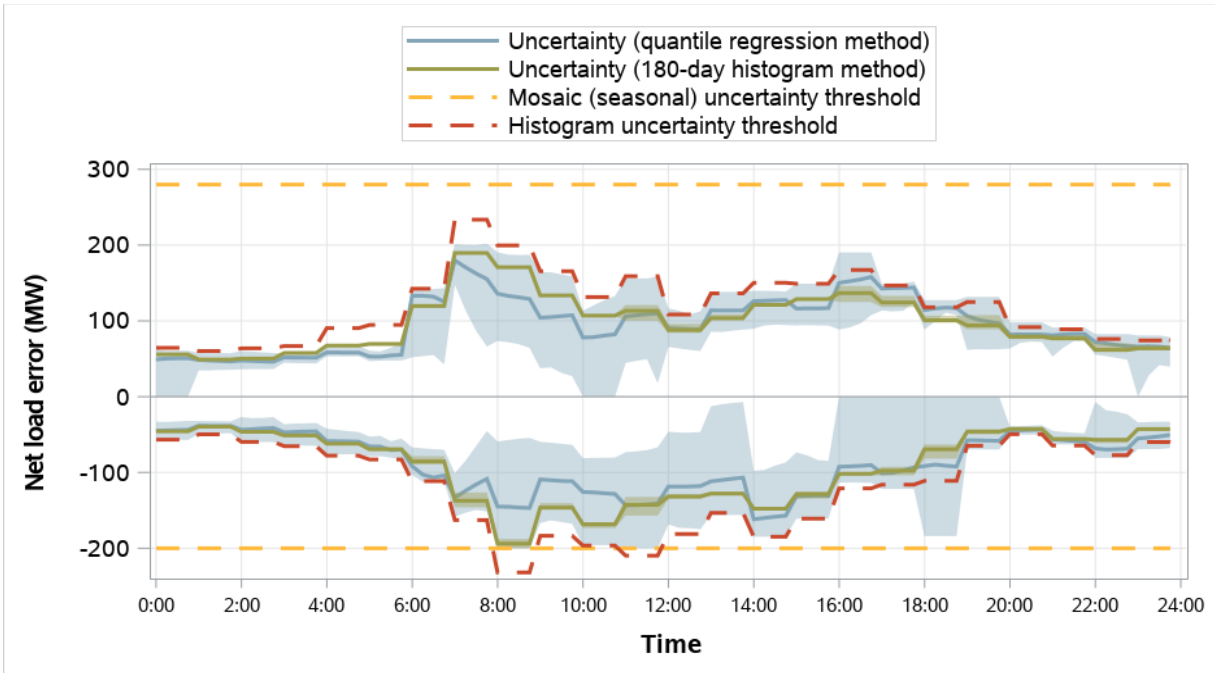
Figure 4.39 Salt River Project distribution of RSE and RTD net load error and comparison to RSE uncertainty (weekdays, May 2023)
