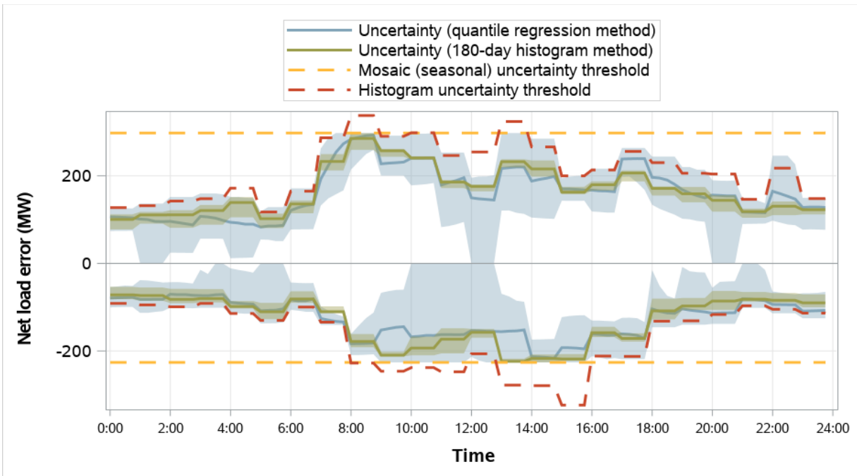
Figure 4.7 Arizona Public Service distribution of RSE and RTD net load error and comparison to RSE uncertainty (weekdays, May 2023)
