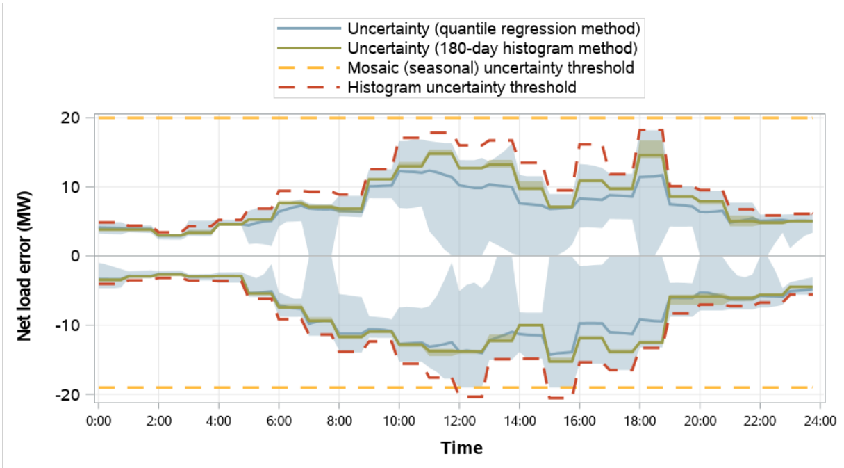
Figure 4.47 Turlock Irrigation District distribution of RSE and RTD net load error and comparison to RSE uncertainty (weekdays, May 2023)
