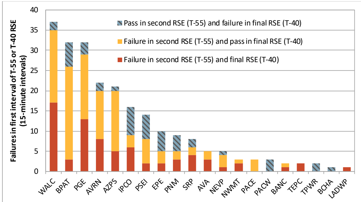
Figure 3.11 Upward resource sufficiency evaluation failures in first 15-minute interval of hour (May 2023)
