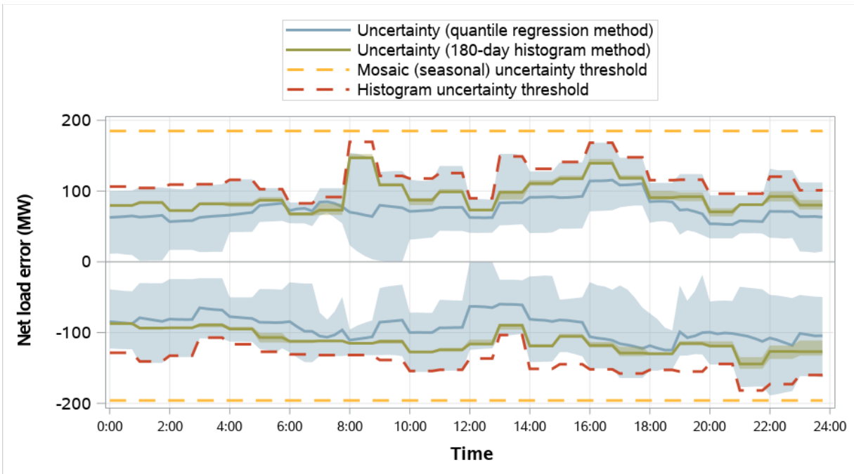
Figure 4.29 PacifiCorp West distribution of RSE and RTD net load error and comparison to RSE uncertainty (weekdays, May 2023)
