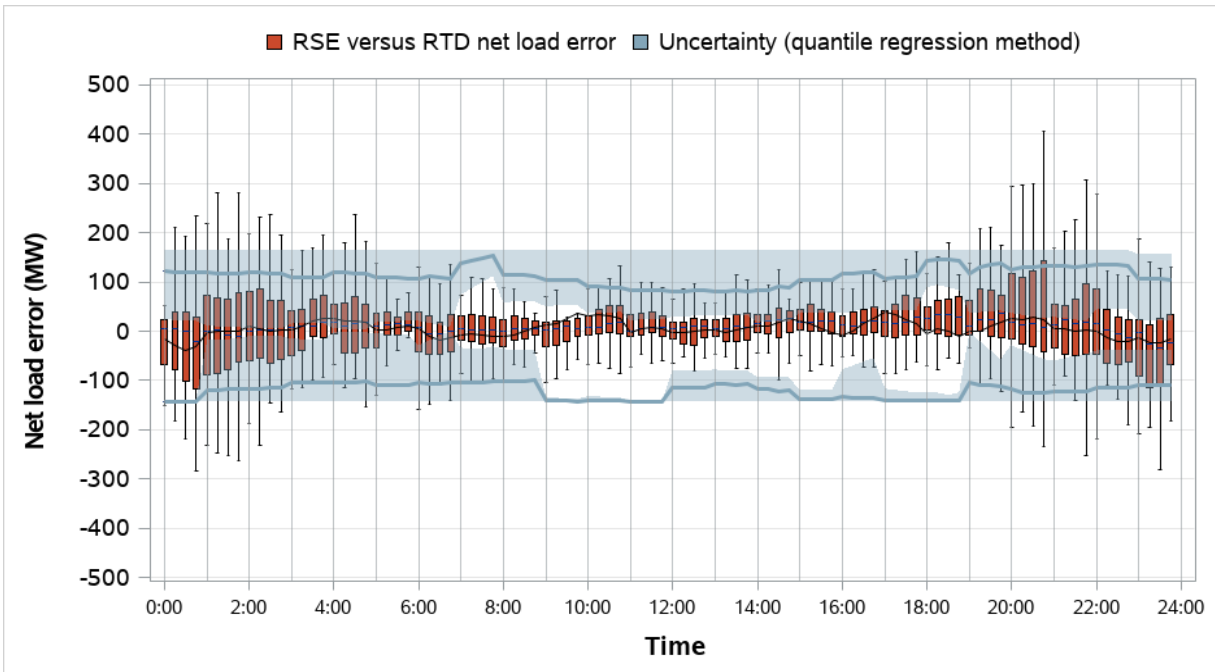
Figure 4.9 Avangrid distribution of RSE and RTD net load error and comparison to RSE uncertainty (weekdays, May 2023)
