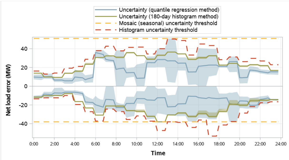
Figure 4.41 Seattle City Light distribution of RSE and RTD net load error and comparison to RSE uncertainty (weekdays, May 2023)
