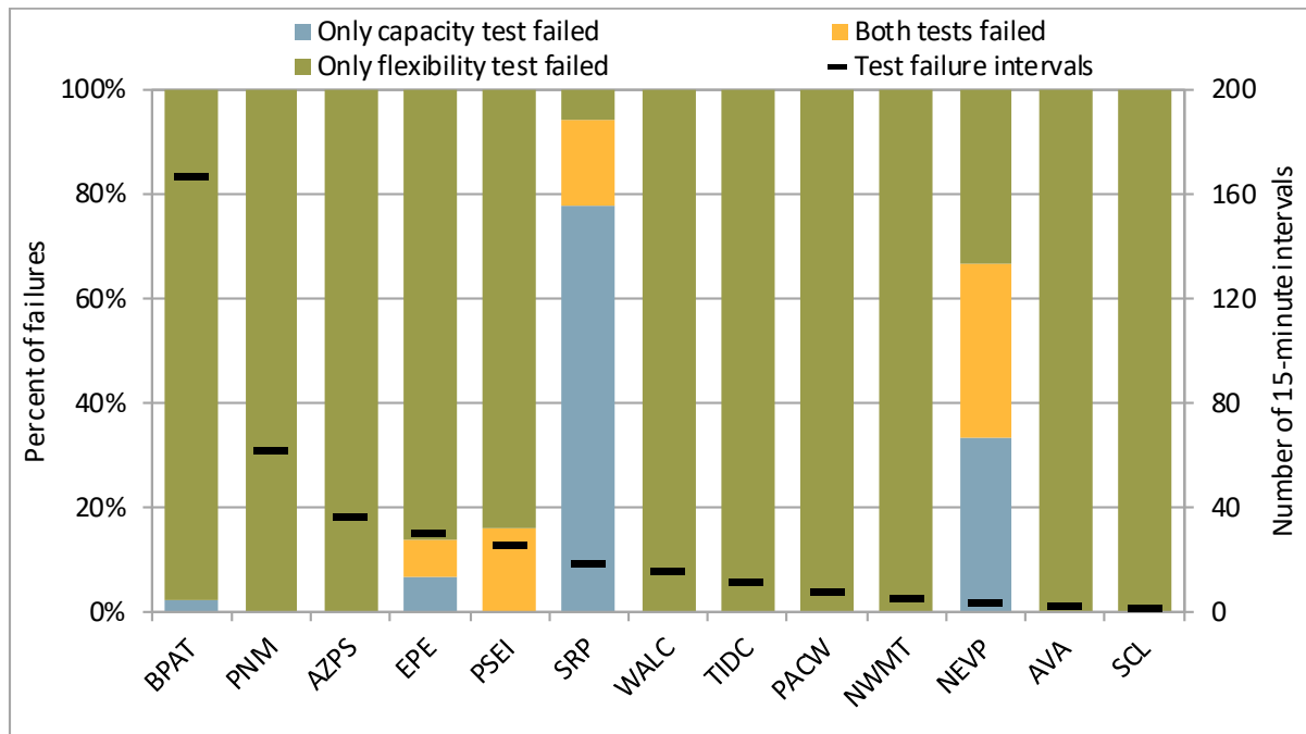
Figure 3.10 Downward capacity/flexibility test failure intervals by concurrence (May 2023)
