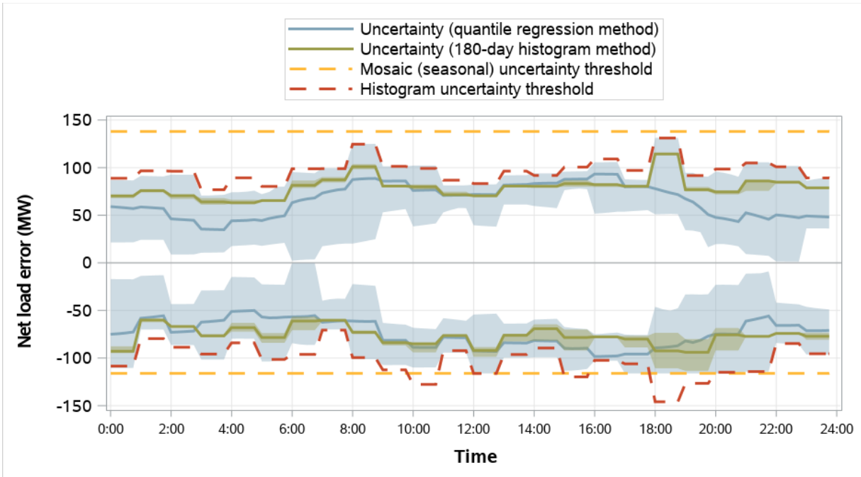
Figure 4.23 NorthWestern Energy distribution of RSE and RTD net load error and comparison to RSE uncertainty (weekdays, May 2023)
