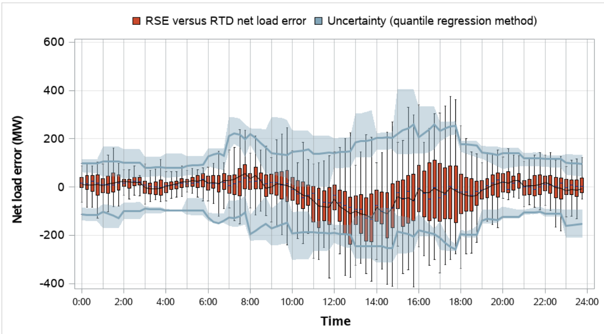
Figure 4.21 LADWP distribution of RSE and RTD net load error and comparison to RSE uncertainty (weekdays, May 2023)
