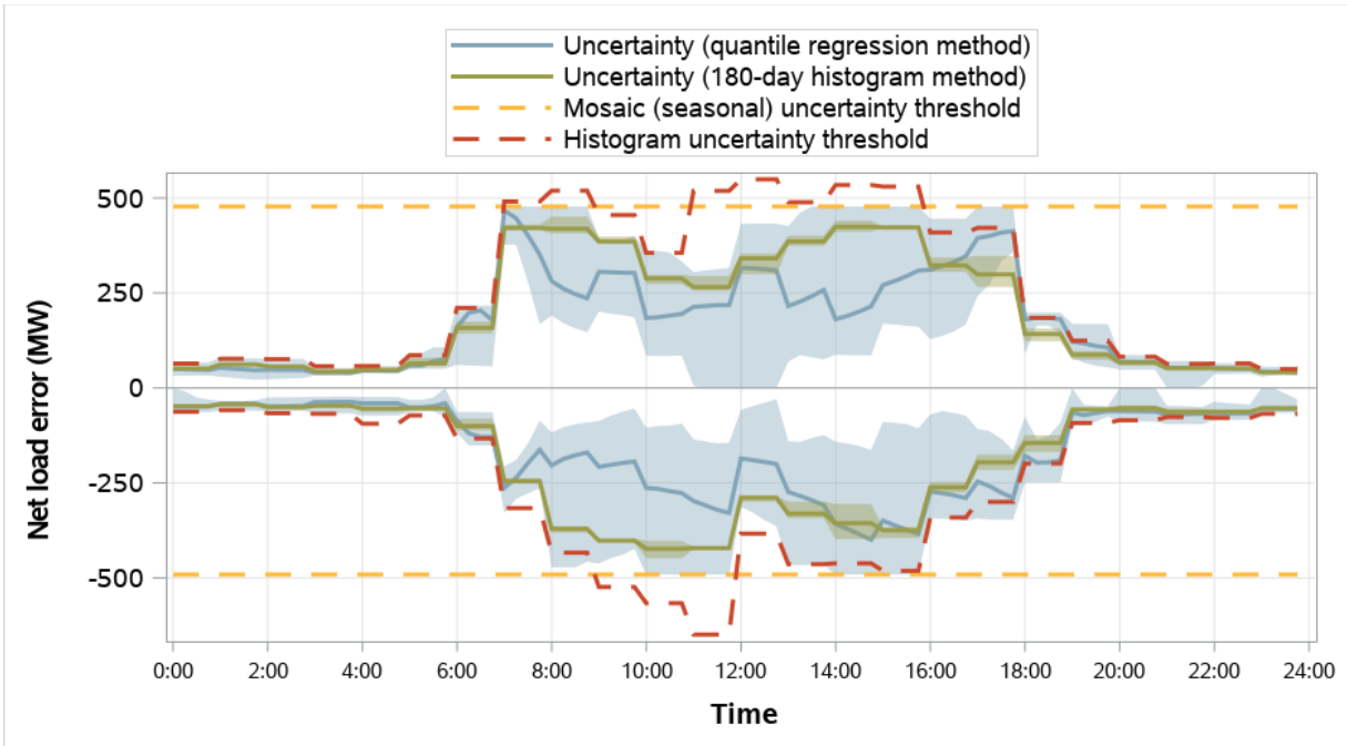
Figure 4.25 NV Energy distribution of RSE and RTD net load error and comparison to RSE uncertainty (weekdays, May 2023)
