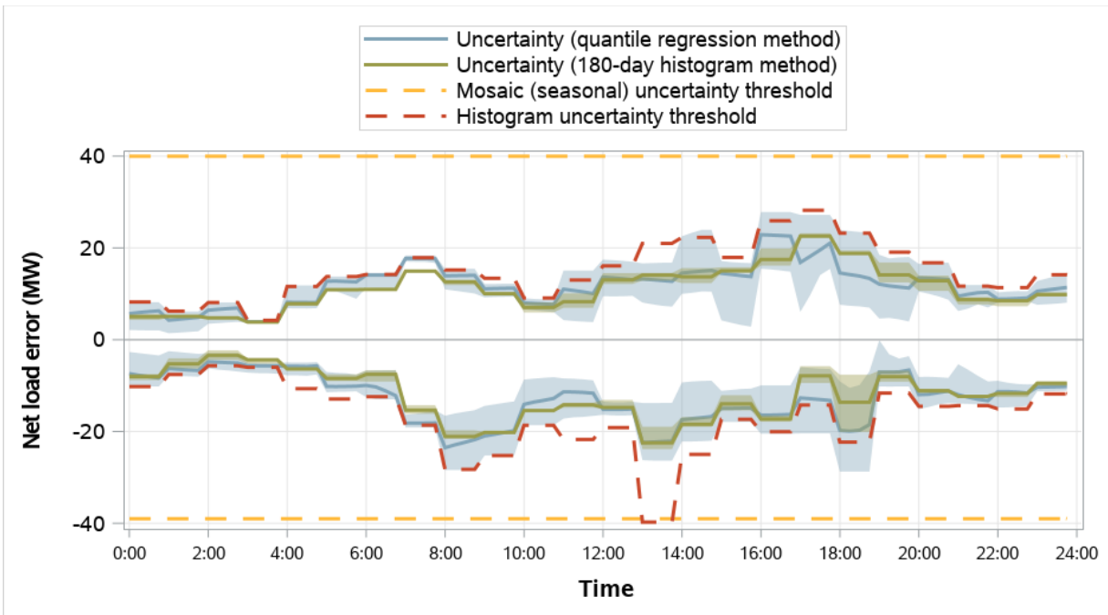
Figure 4.49 WAPA Desert Southwest distribution of RSE and RTD net load error and comparison to RSE uncertainty (weekdays, May 2023)
