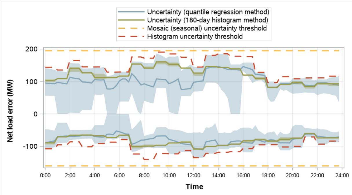
Figure 4.45 Tucson Electric Power distribution of RSE and RTD net load error and comparison to RSE uncertainty (weekdays, May 2023)
