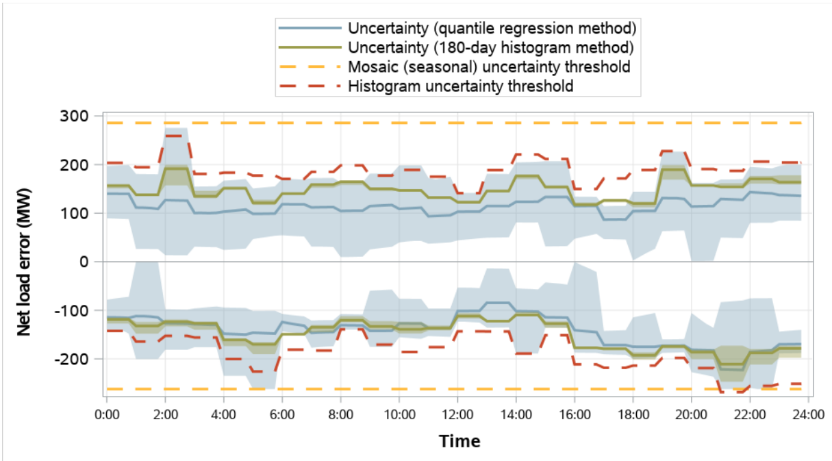
Figure 4.37 Puget Sound Energy distribution of RSE and RTD net load error and comparison to RSE uncertainty (weekdays, May 2023)
