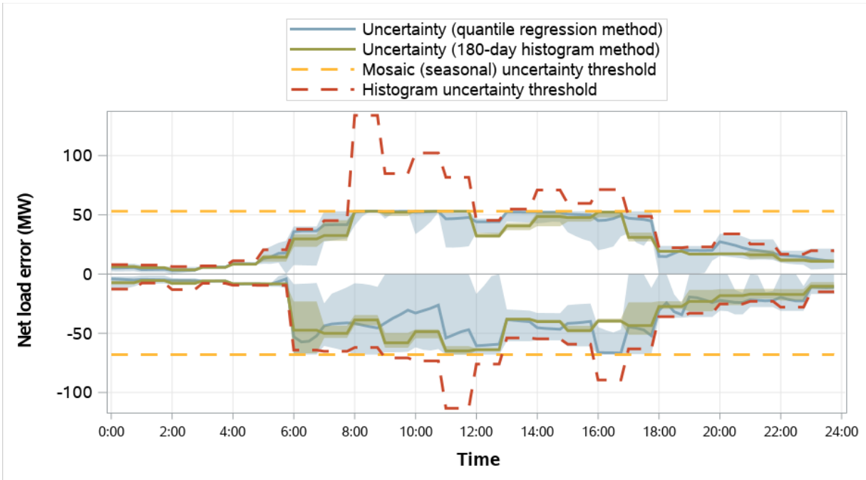
Figure 4.17 El Paso Electric distribution of RSE and RTD net load error and comparison to RSE uncertainty (weekdays, May 2023)
