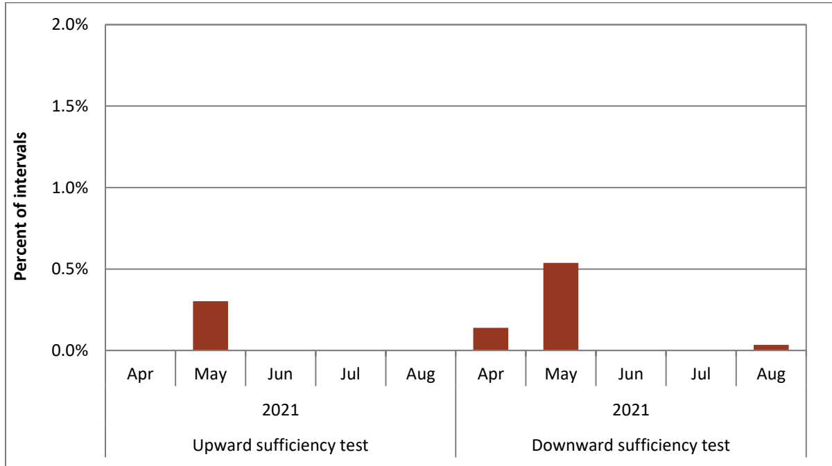
Figure 2.1 Frequency of upward and downward sufficiency test failures by month Turlock Irrigation District (TIDC)
