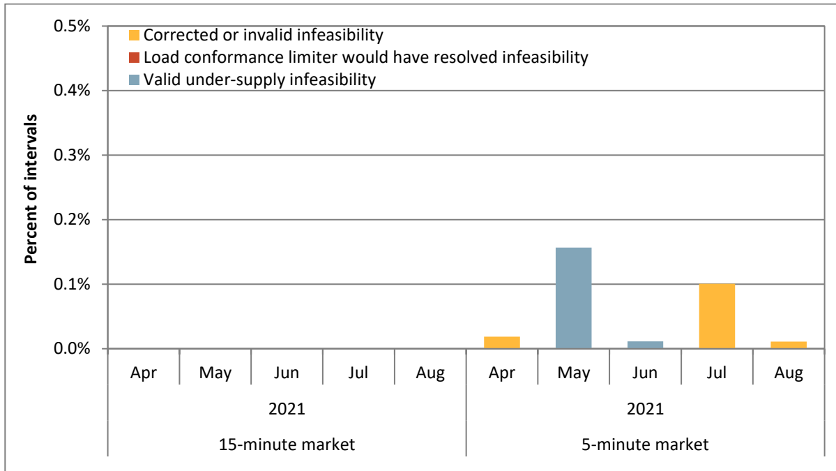
Figure 1.3 Frequency of under-supply power balance infeasibilities by month Turlock Irrigation District
