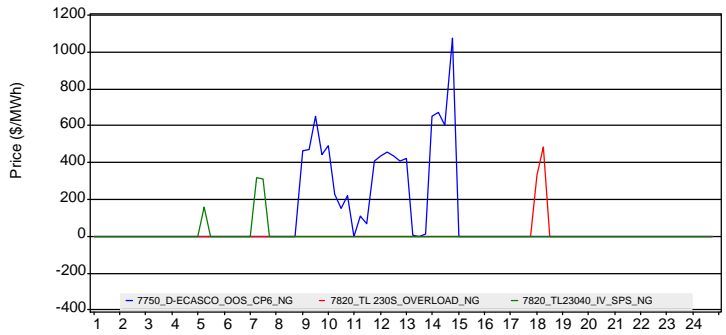
Selected FMM Transmission Line and Transformer Shadow Prices
