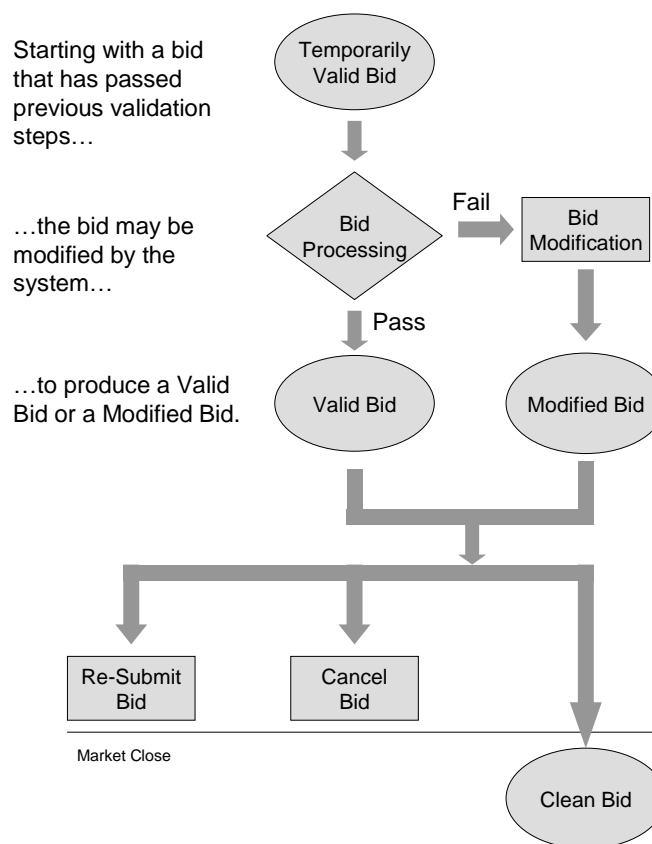
Figure 5: Day Ahead Processing (After Master File Update)
