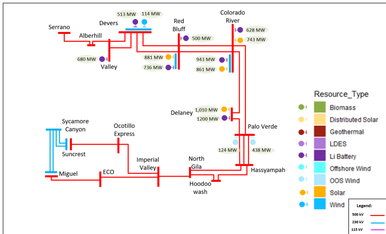
Figure F.14-1: SCE Eastern Interconnection Area – Mapped 35 Base Portfolio
