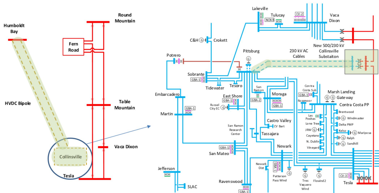
Figure F.16-3: LCC HVDC Option to Interconnect Humboldt Bay Offshore Wind (Option 3)
