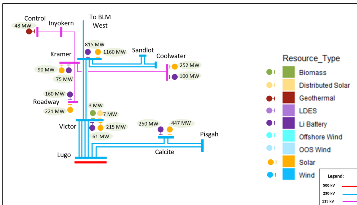
Figure F.12-1: SCE North of Lugo Interconnection Area – Mapped 25 Base Portfolio
