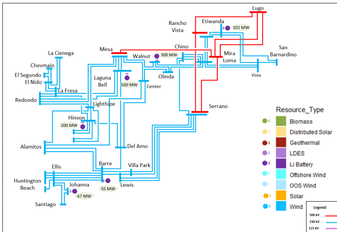
Figure F.13-1: SCE Metro Interconnection Area – Mapped 32 Base Portfolio
