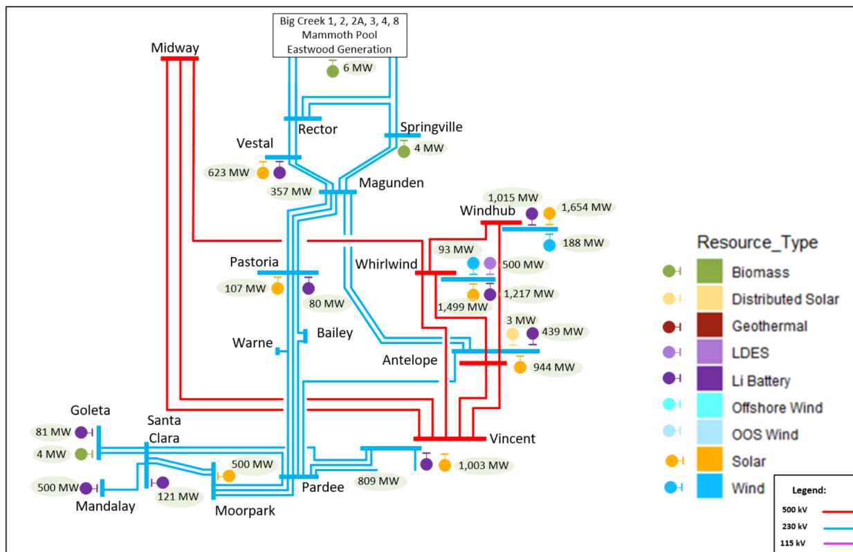
Figure F.11-1: SCE Northern Interconnection Area – Mapped 20 Base Portfolio
