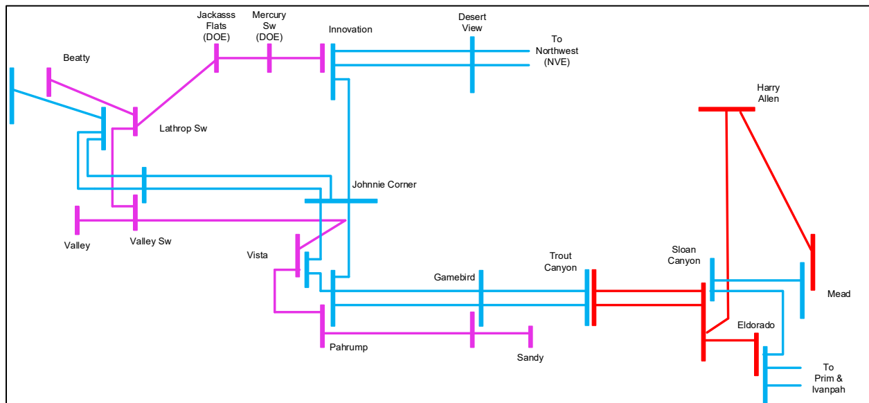
Figure F.10-2: GLW/VEA Transmission System with Recommended Re-scoping of the GLW/VEA Area Upgrades Project and the Beatty 230 kV Projected
