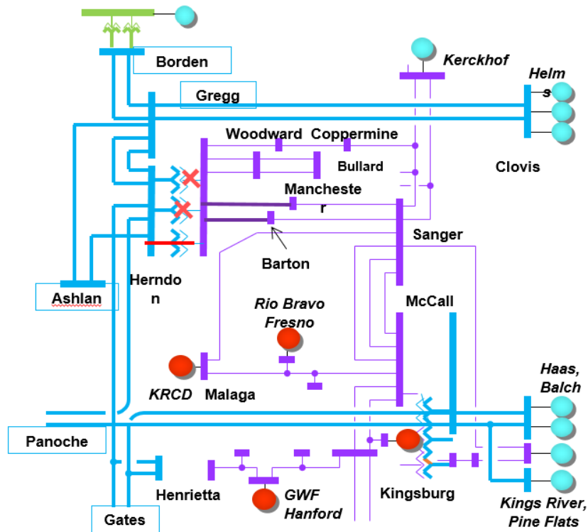
Figure 3.2-50 Herndon LCR Sub-area
