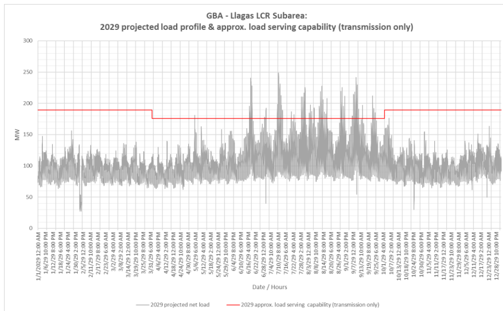
Figure 3-25 Llagas LCR Sub-area 2029 Forecast Hourly Profiles
