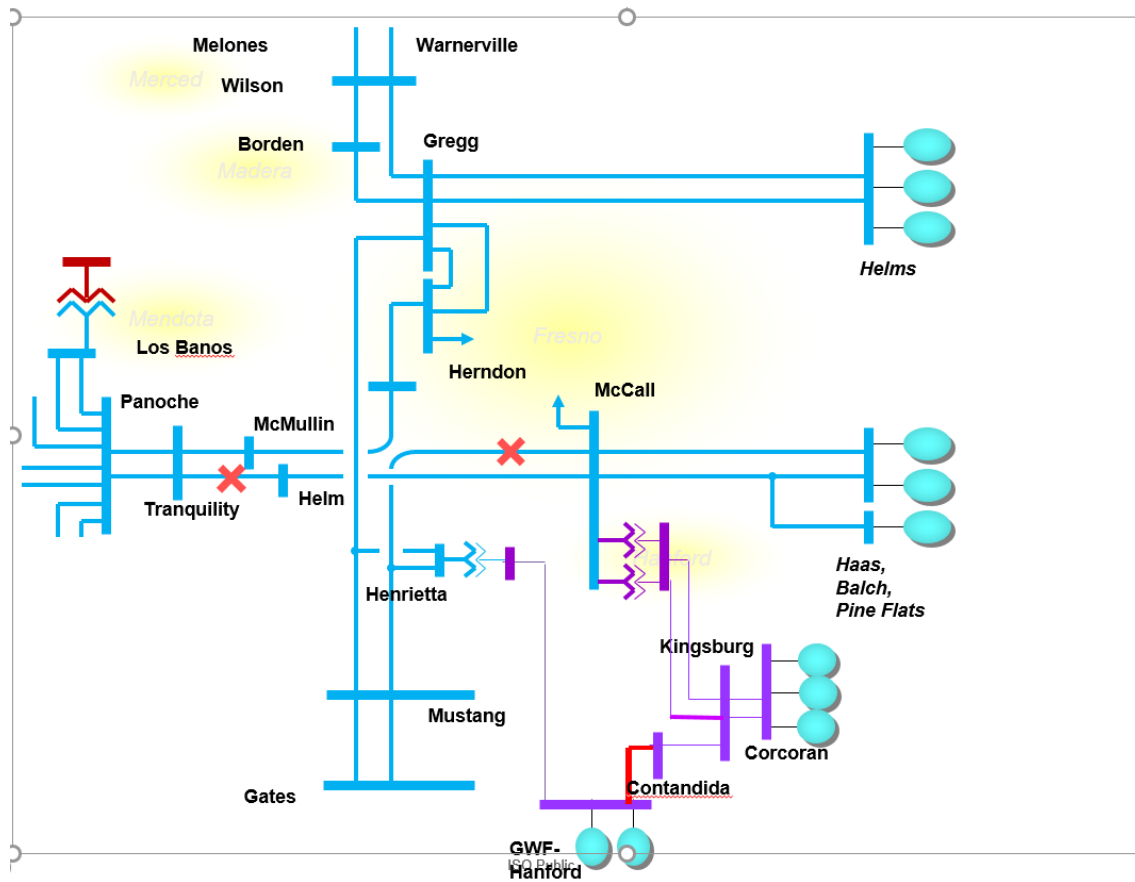
Figure 3.2-53 Fresno LCR area
