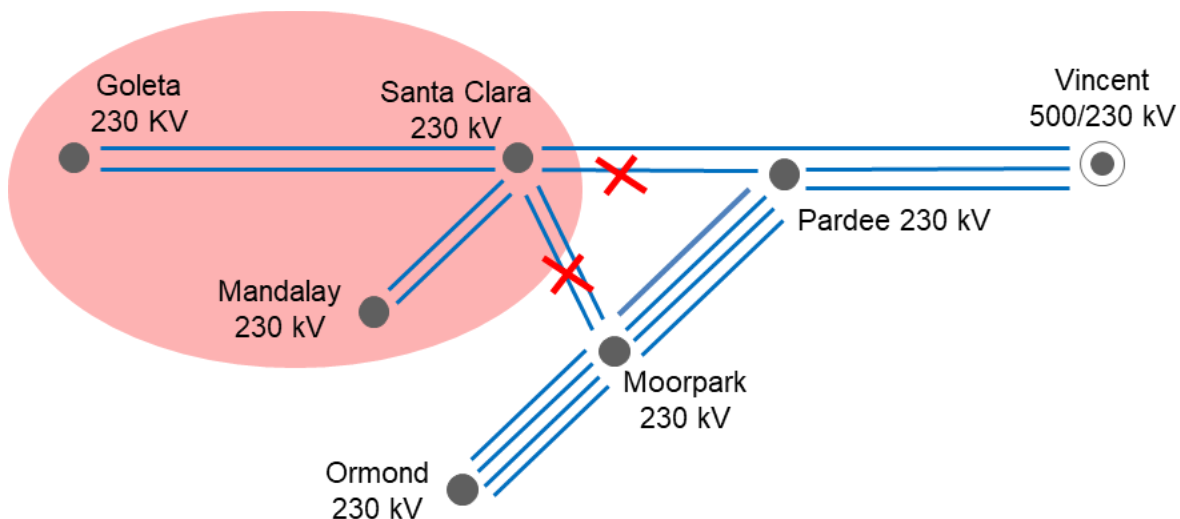
Figure 3.2-68 Santa Clara LCR Sub-area
