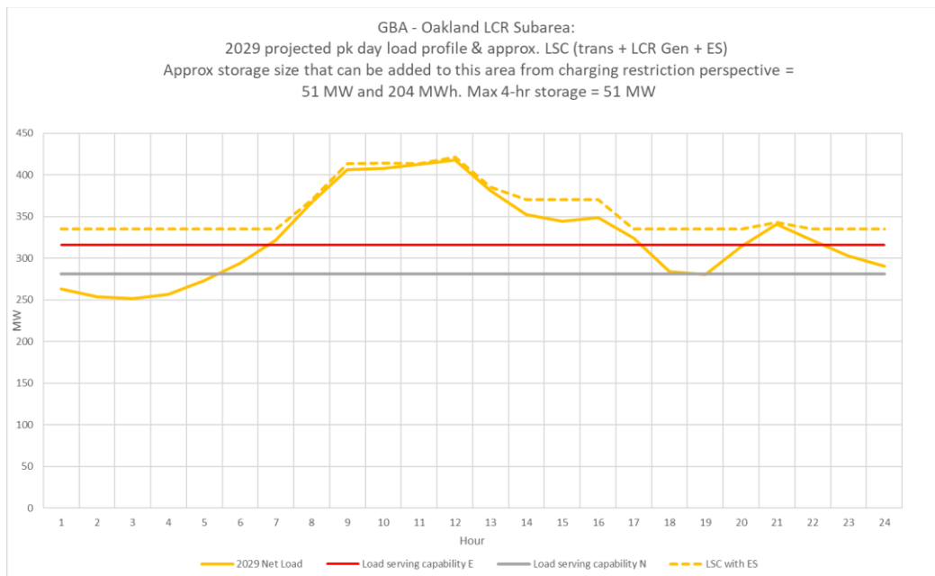
Figure 3-31 Oakland LCR Sub-area 2029 Peak Day Forecast Profiles
