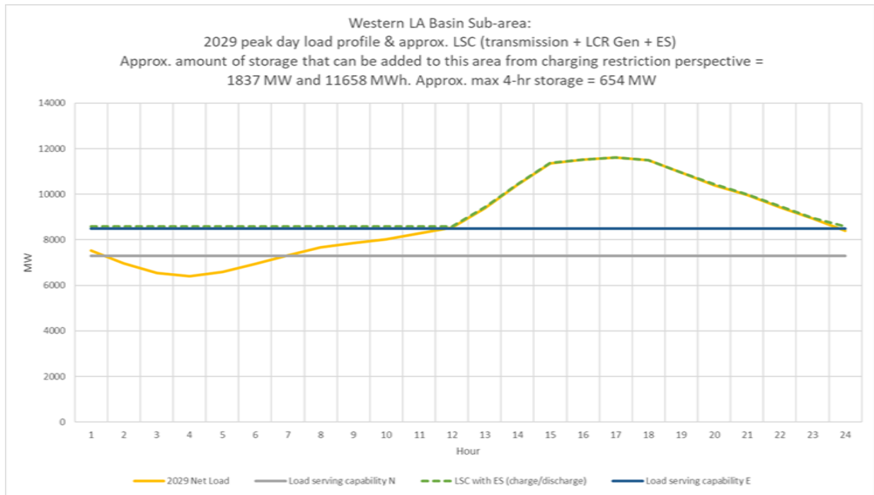
Figure 3.2-77 Western LA Basin LCR Sub-area 2029 Load Shape and Estimated Maximum Energy Storage Capacity and Energy Based on Charging Capability Under Critical Contingency
