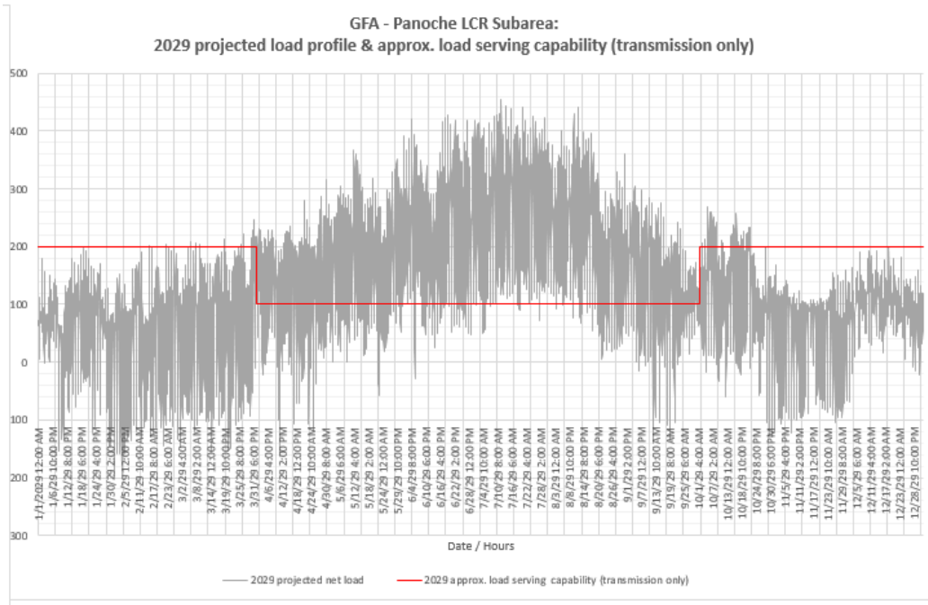
Figure 3.2-49 Panoche LCR Sub-area 2029 Forecast Hourly Profiles
