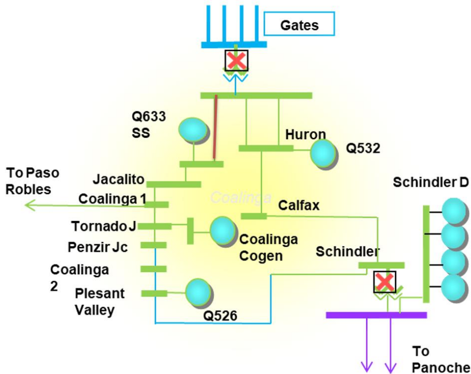
Figure 3.2-41 Coalinga LCR Sub-area
