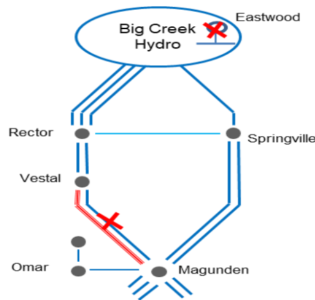
Figure 3.2-65 Vestal LCR Sub-area
