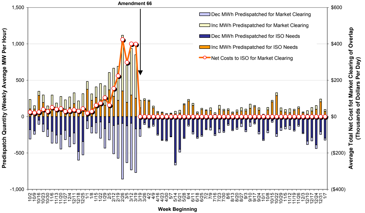
Figure 1. Average Hourly Volume of Bids Pre-Dispatched by the CAISO and Average Daily Costs to CAISO of Market Clearing (By Week Since Phase1B Implementation)
