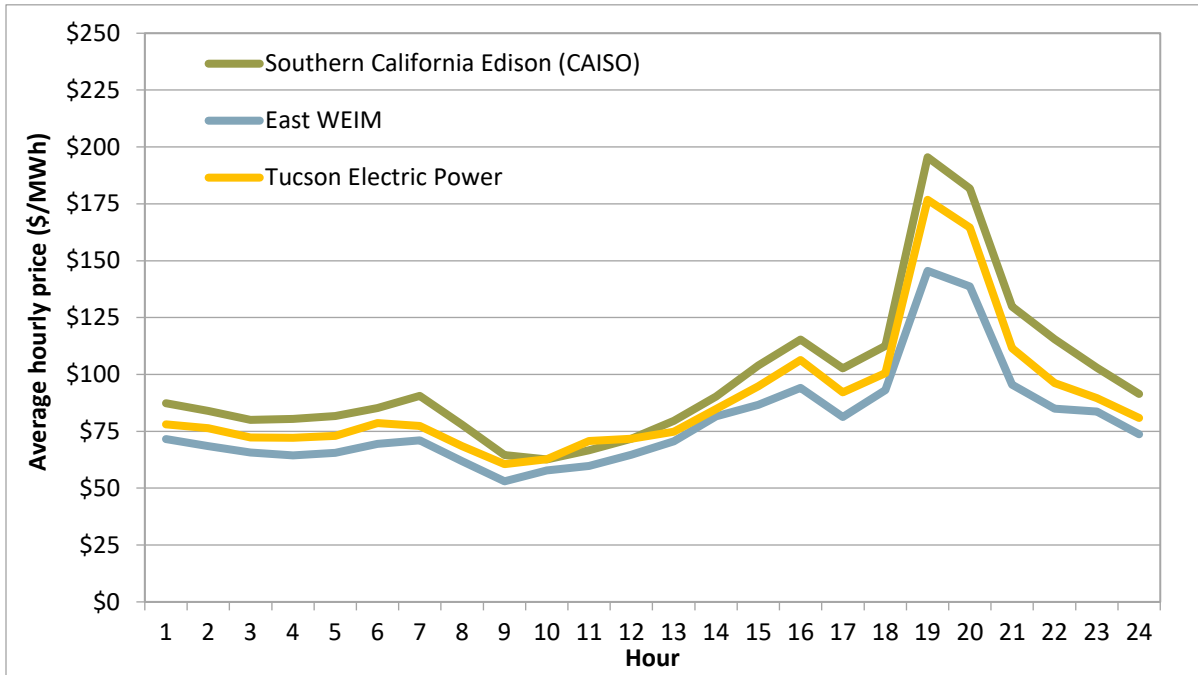
Figure 1.2 Average hourly 5-minute price (August 2022)
