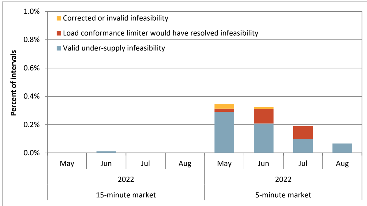
Figure 1.4 Frequency of under-supply power balance infeasibilities by month Tucson Electric Power (TEPC)
