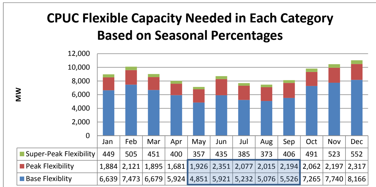
Revised Figure 8: CPUC Flexible Capacity Need in Each Category for 2015
