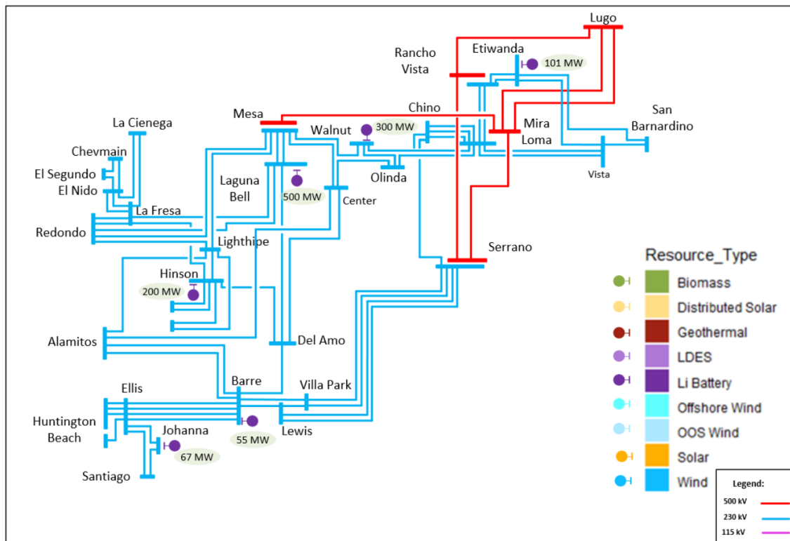
Figure F.13-1: SCE Metro Interconnection Area – Mapped 33 Base Portfolio
