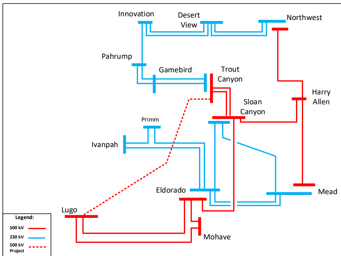
Figure F.10-3: Trout Canyon – Lugo 500 kV Line One-line Diagram
