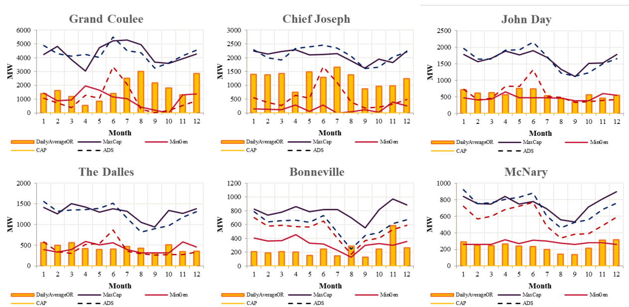
Figure 4.3-4: Min, Max, and Daily Operating Range for Mainstem Units for Medium Hydro Years
