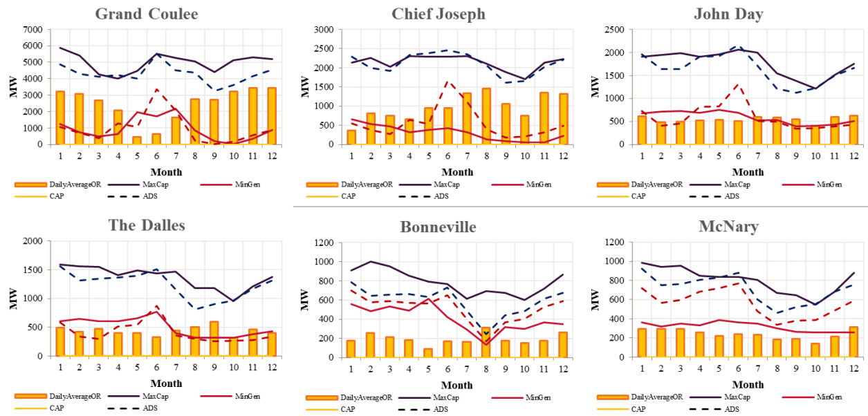
Figure 4.3-5: Min, Max, and Daily Operating Range for Mainstem Units for High Hydro Years
