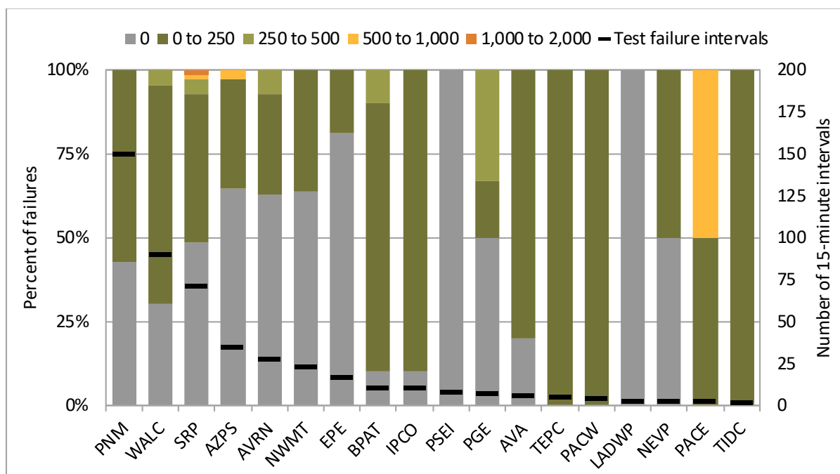
Figure 5.2 Upward capacity/flexibility test failure intervals by dynamic import limit (April 2023)
