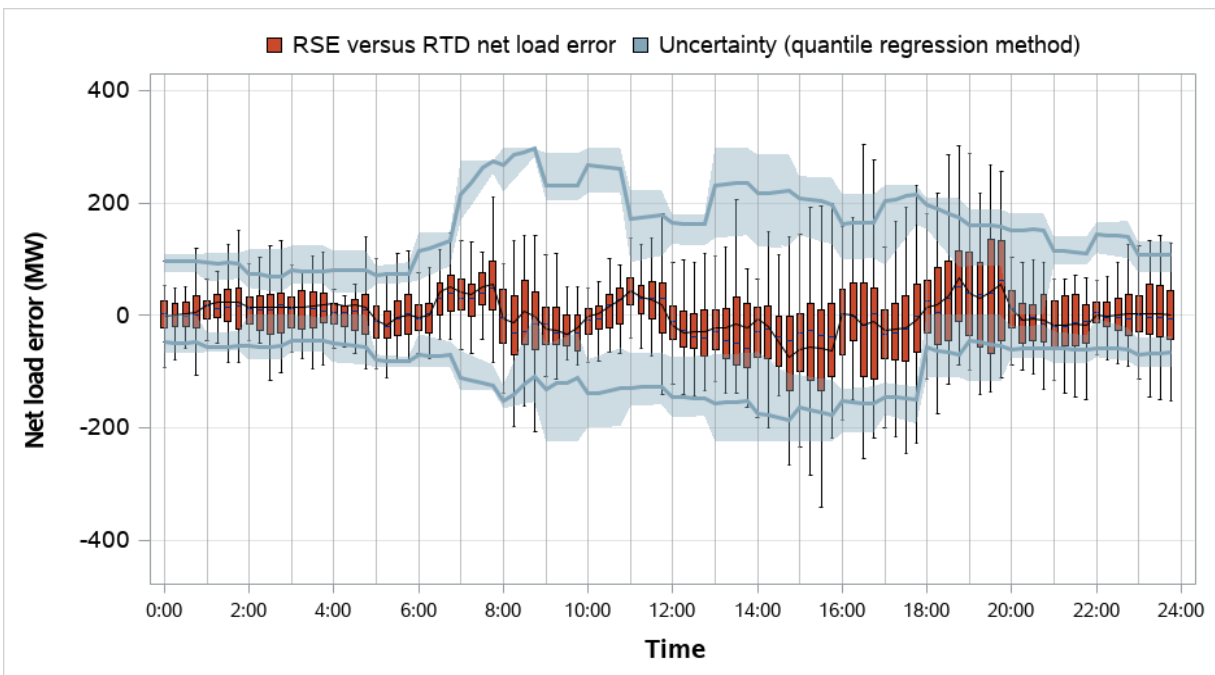
Figure 4.7 Arizona Public Service distribution of RSE and RTD net load error and comparison to RSE uncertainty (weekdays, April 2023)
