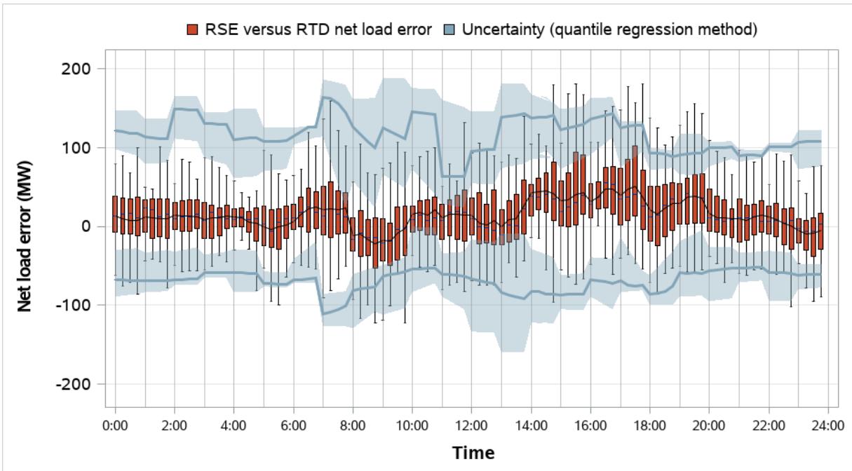
Figure 4.45 Tucson Electric Power distribution of RSE and RTD net load error and comparison to RSE uncertainty (weekdays, April 2023)
