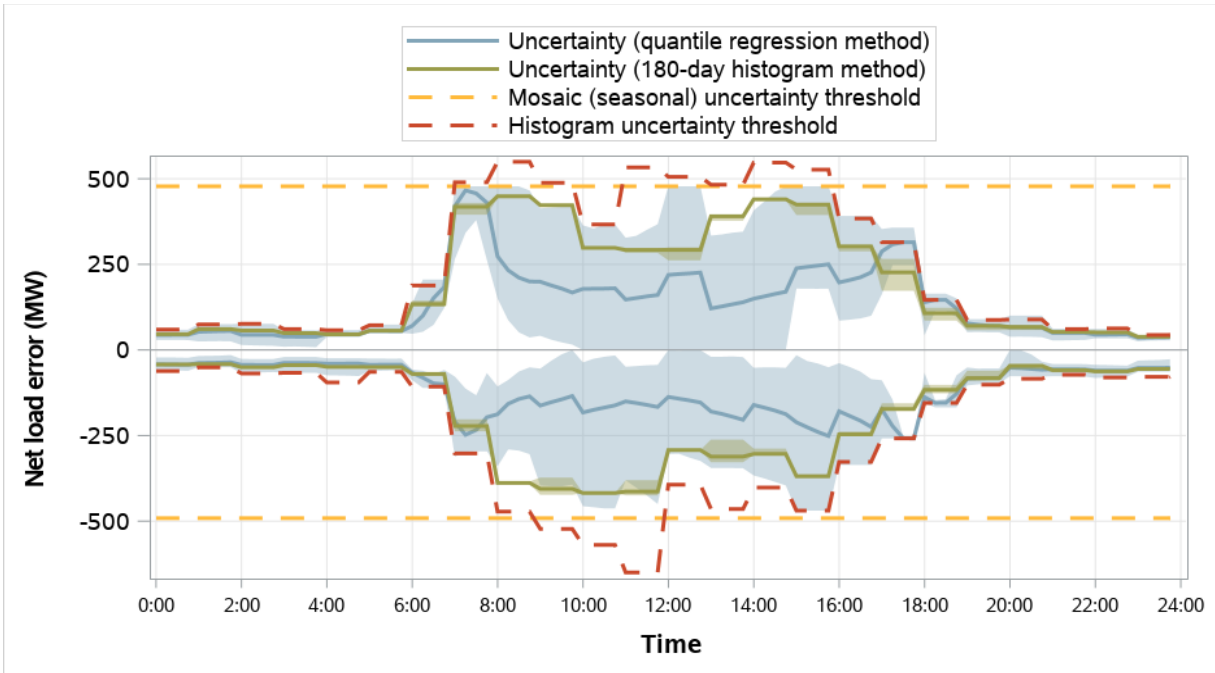
Figure 4.25 NV Energy distribution of RSE and RTD net load error and comparison to RSE uncertainty (weekdays, April 2023)
