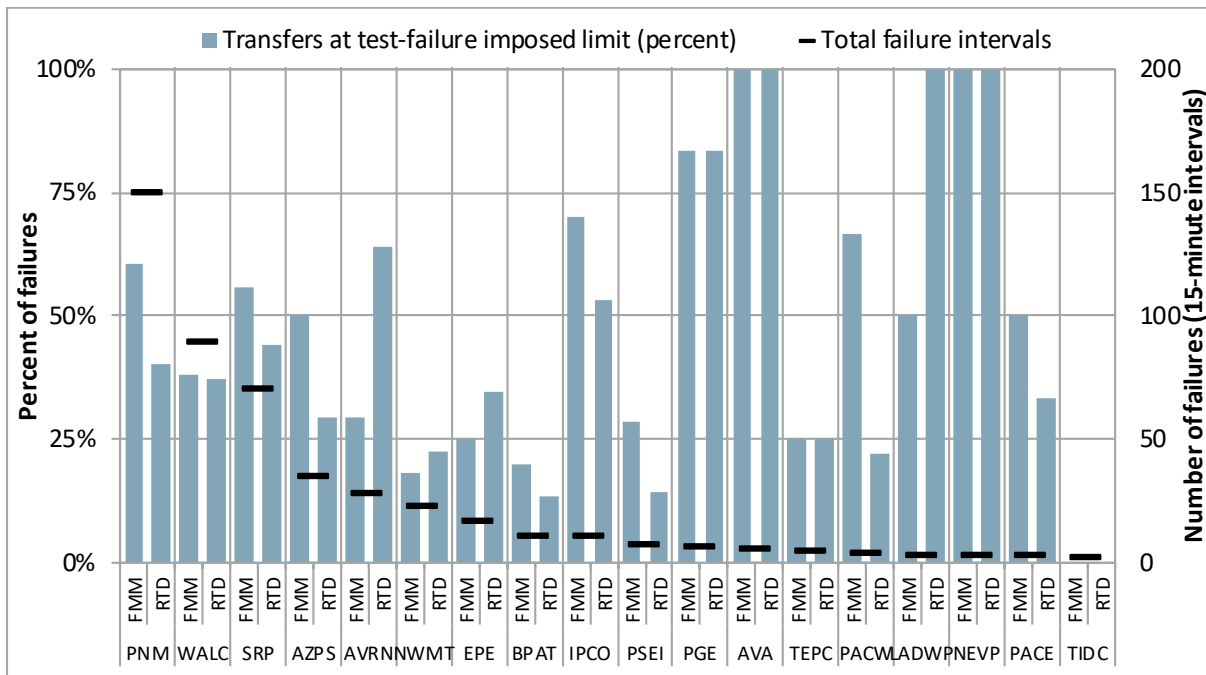
Figure 5.5 Percent of upward test failure intervals with market transfers at the imposed cap (April 2023)
