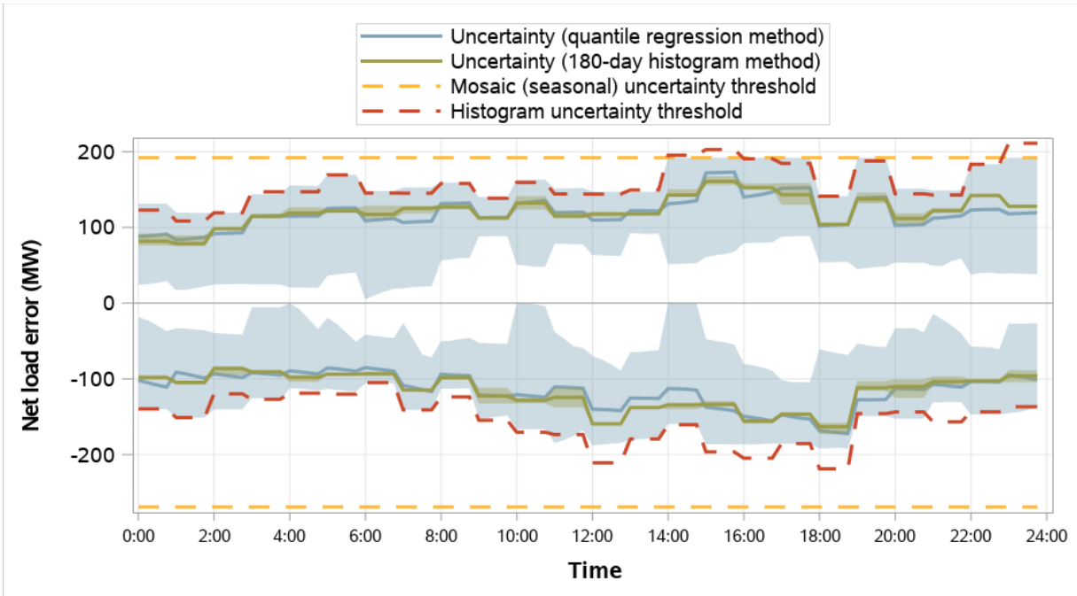
Figure 4.31 Portland General Electric distribution of RSE and RTD net load error and comparison to RSE uncertainty (weekdays, April 2023)
