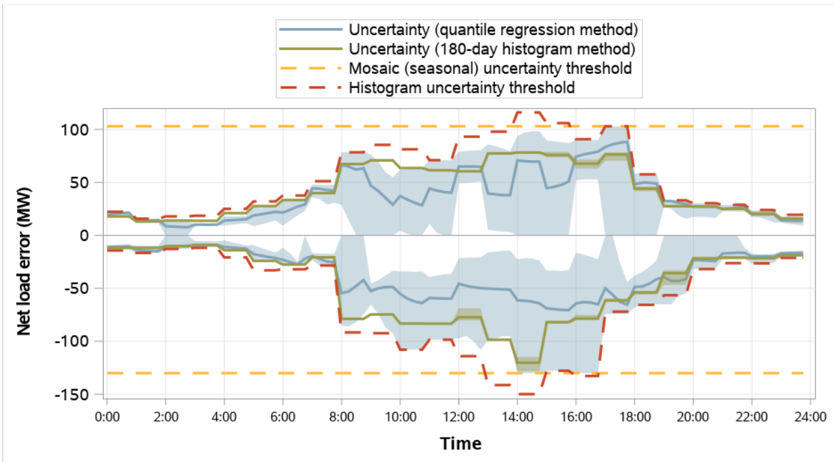
Figure 4.13 BANC distribution of RSE and RTD net load error and comparison to RSE uncertainty (weekdays, April 2023)
