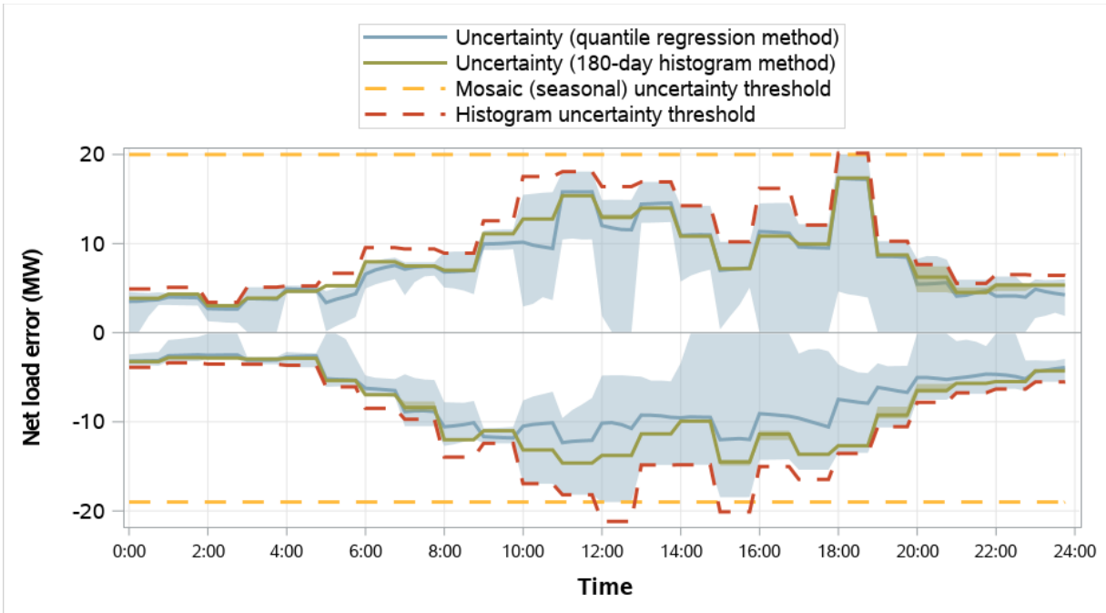
Figure 4.47 Turlock Irrigation District distribution of RSE and RTD net load error and comparison to RSE uncertainty (weekdays, April 2023)
