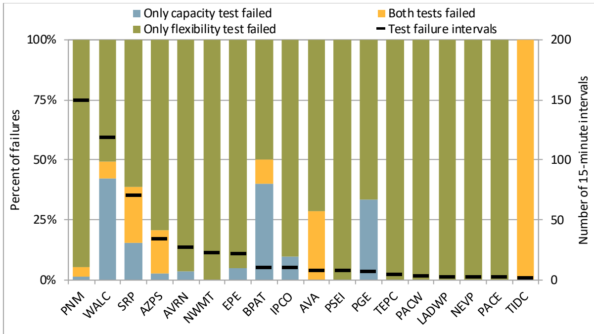
Figure 3.9 Upward capacity/flexibility test failure intervals by concurrence (April 2023)
