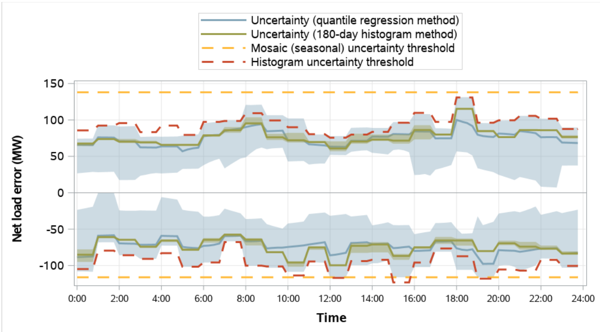
Figure 4.23 NorthWestern Energy distribution of RSE and RTD net load error and comparison to RSE uncertainty (weekdays, April 2023)
