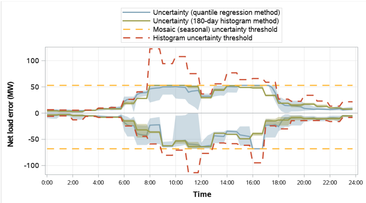
Figure 4.17 El Paso Electric distribution of RSE and RTD net load error and comparison to RSE uncertainty (weekdays, April 2023)
