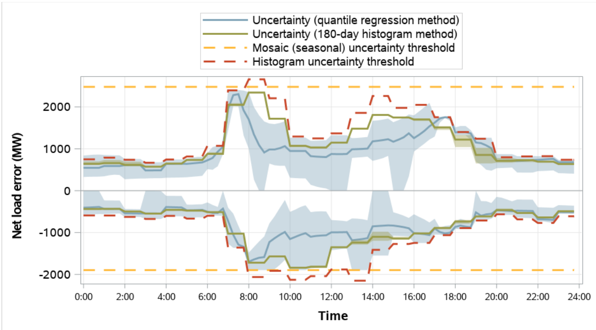
Figure 4.4 CAISO resource sufficiency evaluation uncertainty requirements (weekdays, April 2023)
