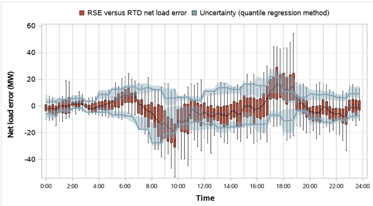
Figure 4.49 WAPA Desert Southwest distribution of RSE and RTD net load error and comparison to RSE uncertainty (weekdays, April 2023)
