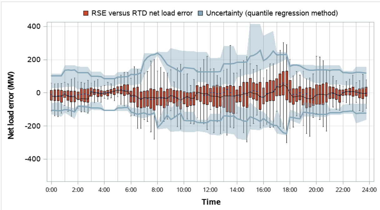
Figure 4.21 LADWP distribution of RSE and RTD net load error and comparison to RSE uncertainty (weekdays, April 2023)
