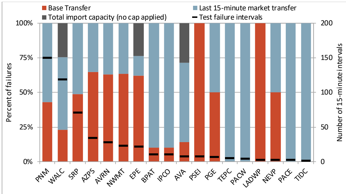
Figure 5.1 Upward capacity/flexibility test failure intervals by source of import limit (April 2023)
