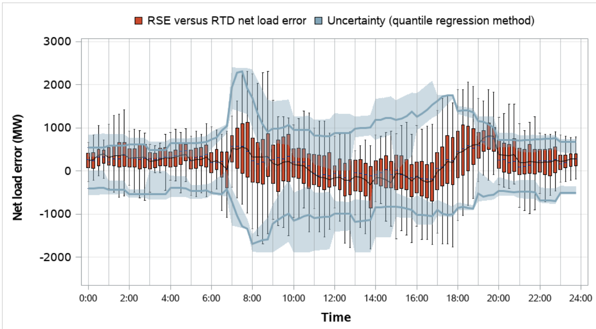
Figure 4.5 CAISO distribution of RSE and RTD net load error and comparison to RSE uncertainty (weekdays, April 2023)
