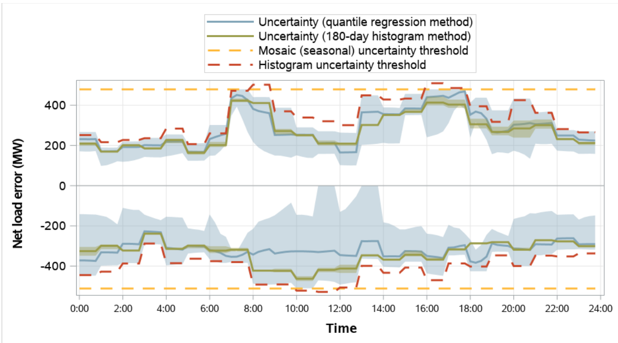
Figure 4.27 PacifiCorp East distribution of RSE and RTD net load error and comparison to RSE uncertainty (weekdays, April 2023)
