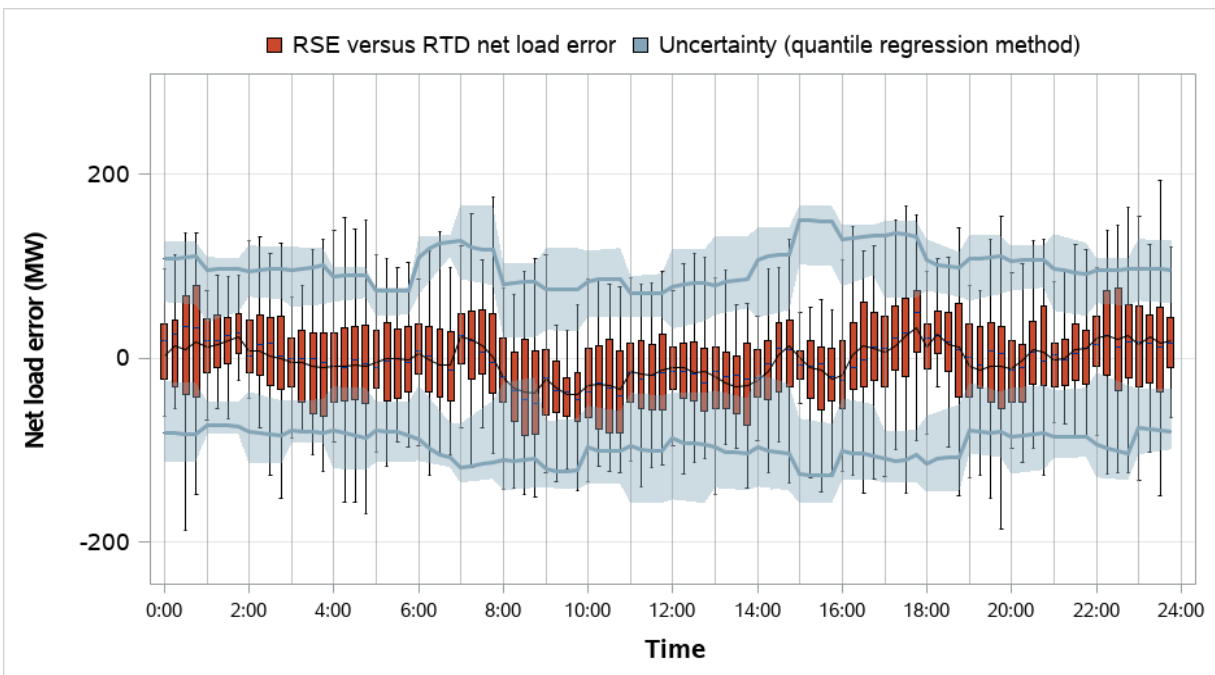
Figure 4.35 PNM distribution of RSE and RTD net load error and comparison to RSE uncertainty (weekdays, April 2023)
