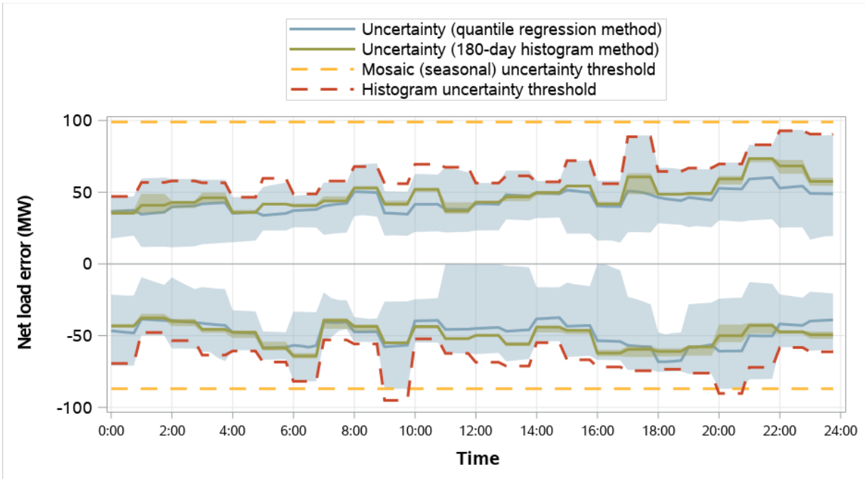
Figure 4.11 Avista distribution of RSE and RTD net load error and comparison to RSE uncertainty (weekdays, April 2023)
