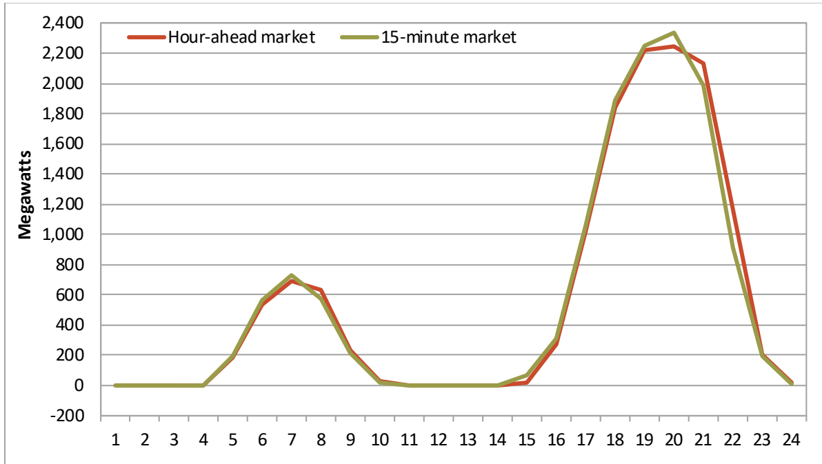
Figure 6.1 Average CAISO hour-ahead and 15-minute market load conformance (April 2023)
