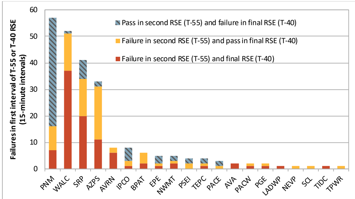
Figure 3.11 Upward resource sufficiency evaluation failures in first 15-minute interval of hour (April 2023)
