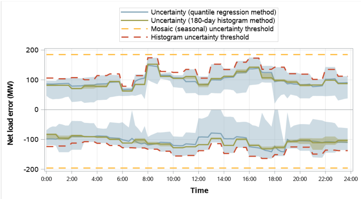
Figure 4.29 PacifiCorp West distribution of RSE and RTD net load error and comparison to RSE uncertainty (weekdays, April 2023)
