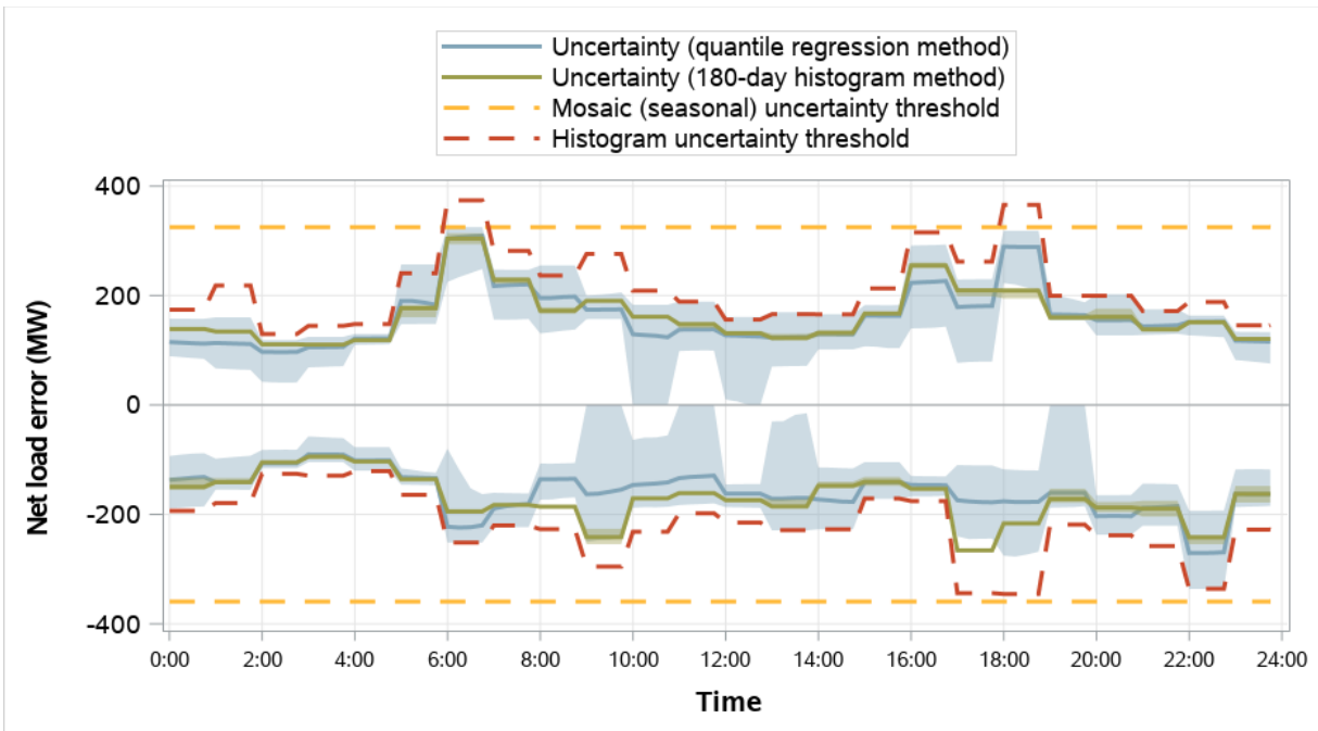
Figure 4.33 Powerex distribution of RSE and RTD net load error and comparison to RSE uncertainty (weekdays, April 2023)
