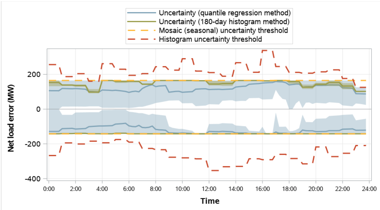
Figure 4.9 Avangrid distribution of RSE and RTD net load error and comparison to RSE uncertainty (weekdays, April 2023)
