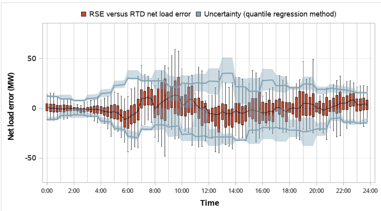
Figure 4.41 Seattle City Light distribution of RSE and RTD net load error and comparison to RSE uncertainty (weekdays, April 2023)
