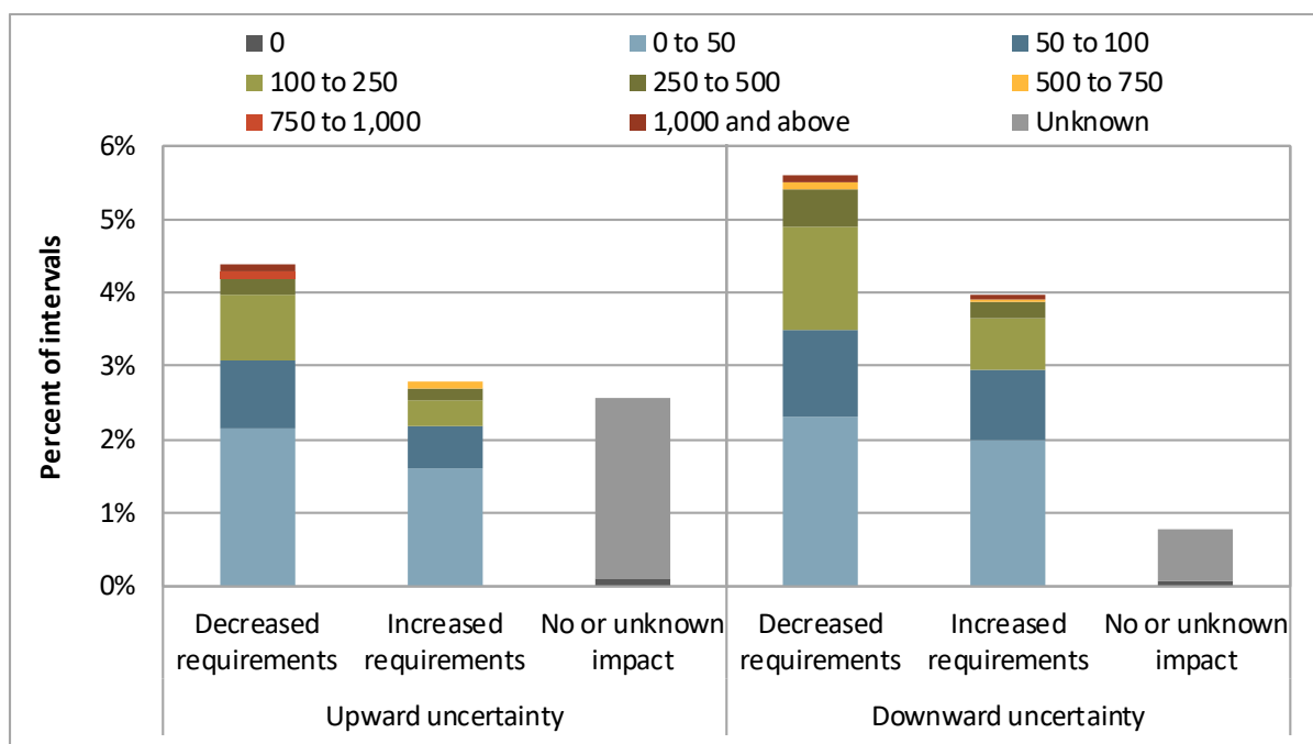
Figure 3.13 Impact of pass-group inconsistency on uncertainty requirements (April 2023)
