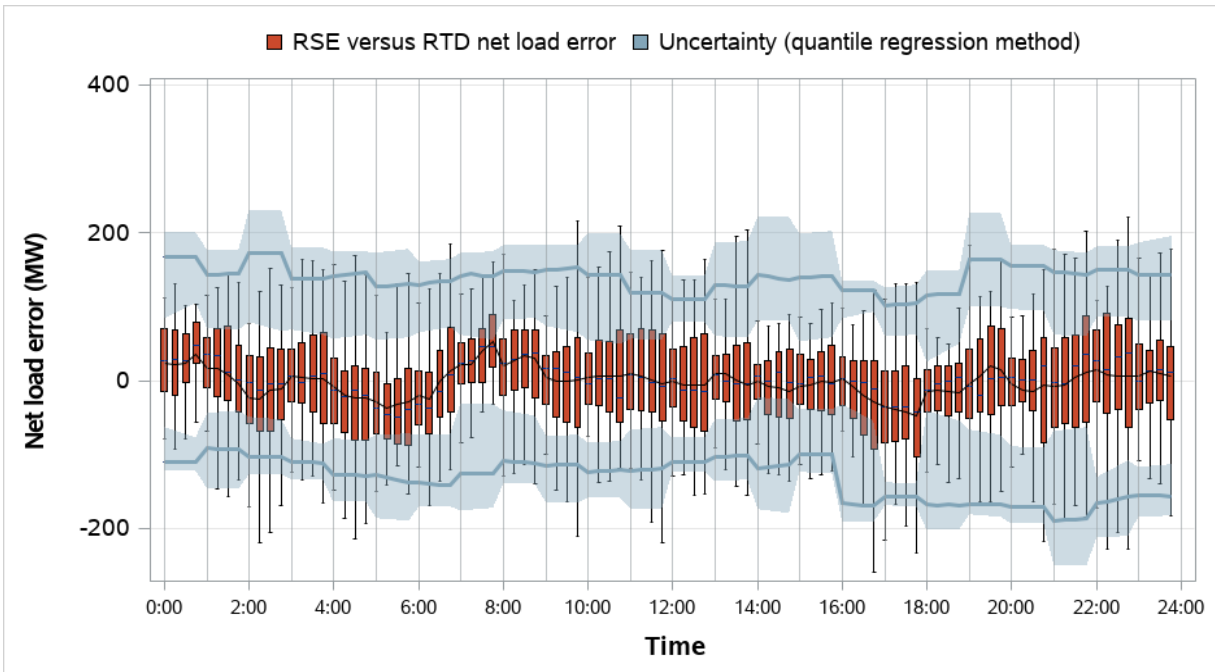
Figure 4.37 Puget Sound Energy distribution of RSE and RTD net load error and comparison to RSE uncertainty (weekdays, April 2023)
