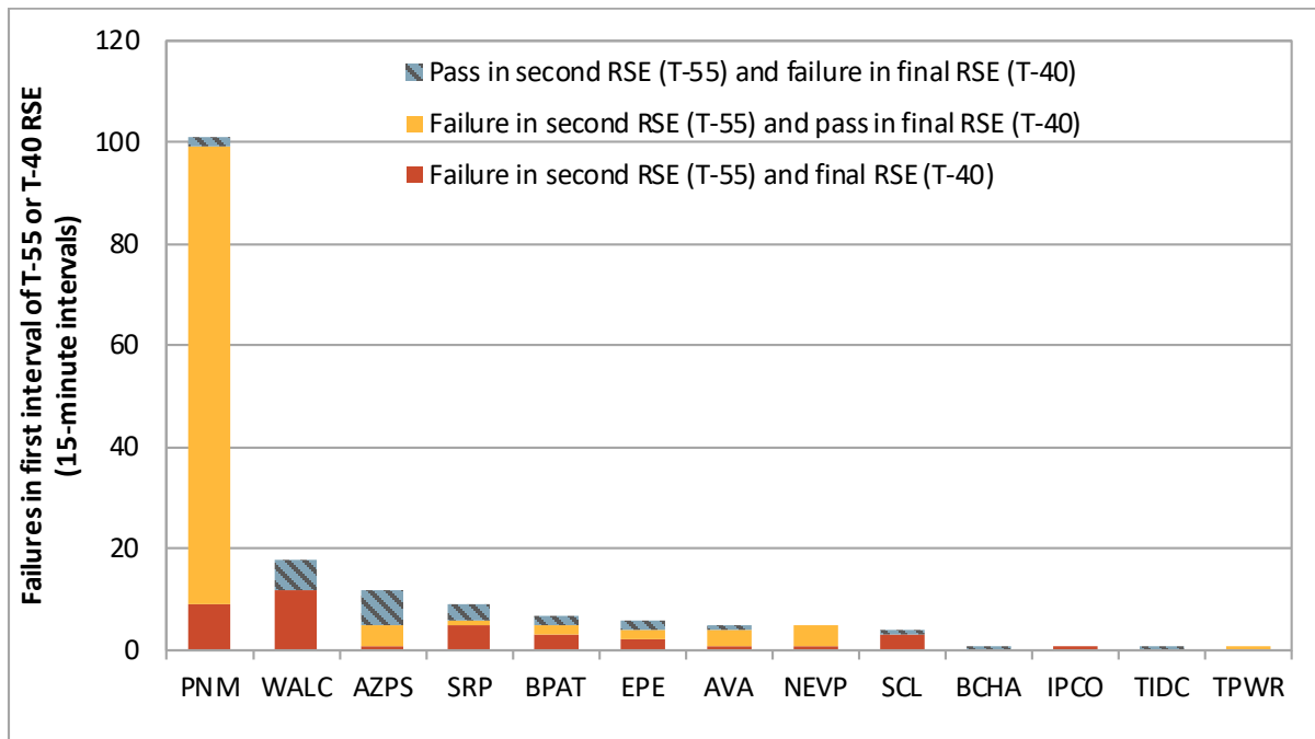
Figure 3.12 Downward resource sufficiency evaluation failures in first 15-minute interval of hour (April 2023)
