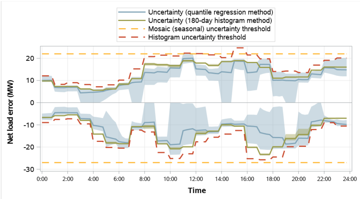
Figure 4.43 Tacoma Power distribution of RSE and RTD net load error and comparison to RSE uncertainty (weekdays, April 2023)
