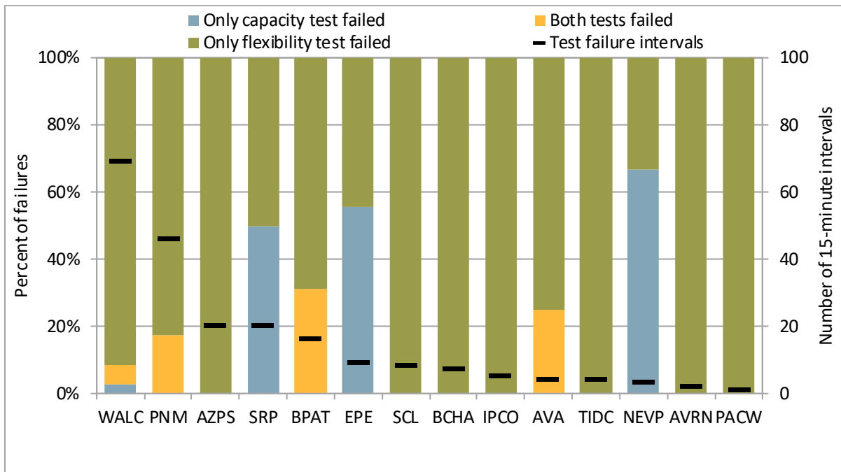
Figure 3.10 Downward capacity/flexibility test failure intervals by concurrence (April 2023)
