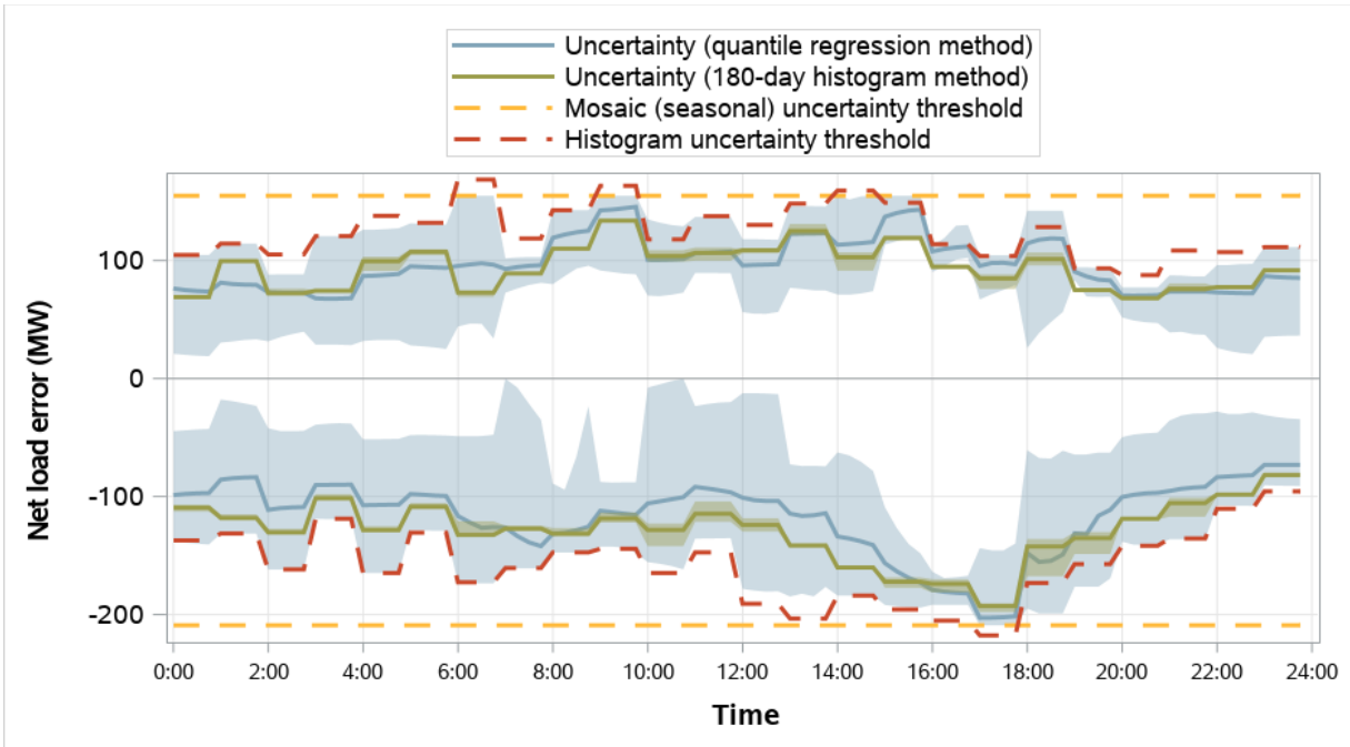
Figure 4.19 Idaho Power distribution of RSE and RTD net load error and comparison to RSE uncertainty (weekdays, April 2023)
