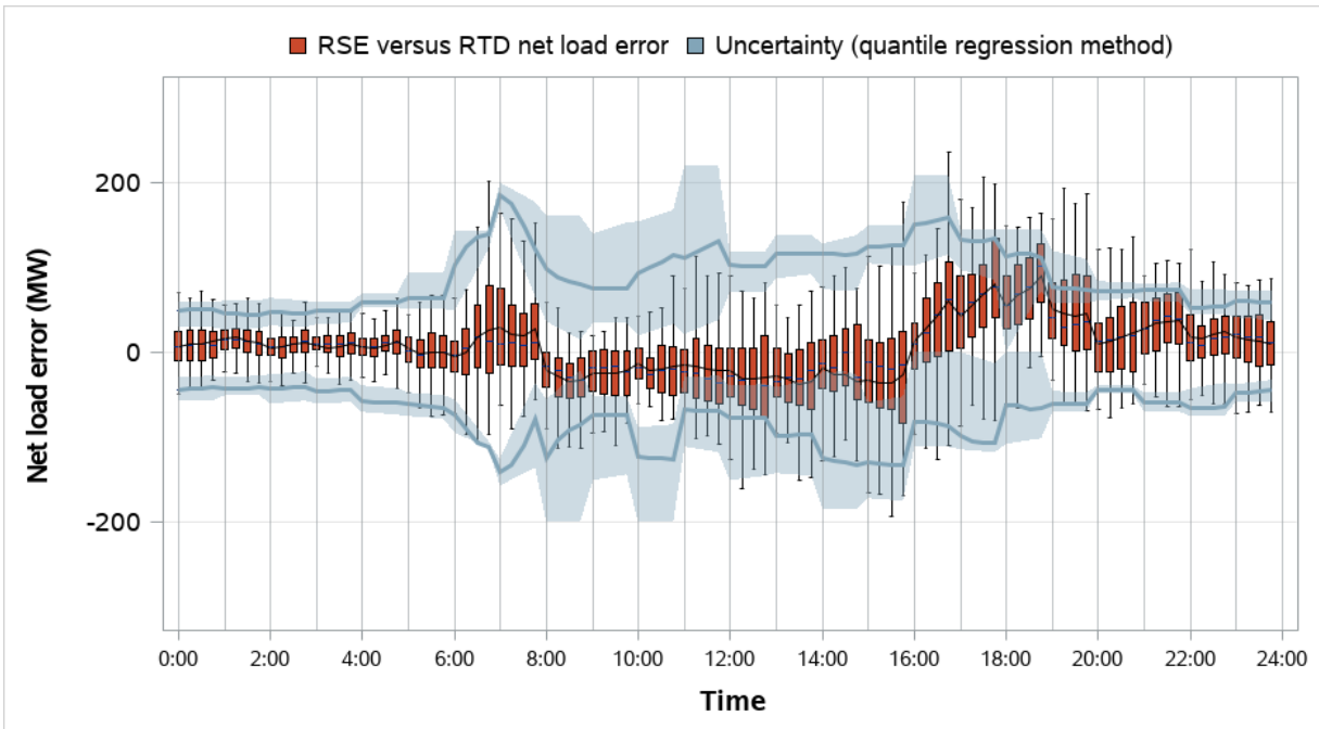
Figure 4.39 Salt River Project distribution of RSE and RTD net load error and comparison to RSE uncertainty (weekdays, April 2023)
