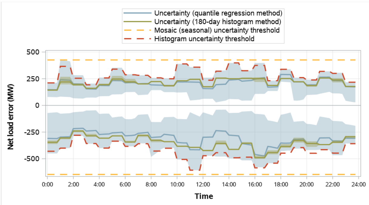
Figure 4.15 BPA distribution of RSE and RTD net load error and comparison to RSE uncertainty (weekdays, April 2023)
