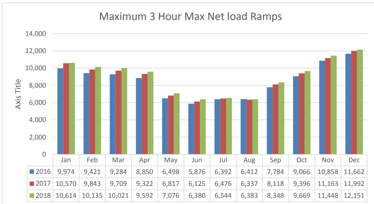
Figure 1: ISO System Maximum 3-hour Net-Load Ramps
