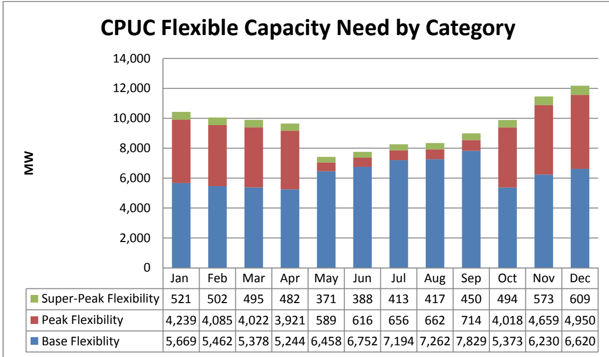
Figure 8: CPUC Flexible Capacity Need in Each Category for 2015
