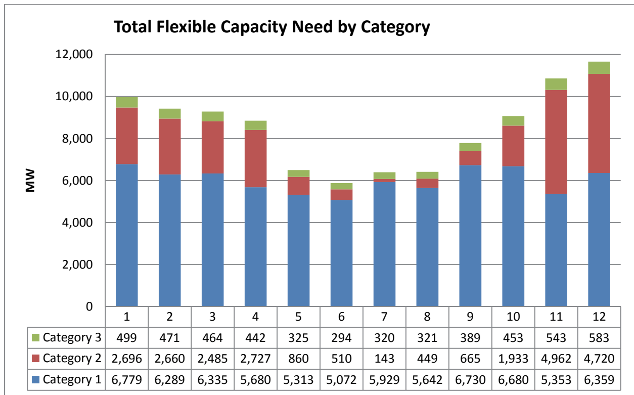
Figure 3: ISO System-Wide Flexible Capacity Monthly Calculation by Category for 2016
