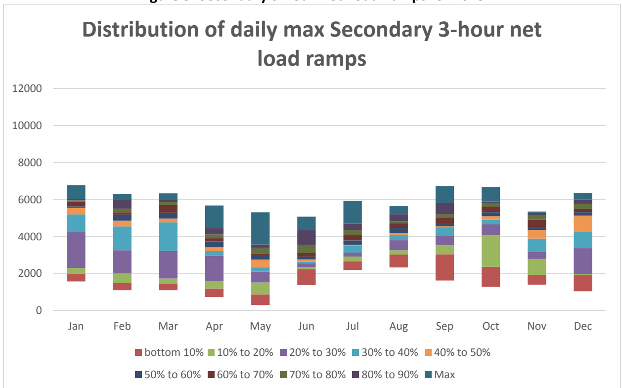
Figure 5: Secondary 3-hour Net-Load Ramps for 2015
