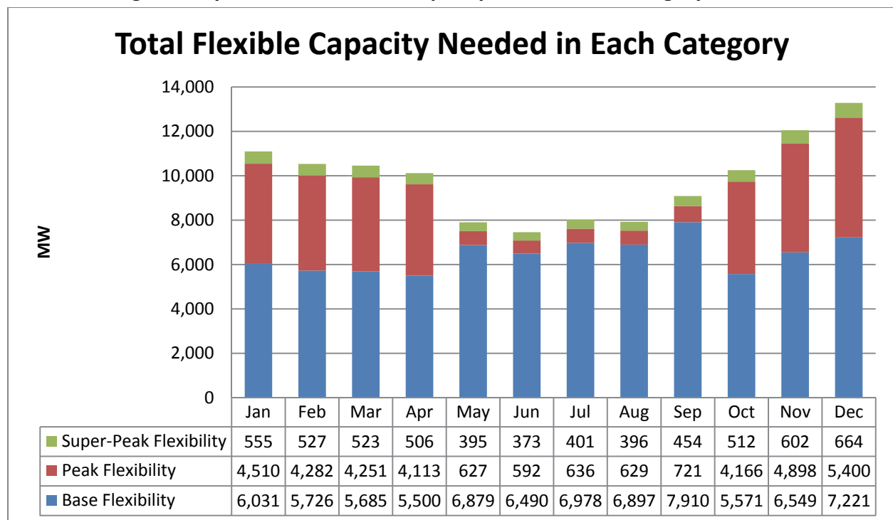
Figure 6: System-wide Flexible Capacity Need in Each Category for 2016
