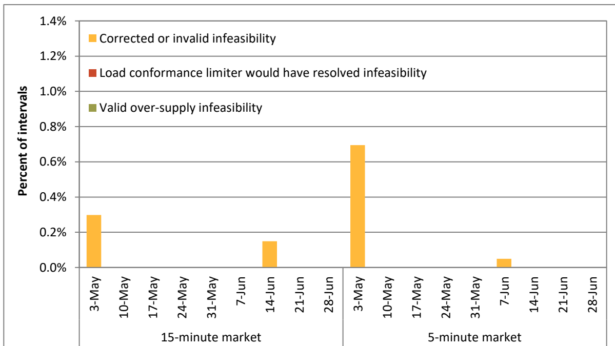
Figure 1.4 Frequency of over-supply power balance infeasibilities by week Bonneville Power Administration
