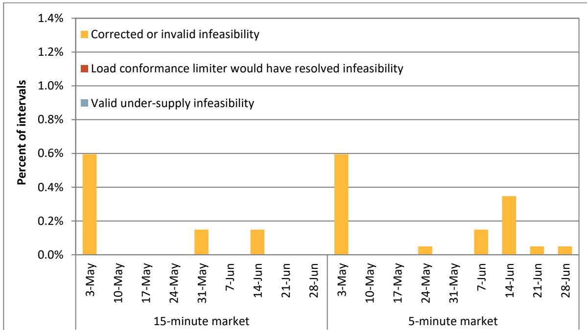
Figure 1.3 Frequency of under-supply power balance infeasibilities by week Bonneville Power Administration
