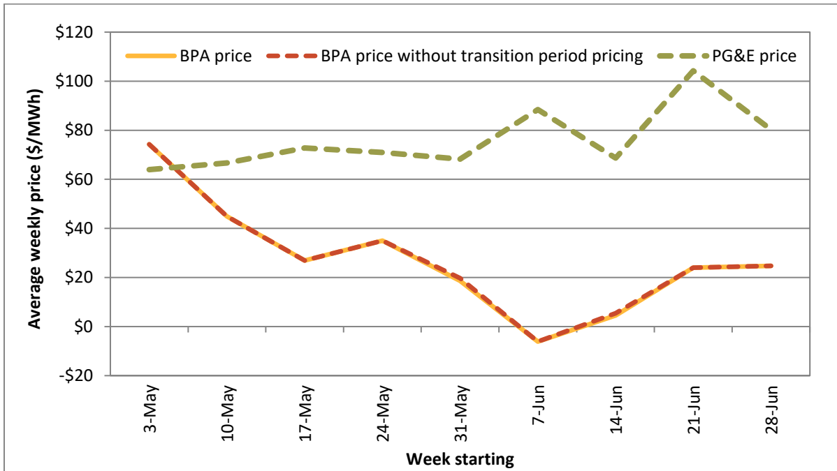
Figure 1.6 Average prices by week – Bonneville Power Administration (BPA) (5-minute market)
