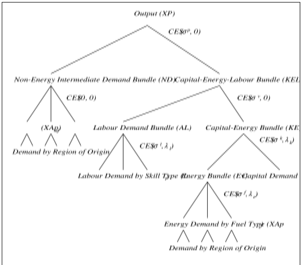
Figure 1: Production Nesting
