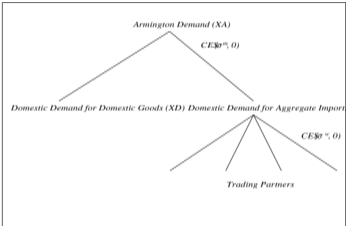
Figure 2: Armington Nesting
