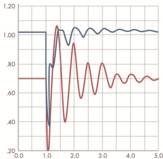
Figure 4.2.1-2: Frequency and voltage at the Wind Gap # 2 pump with the Midway-Gates 230 kV contingency in the 2024 Summer Peak Commercial Interest case
