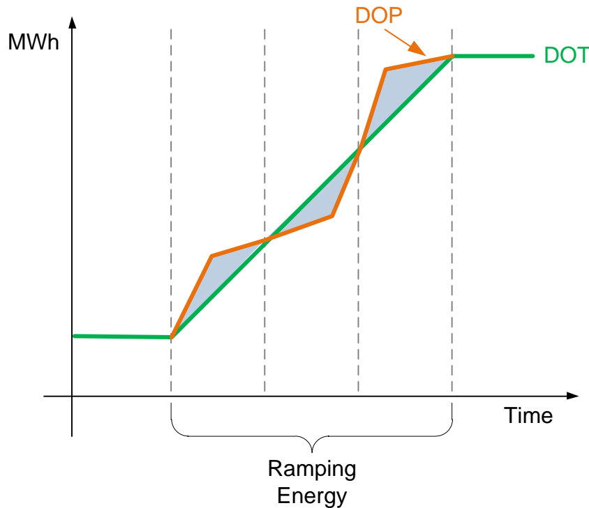
Figure 6.1-2: Ramping Tolerance
