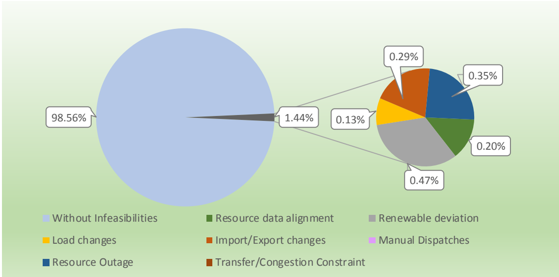
Figure 4: Frequency of undersupply infeasibility in the five-minute market in October - PAC West and PAC East combined.
