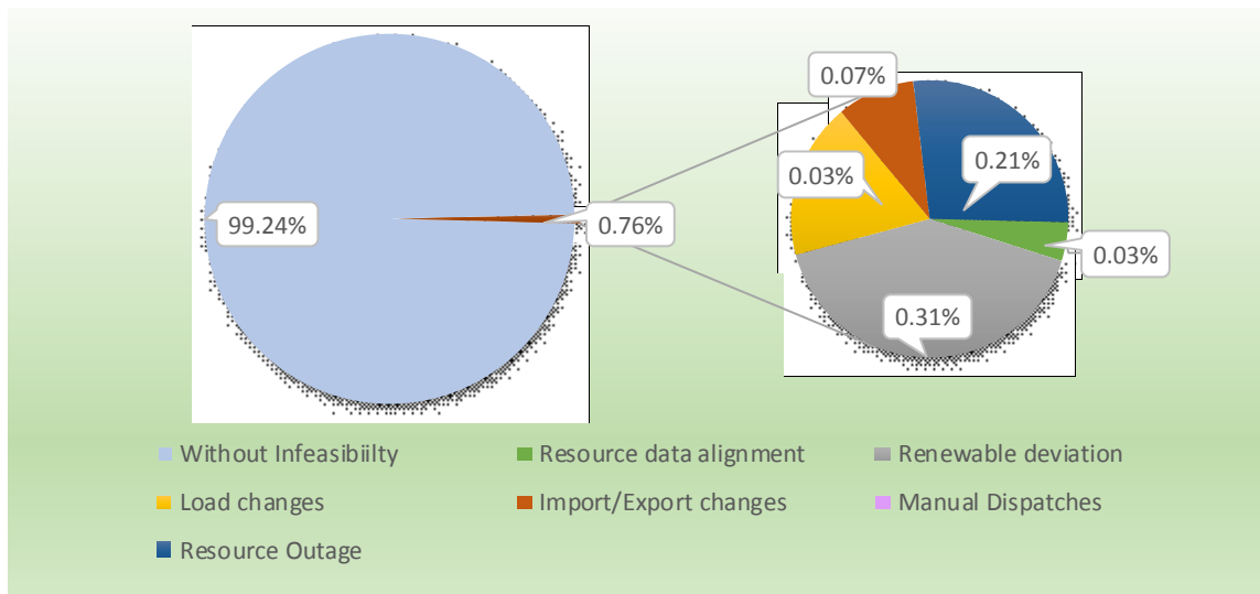
Figure 4: Frequency of undersupply infeasibility in the five-minute market in August-October - PAC West and PAC East combined.
