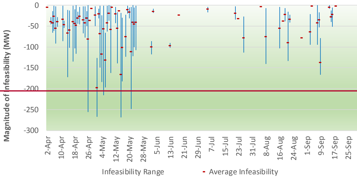
Figure 29: Magnitude of oversupply infeasibility PAC West, Five-minute market.
