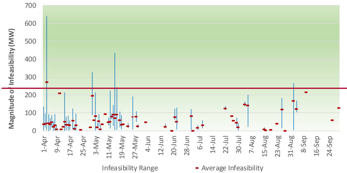
Figure 22: Magnitude of undersupply infeasibility PAC East. Five-minute market.
