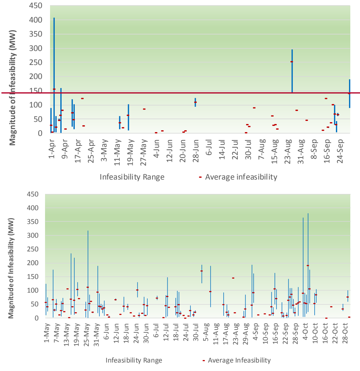
Figure 18: Magnitude of undersupply infeasibility PAC East FifteenWest . Five -minute market.
