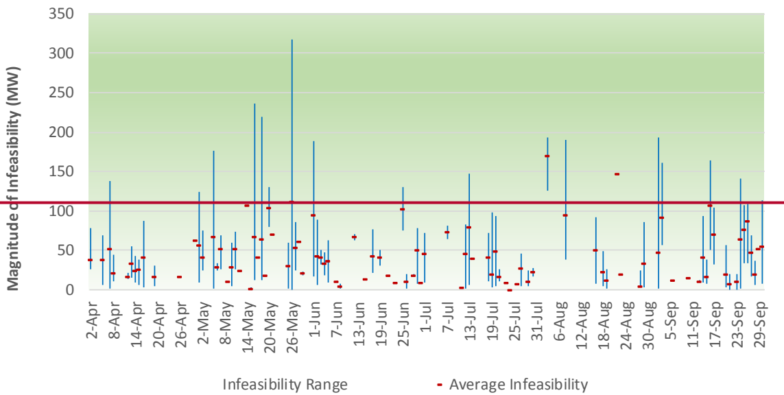
Figure 20: Magnitude of undersupply infeasibility PAC West. Five-minute market.
