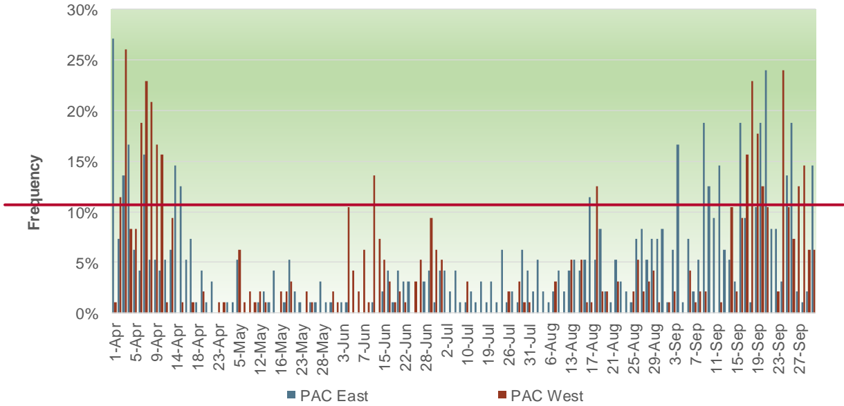
Figure 21: Frequency of flexible ramp constraint infeasibility in PAC
