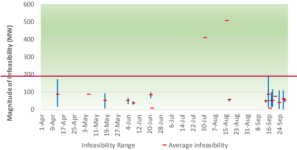
Figure 16: Magnitude of undersupply infeasibility in PAC WestEast. Fifteen-minute market.
