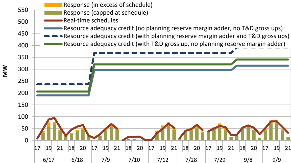
Figure 2.7 CPUC-jurisdictional utility reliability demand response resource (RDRR) performance
