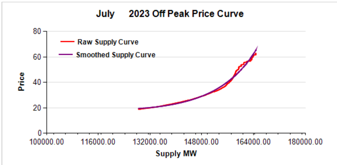
FIGURE 1: July 2023 OFF-PEAK REGRESSION RESULT
