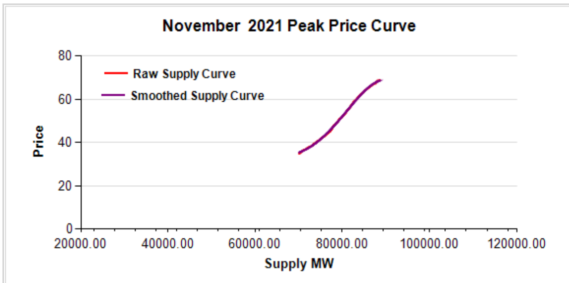
FIGURE 2: November 2021 ON-PEAK REGRESSION RESULT
