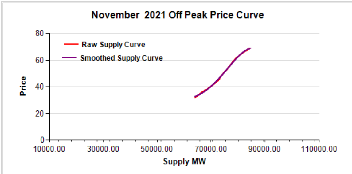
FIGURE 1: November 2021 OFF-PEAK REGRESSION RESULT
