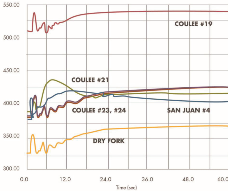
Figure 3.4-5: Generator’s output for an outage of two Palo Verde units with the highest response (WECC)
