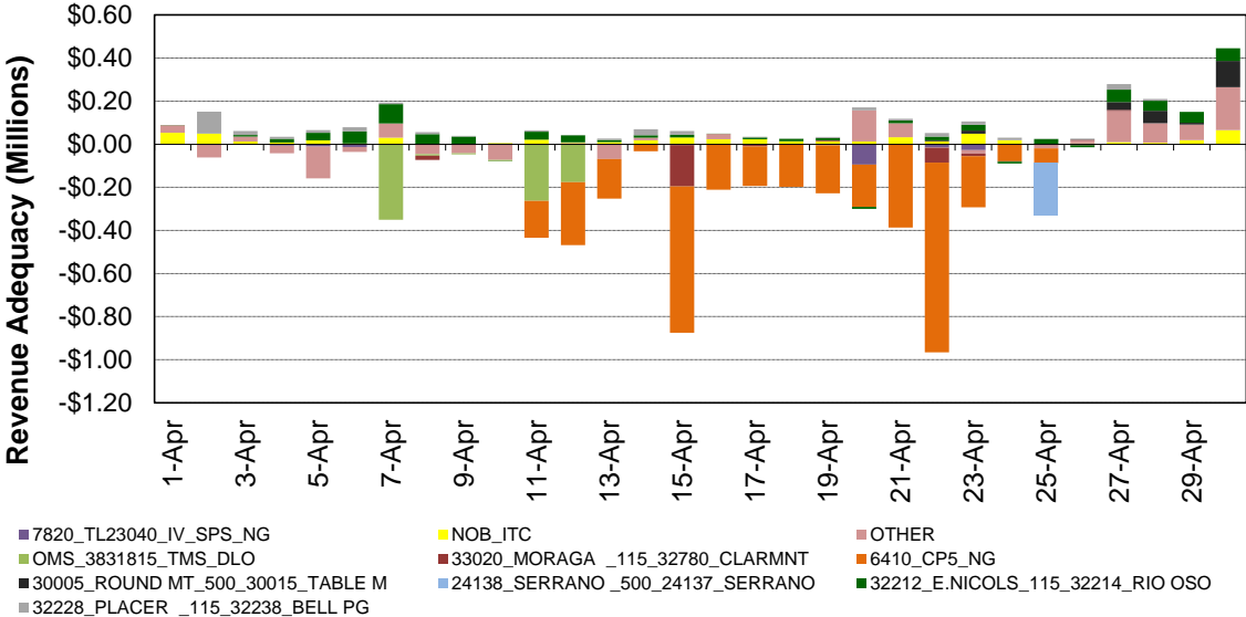
Figure 49: Daily CRR Revenue Adequacy by Transmission Element
