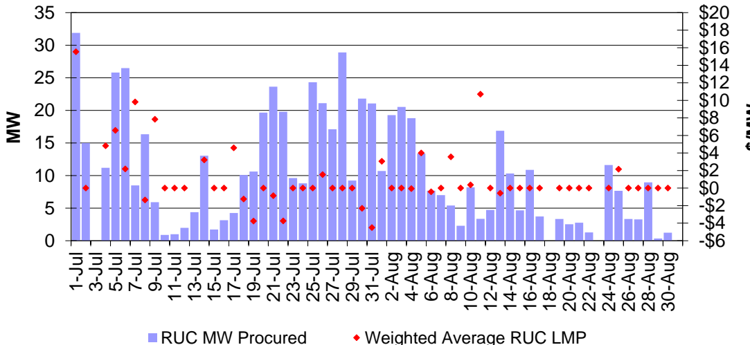
Figure 82: Daily RUC Award and LMP (All Hours)
