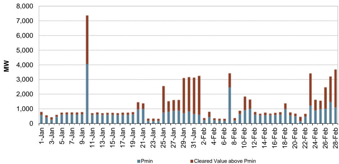
Figure 127: MOC Unit Commitment and Dispatch
