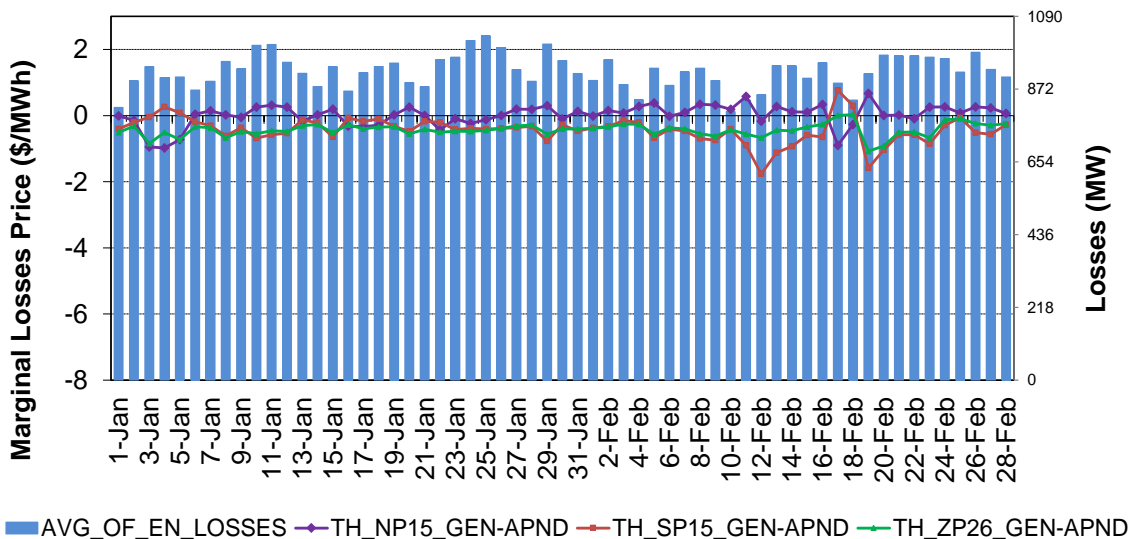
Figure 55: RTD Simple Average TH Prices for Losses
