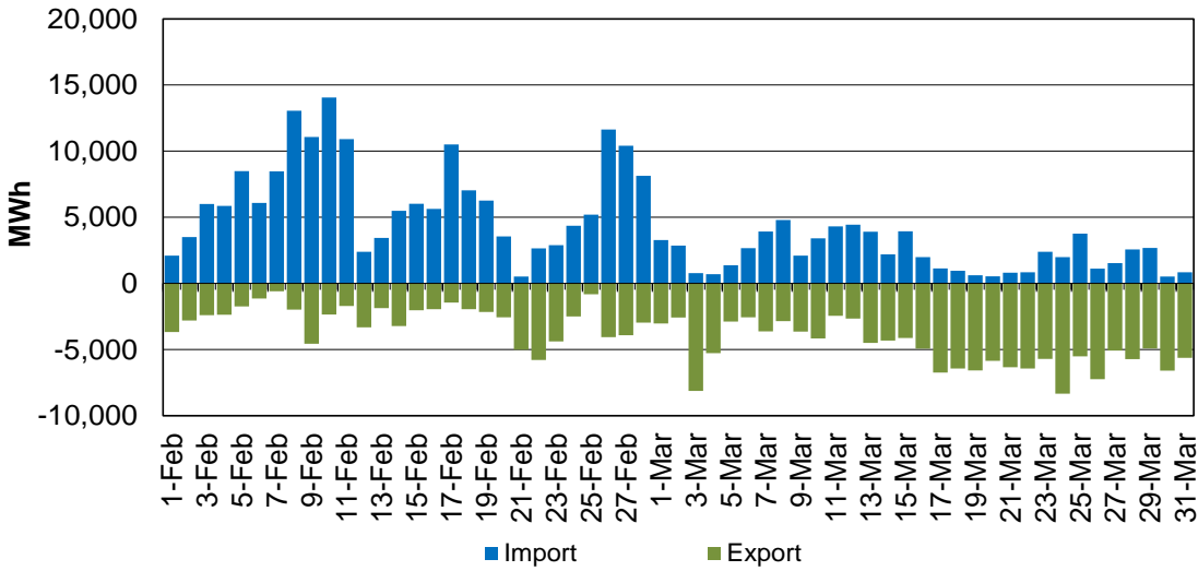
Figure 163: EIM Transfer for PSEI in RTD
