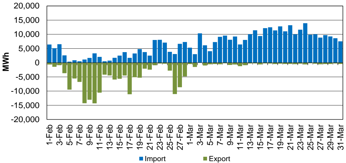
Figure 165: EIM Transfer for BCHA in RTD
