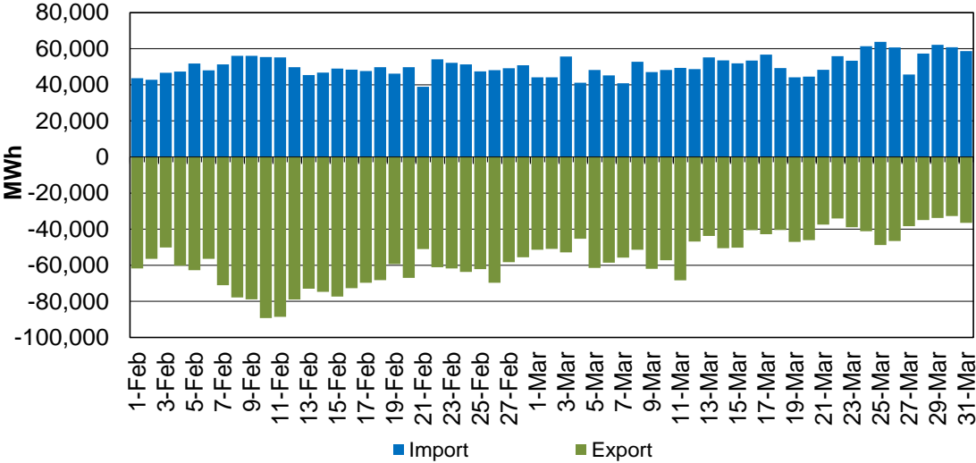
Figure 159: EIM Transfer for PACE in RTD
