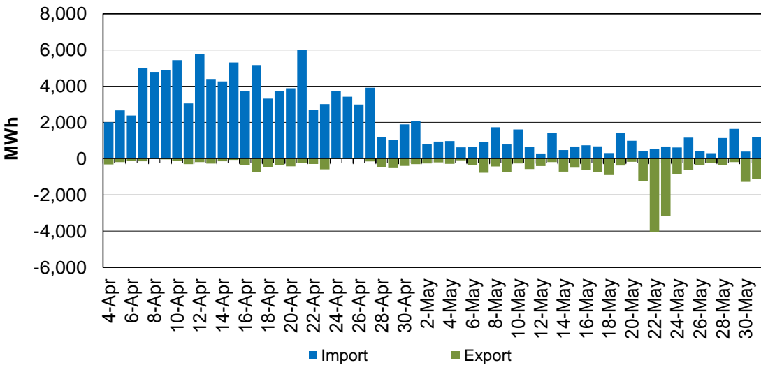
Figure 153: EIM Transfer for BCHA in FMM
