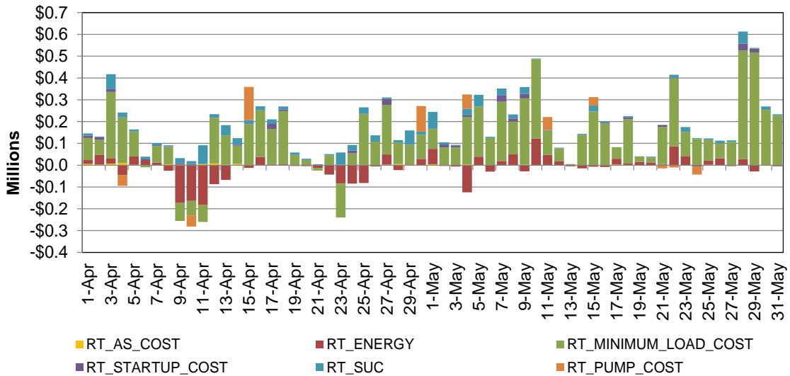
Figure 114: Cost in RT
