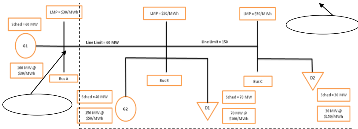
Figure 170: Day-Ahead Market Example 1
