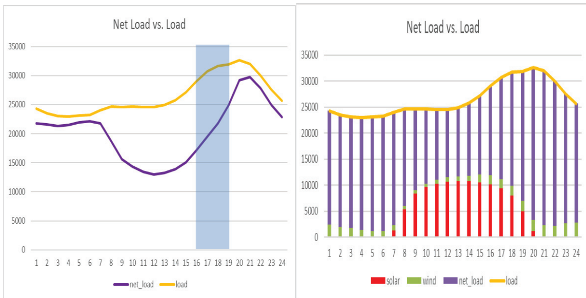
Figure 8: Examples of load contribution to net load ramp
