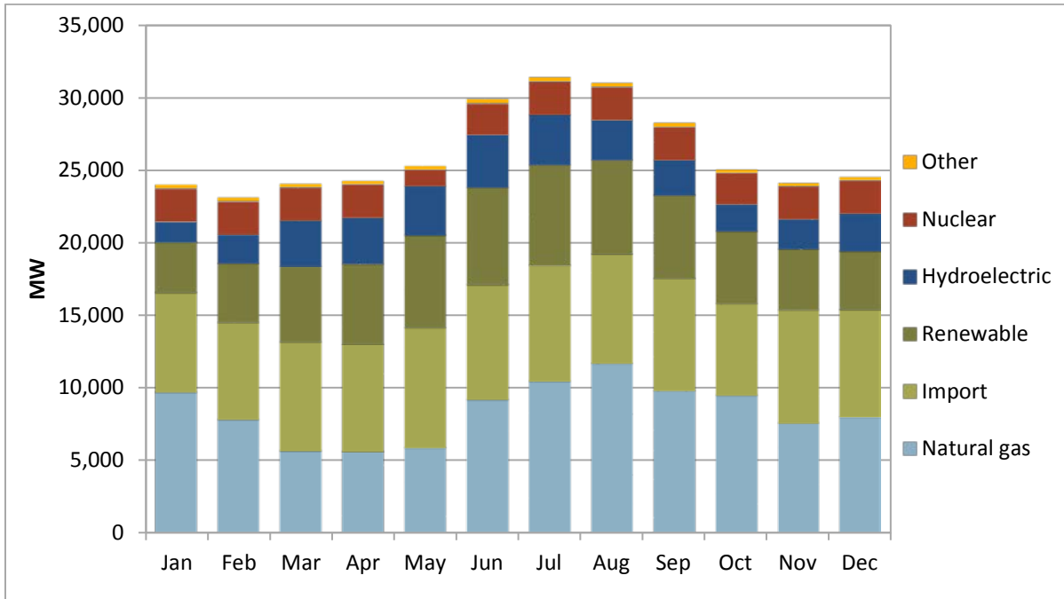
Figure 1.5 Average hourly generation by month and fuel type in 2016
