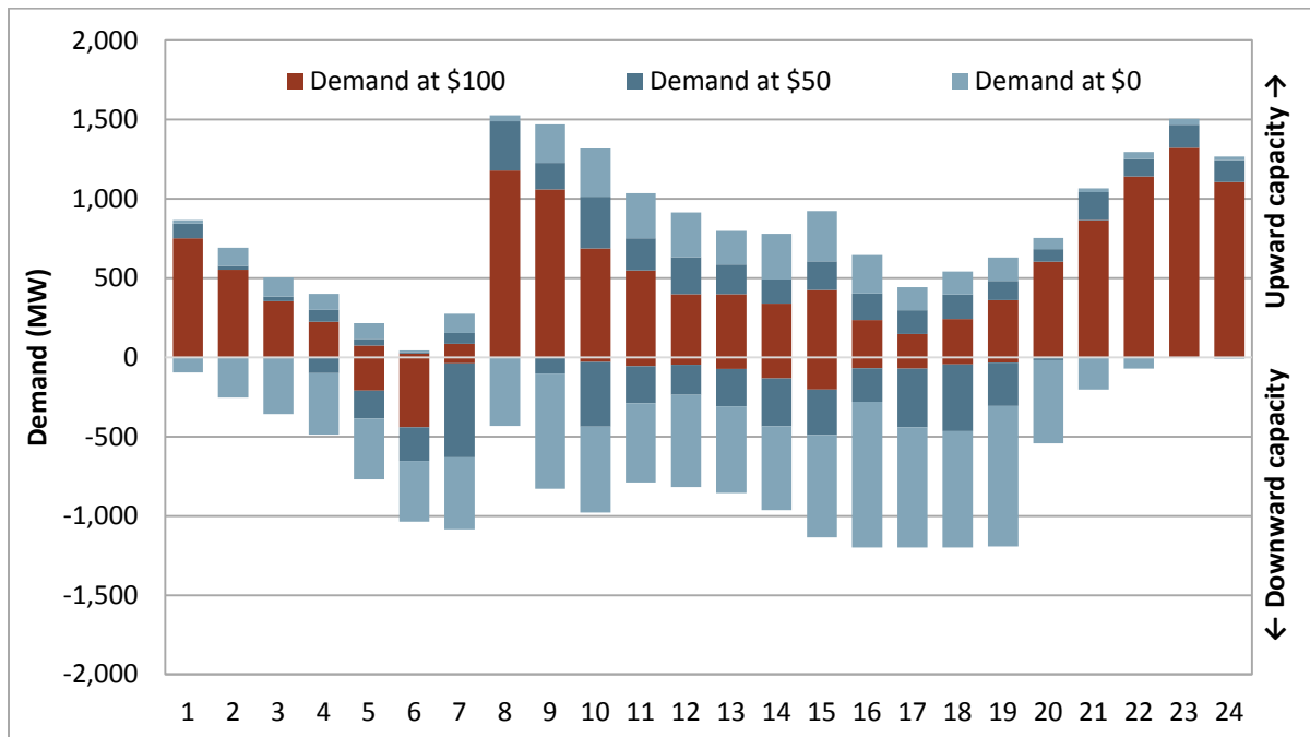
Figure 4.11 Hourly average system-level flexible ramping demand curves in 15-minute market (November – December)
