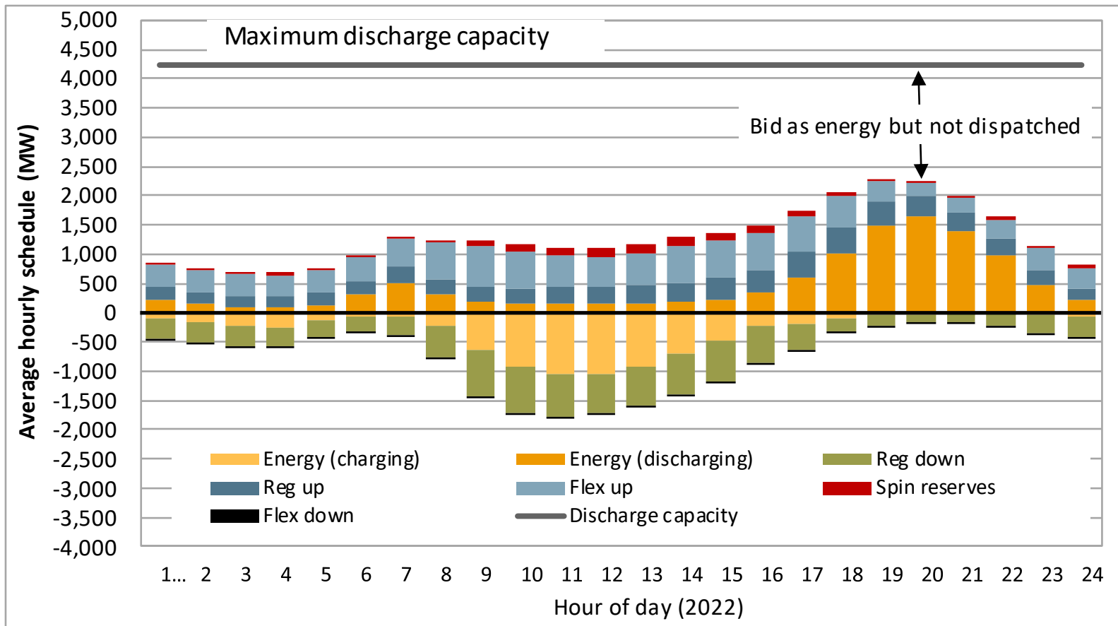
Hourly average battery schedules (2022)
