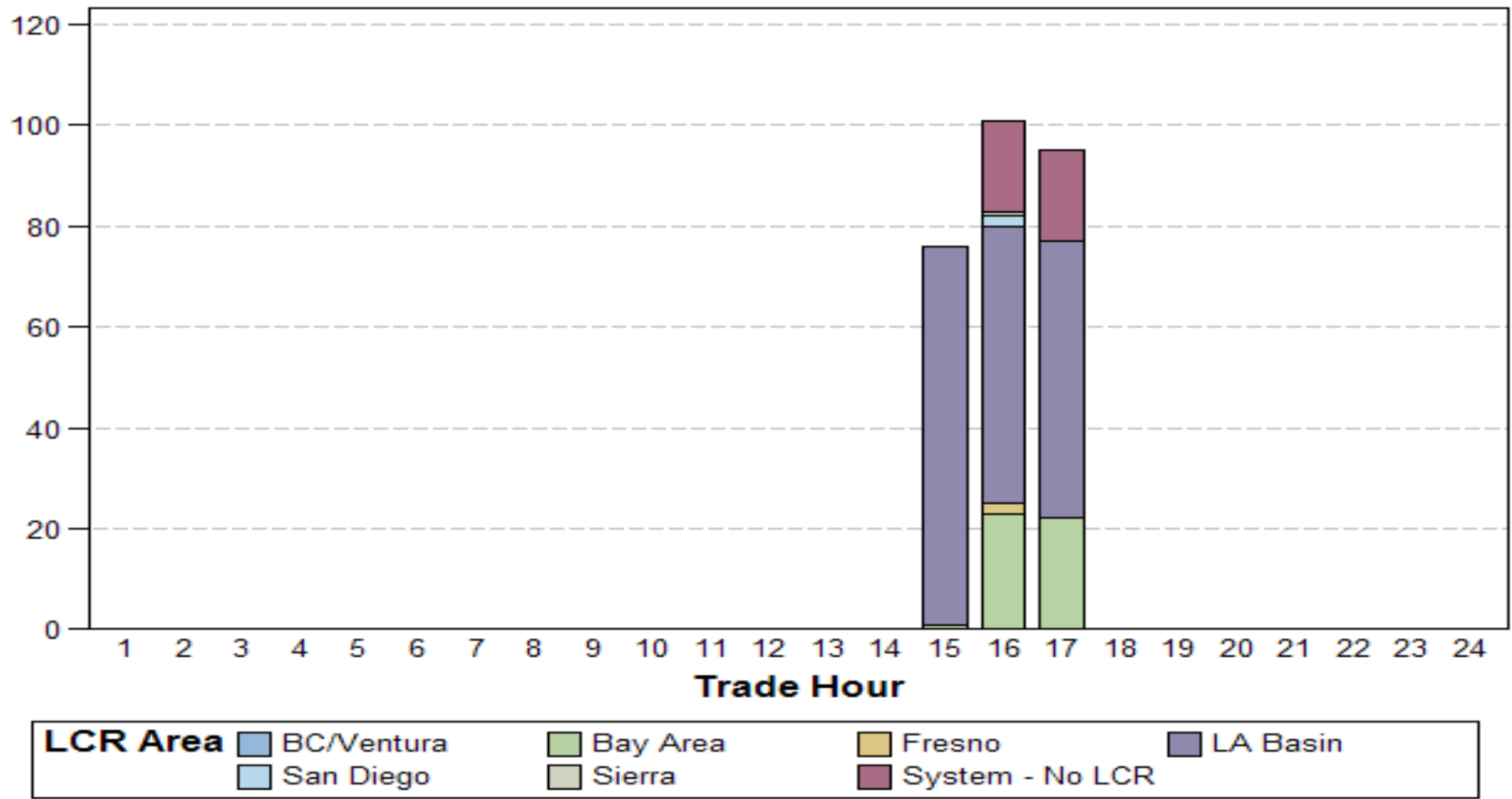
Non-RA RUC MW Procured
