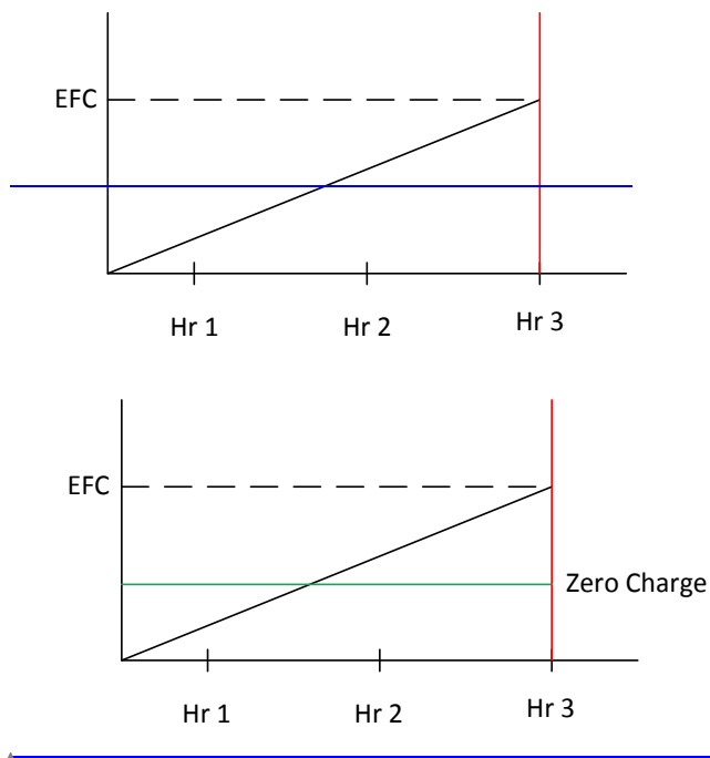
Figure 5: Example of EFC of storage resource over a 3 hour dispatch with constant ramp rate
