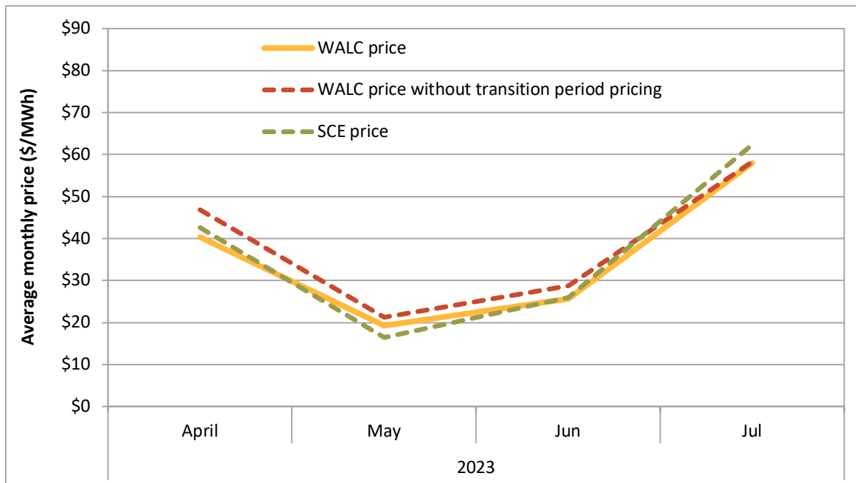
Figure 1.6 Average prices by month – Western Area Power Administration - Desert Southwest Region (WALC) (5-minute market)
