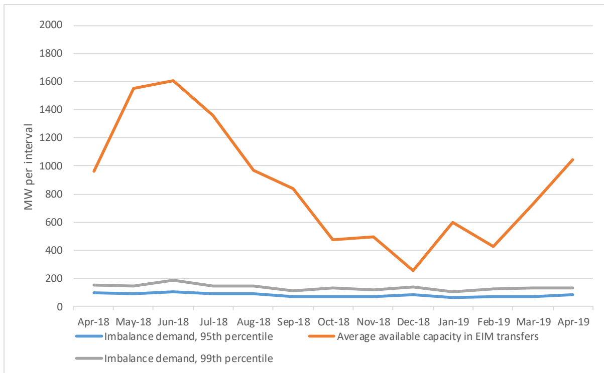
Figure 6: IPCO imbalance demand and competitive supply (5-minute market)
