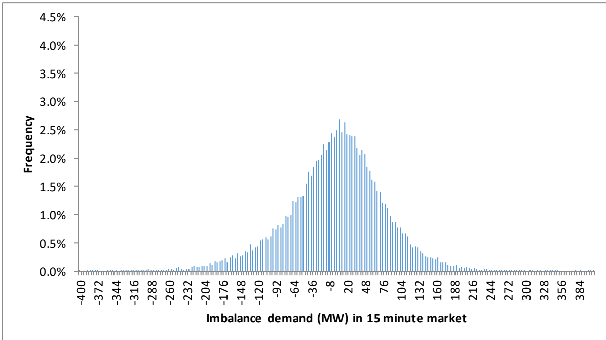
Figure 2. Imbalance energy demand compared to total load for the IPCO BAA (15-minute market, April 4, 2018 to April 3, 2019)
